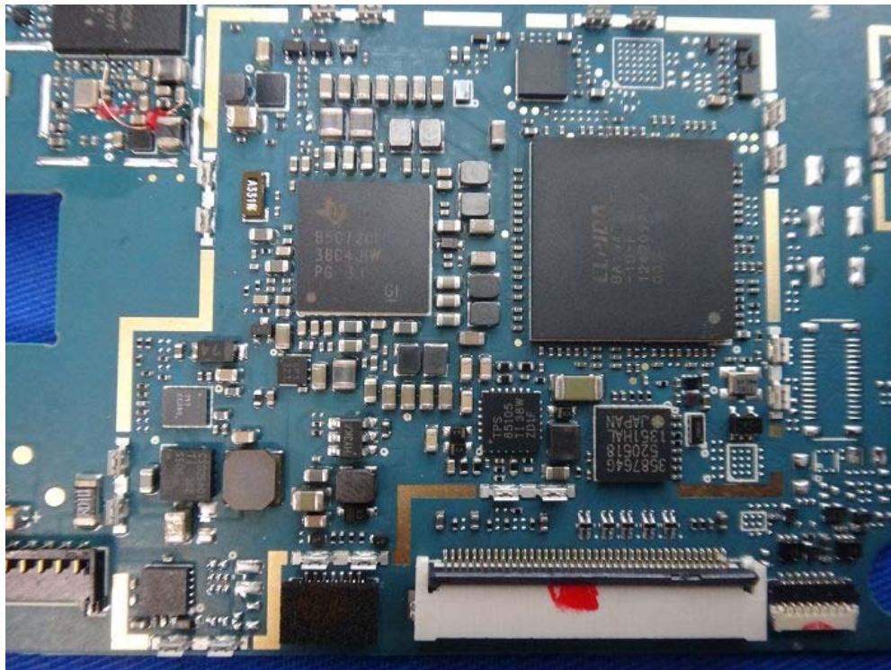
(7) EUT Photo
