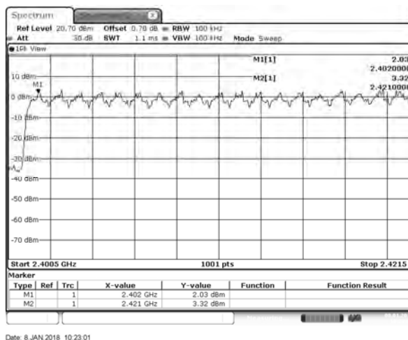
2402-2421MHz
