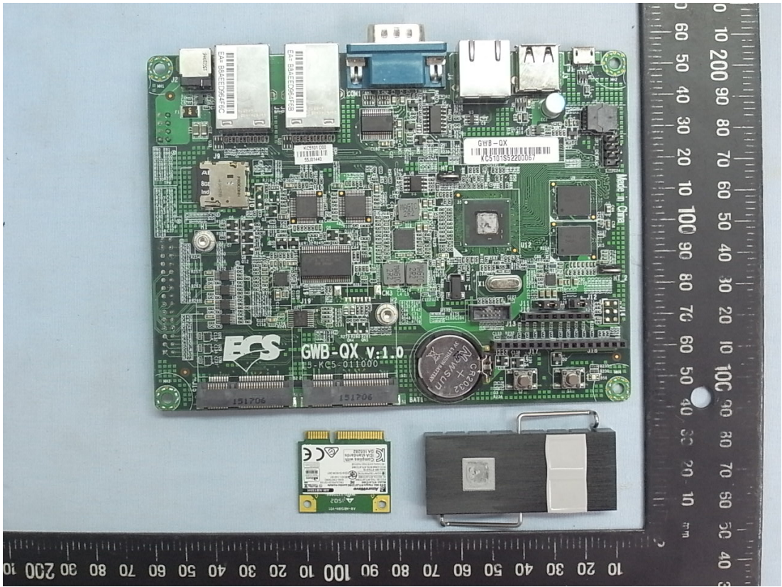
Figure 6 Internal View
