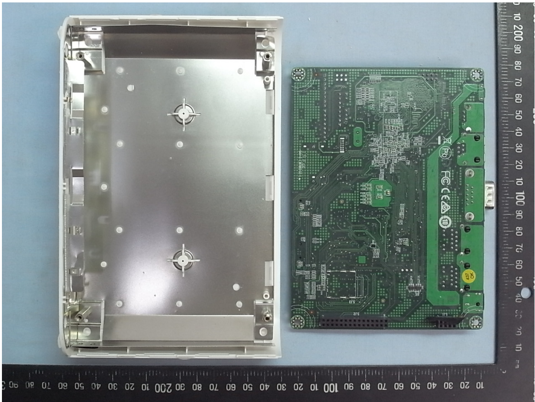
Figure 5 Internal View
