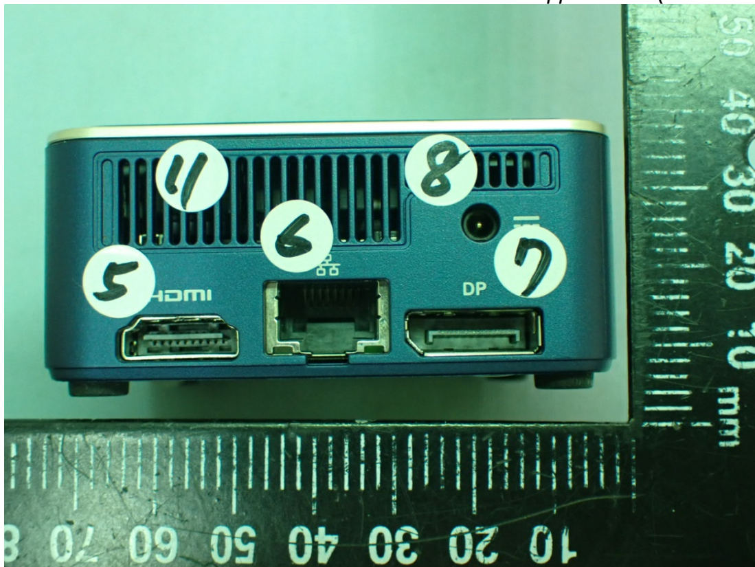
Figure 14 General Appearance (Side View)
