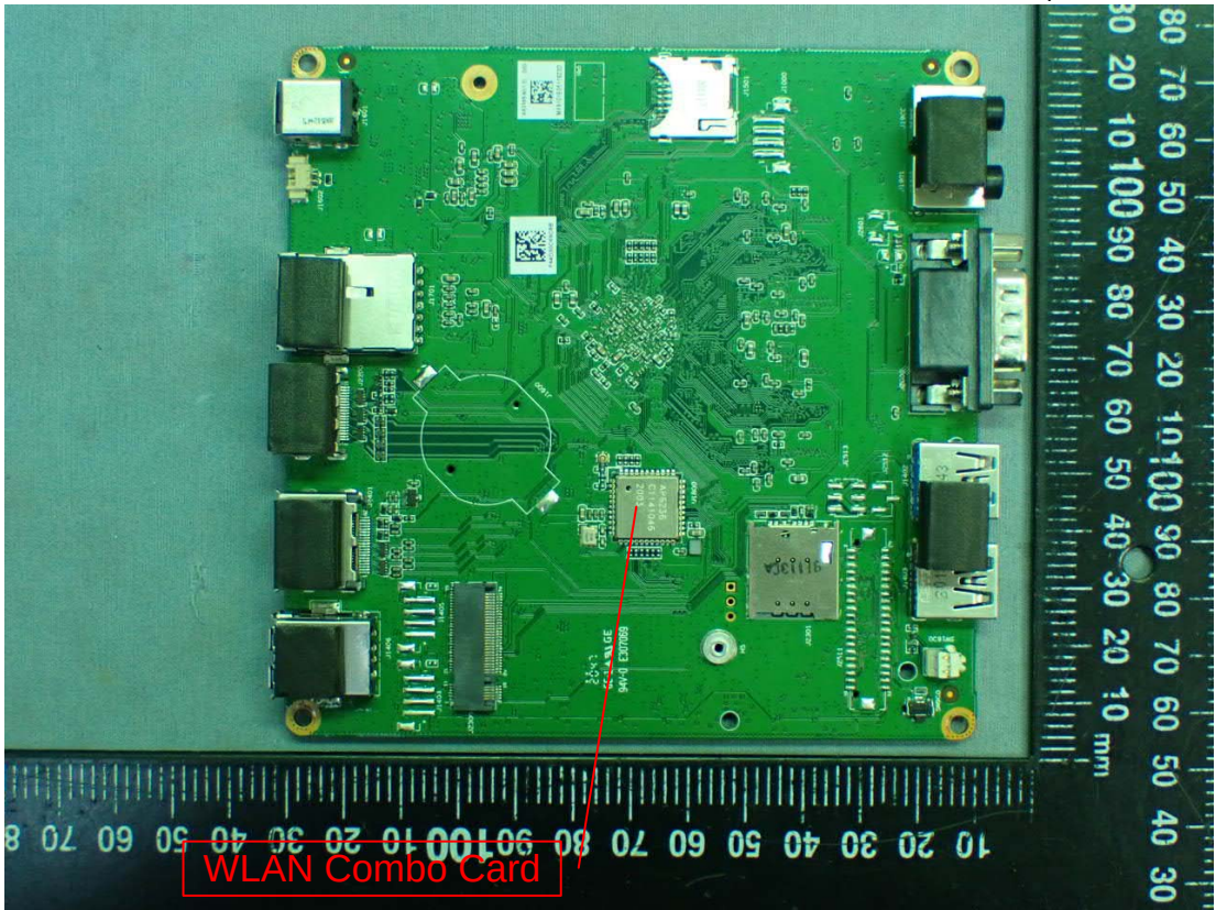
Figure 12 Mother Board, Back View
