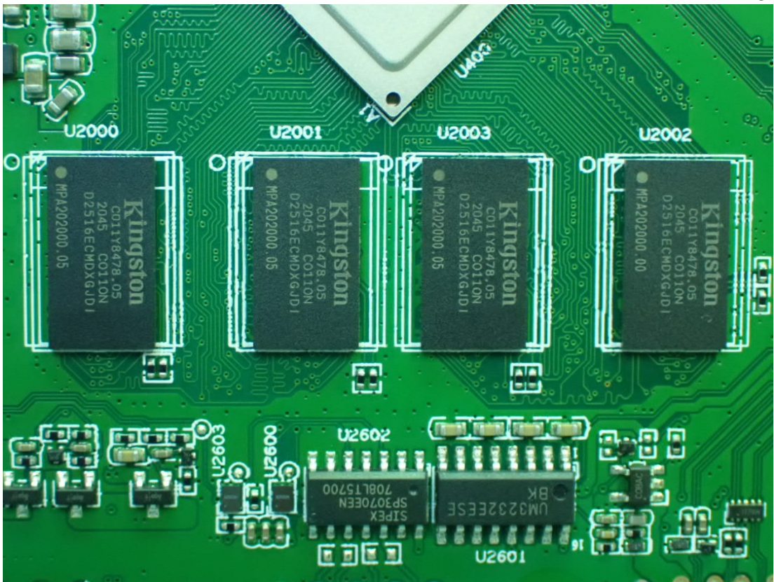
Figure 15 DRAM View
