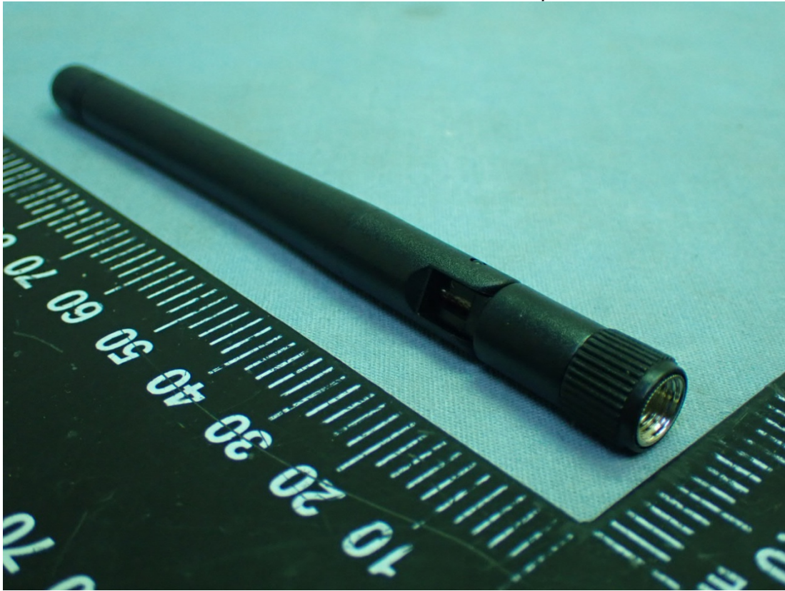
Figure 19 Dipole Antenna, Front View
