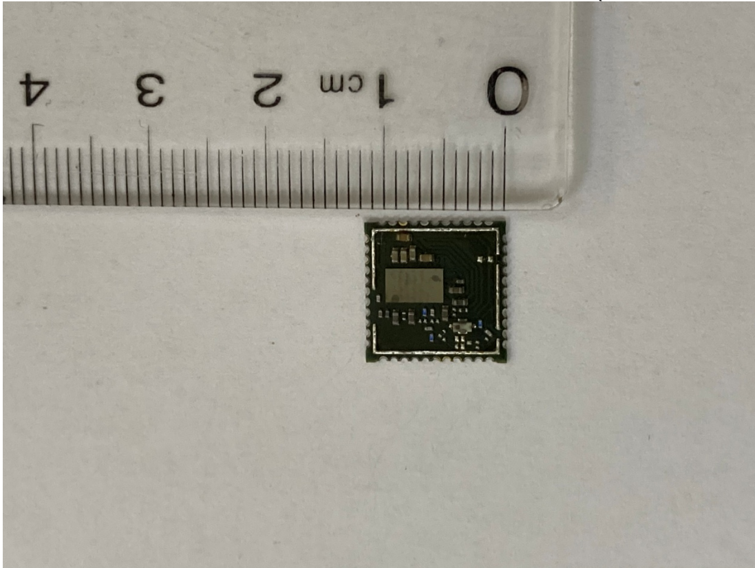
Figure 17 WLAN Combo Card , Front View (Removed Cover)
