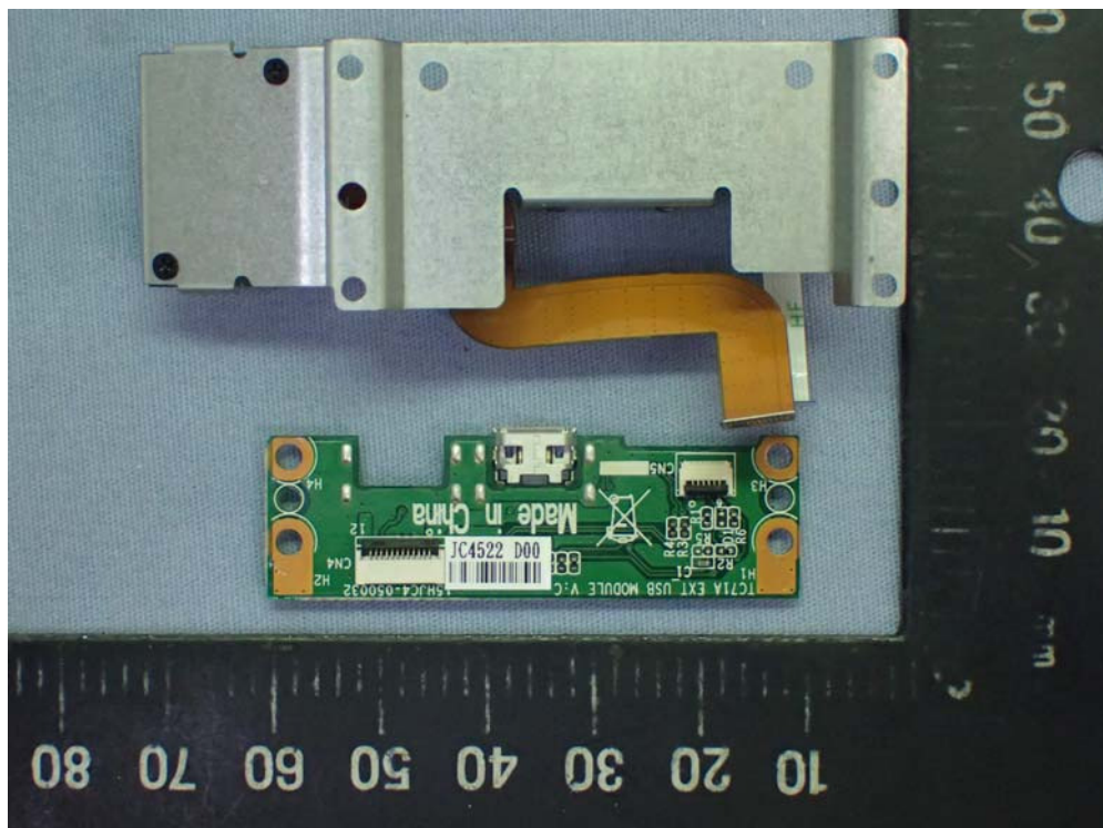
Figure 52 Barcode Scanner mPAD, Internal View (USB Board, Front View)
