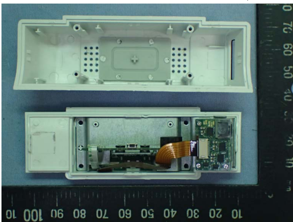
Figure 50 Barcode Scanner mPAD, Internal View (Removed Cover)
