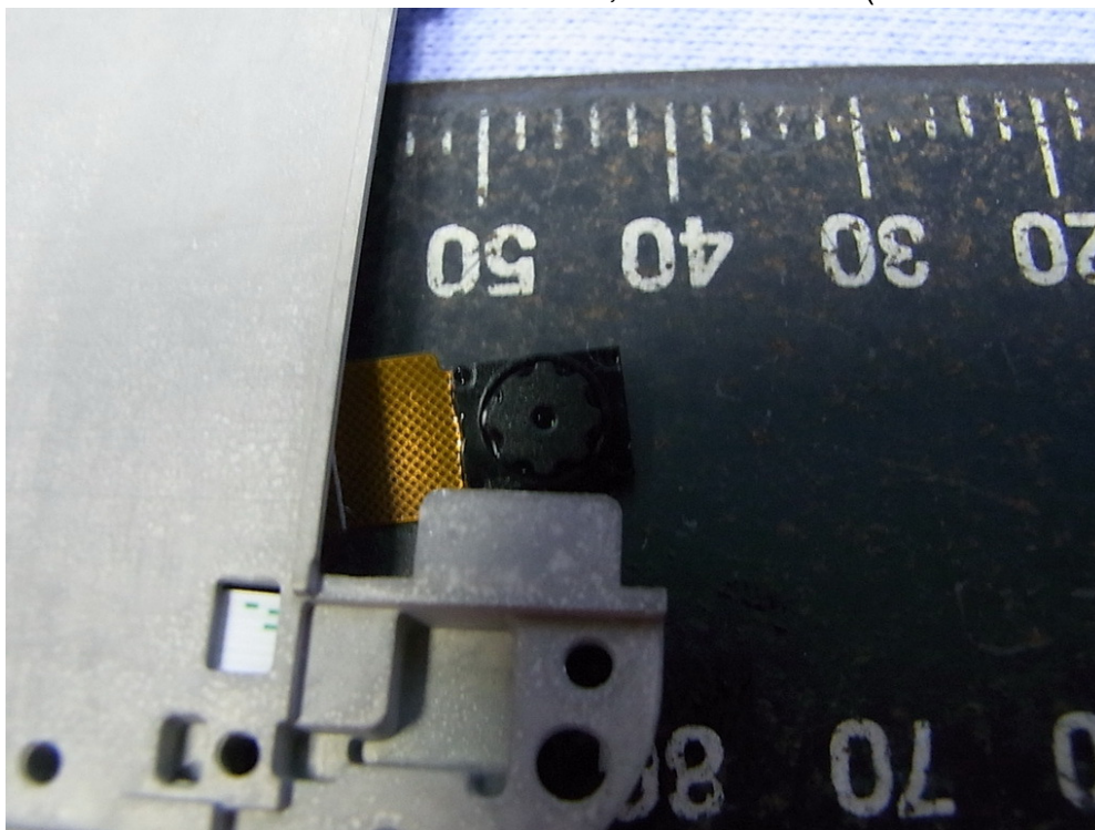
Figure 49 7" Multi Function Pad, Internal View (Front Camera View)
