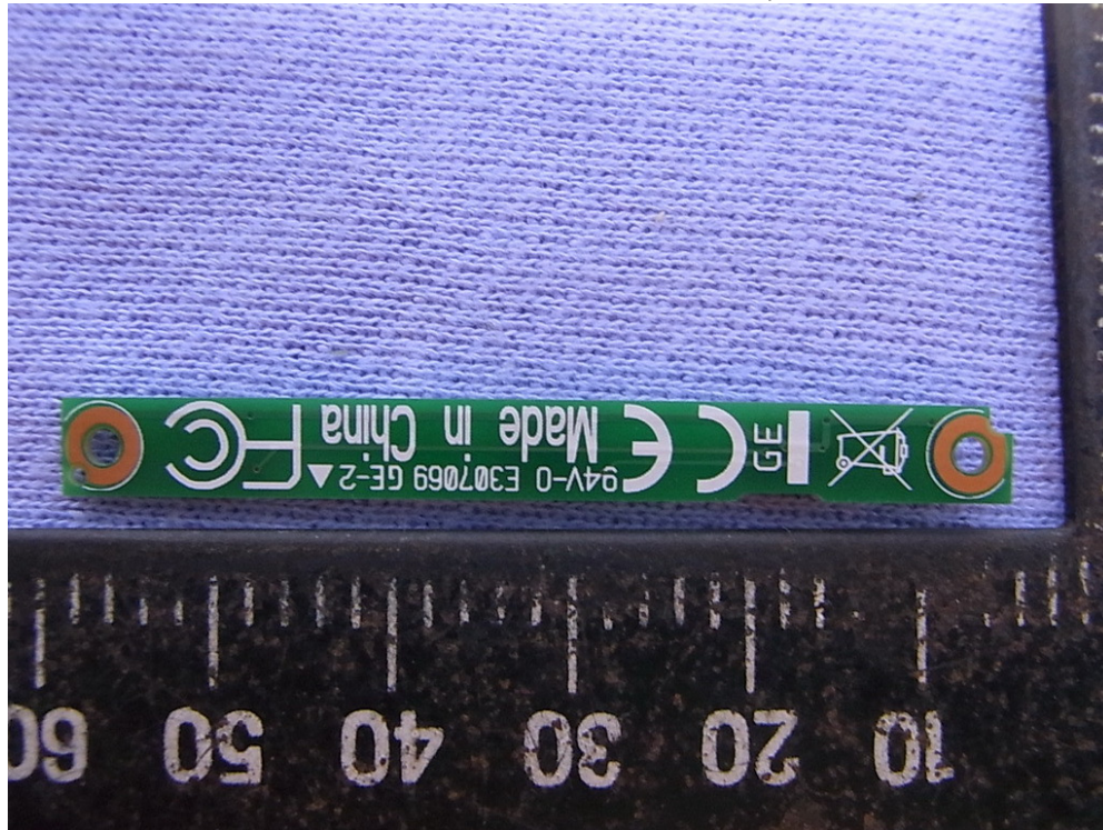
Figure 43 7" Multi Function Pad, Internal View (Control Board, Back View)
