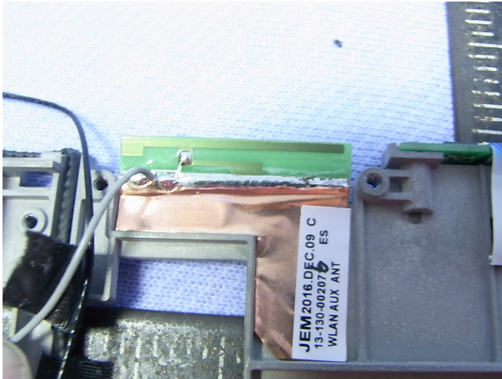
Figure 41 7" Multi Function Pad, Internal View (WLAN Aux Antenna)
