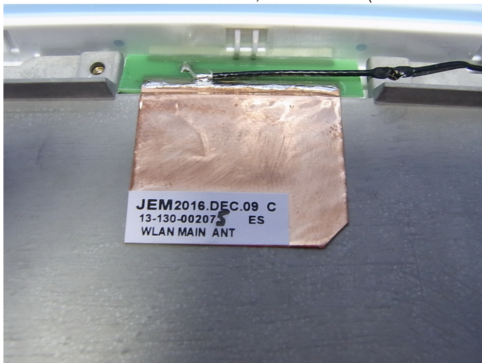
Figure 40 7" Multi Function Pad, Internal View (WLAN Main Antenna)
