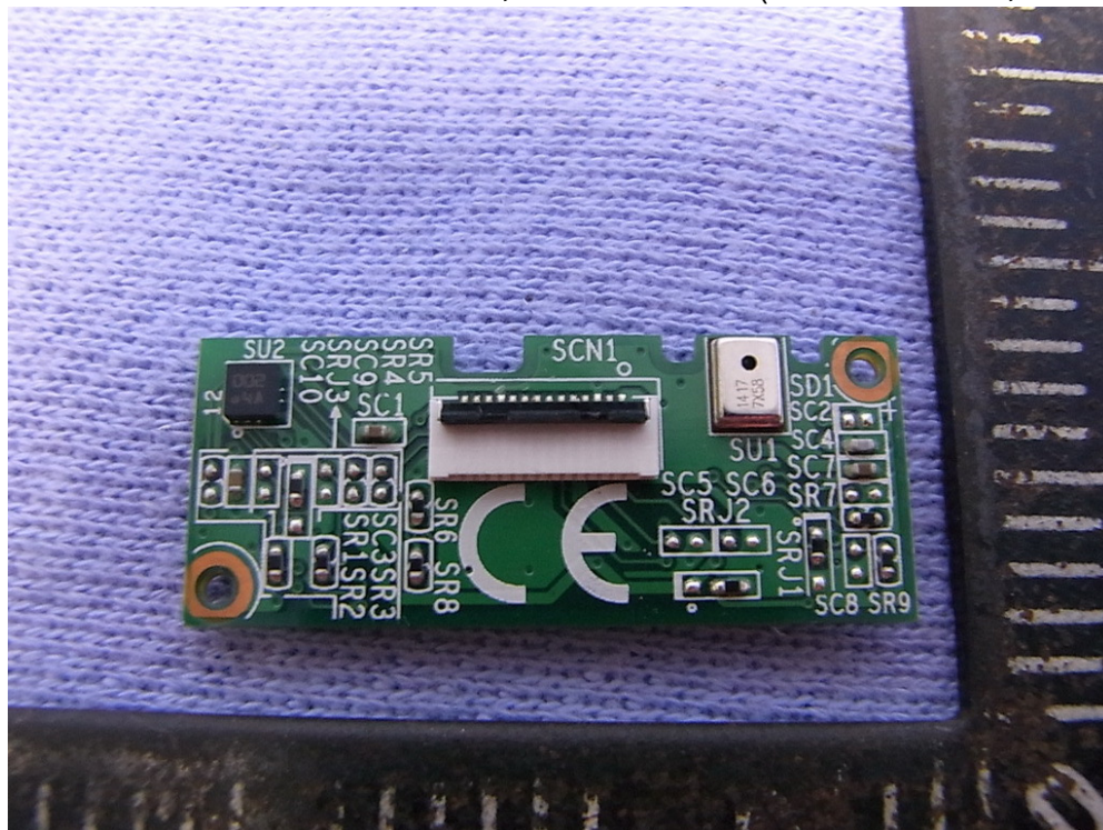
Figure 44 7" Multi Function Pad, Internal View (Control Board, Front View)
