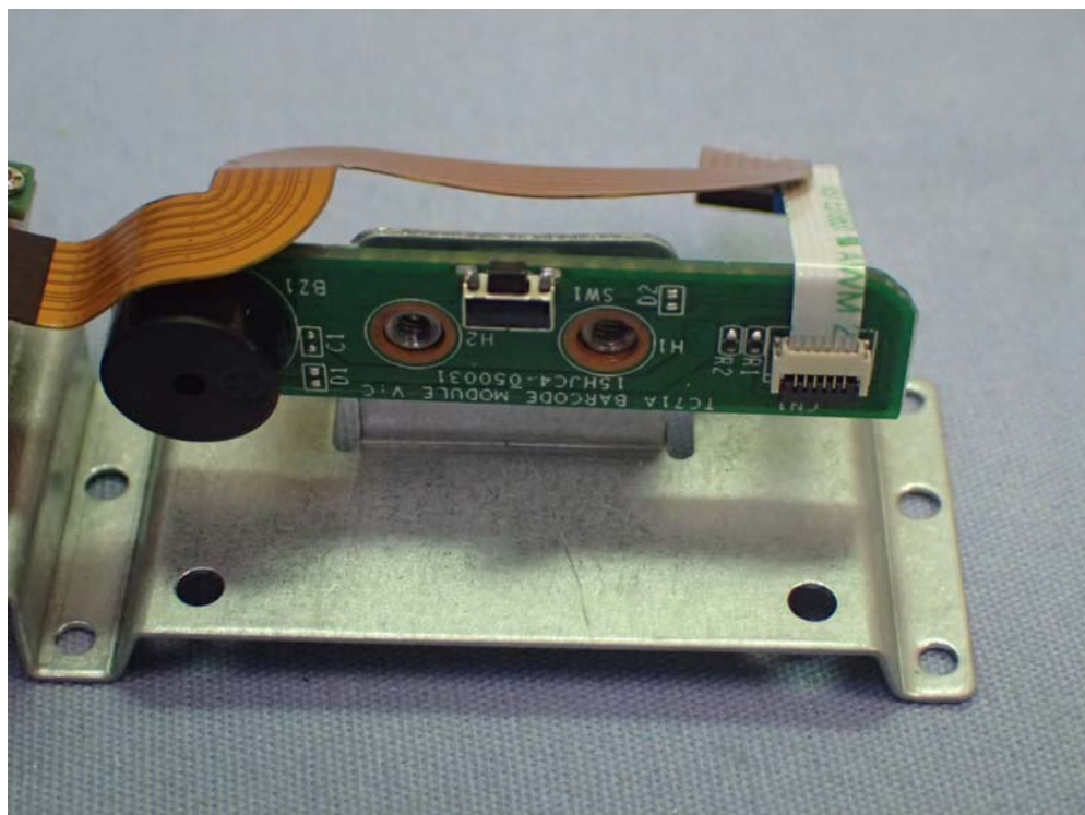
Figure 54 Barcode Scanner mPAD, Internal View
