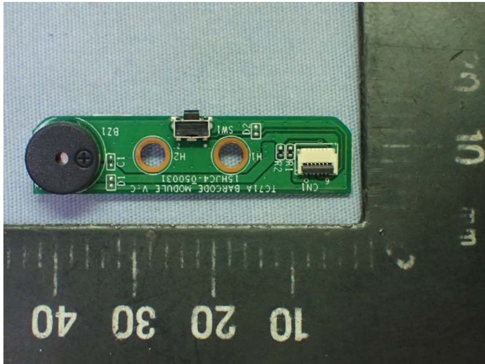
Figure 55 Barcode Scanner mPAD, Internal View (Switch Board, Front View)
