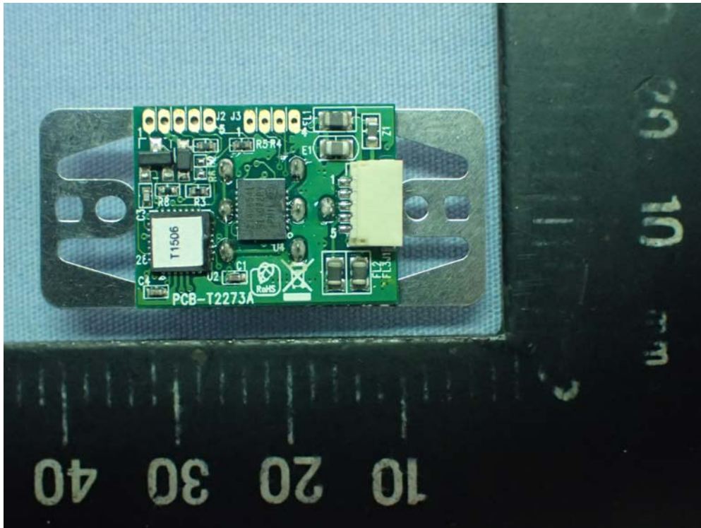
Figure 69 MSR Module, Internal View
