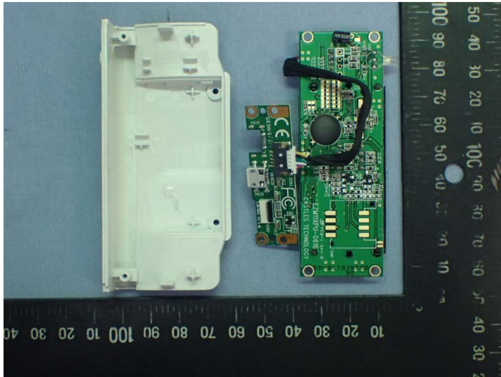
Figure 59 SCR mPAD, Internal View (Removed Cover)
