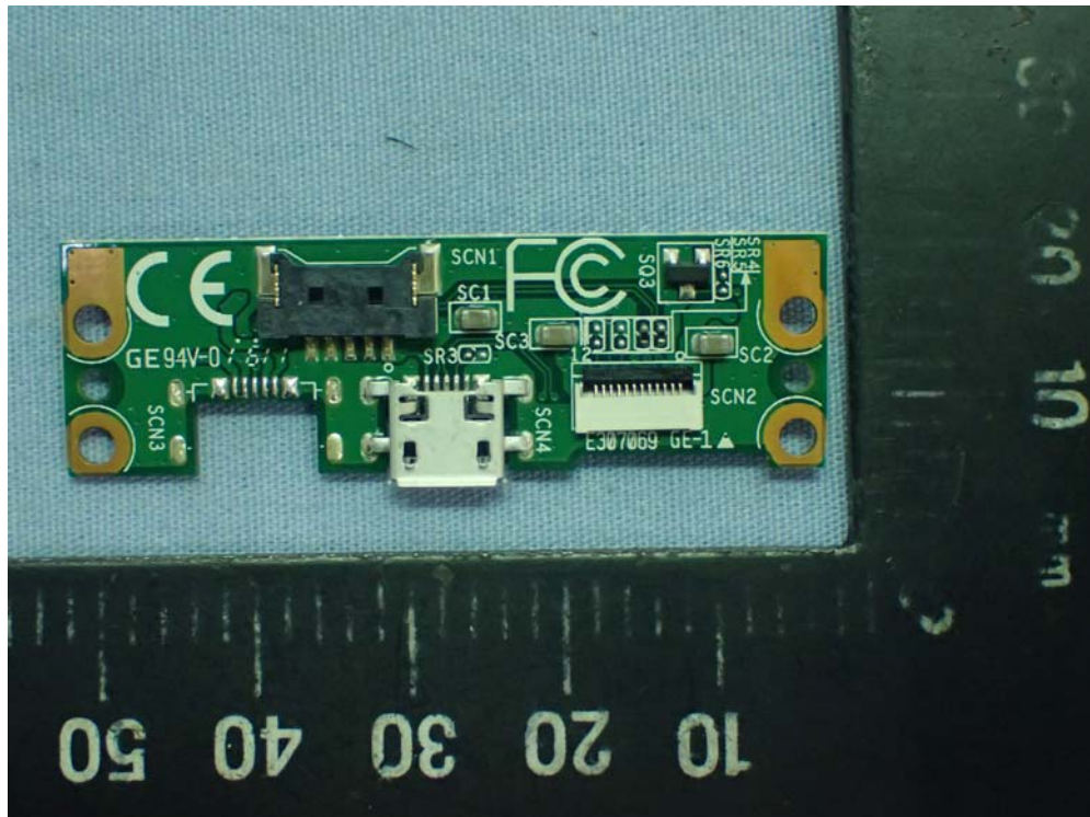
Figure 60 SCR mPAD, Internal View (USB Board, Front View)
