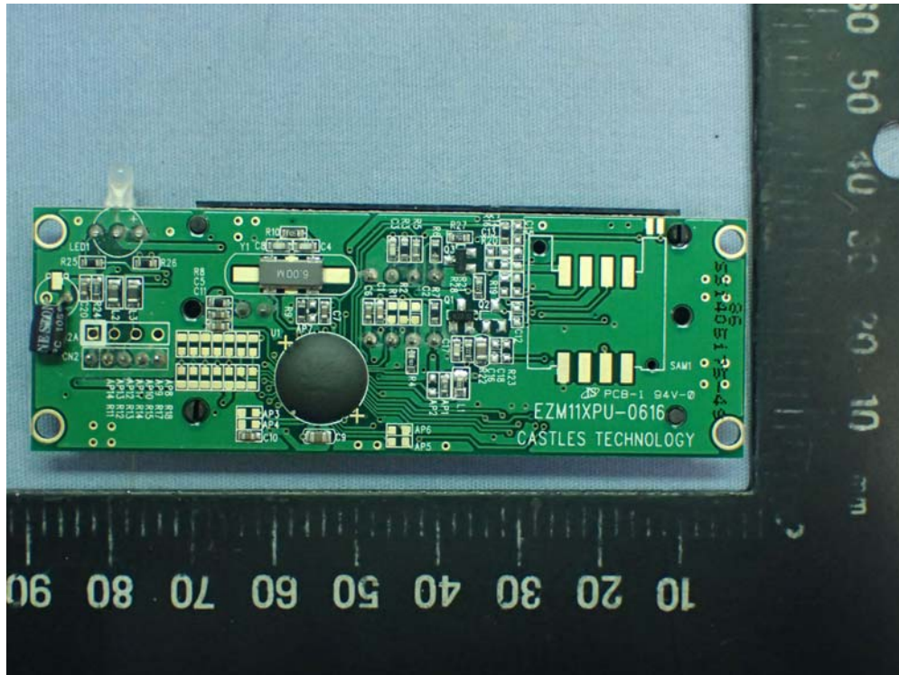
Figure 63 SCR mPAD, Internal View (Control Board, Back View)
