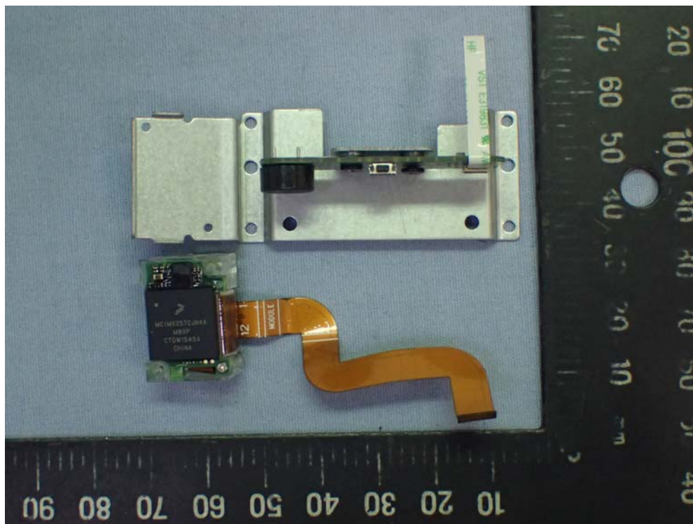
Figure 57 Barcode Scanner mPAD, Internal View
