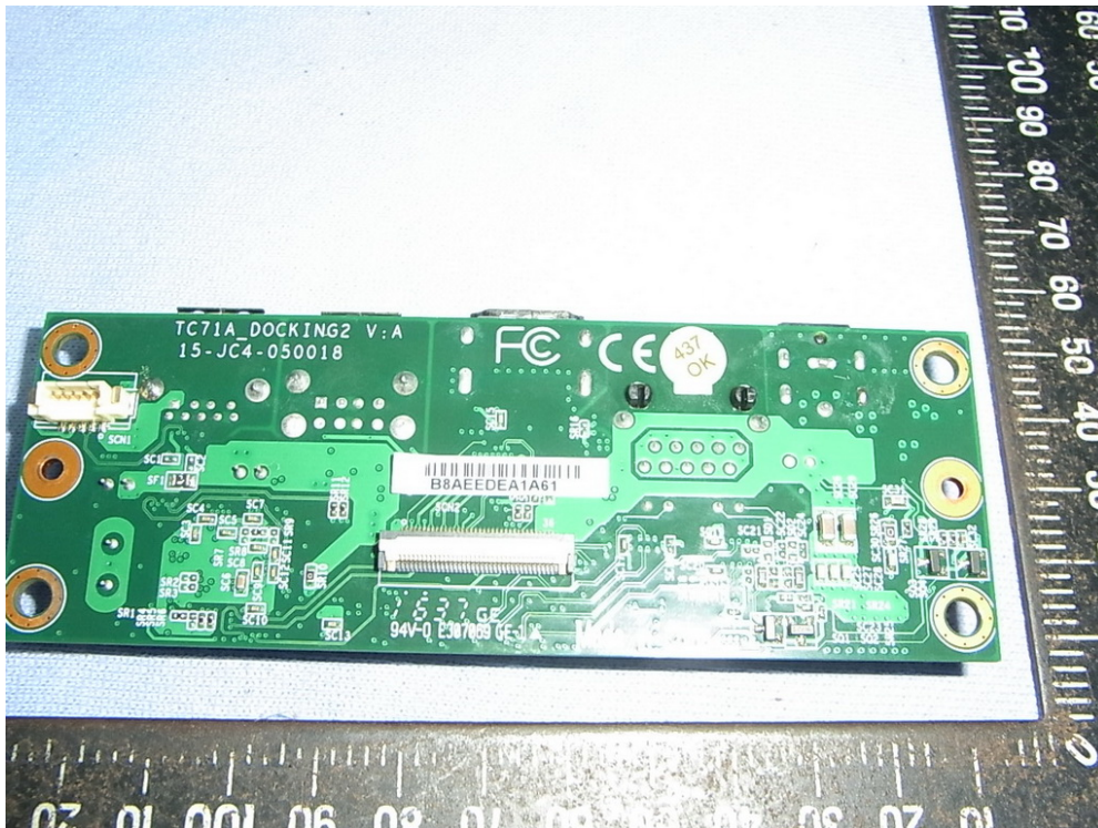
Figure 80 7" Pad Docking, Internal View (Control Board, Back View)
