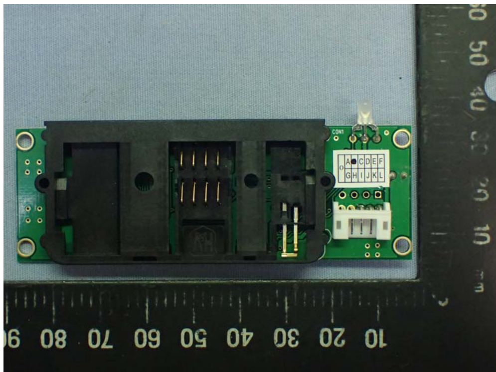
Figure 62 SCR mPAD, Internal View (Control Board, Front View)
