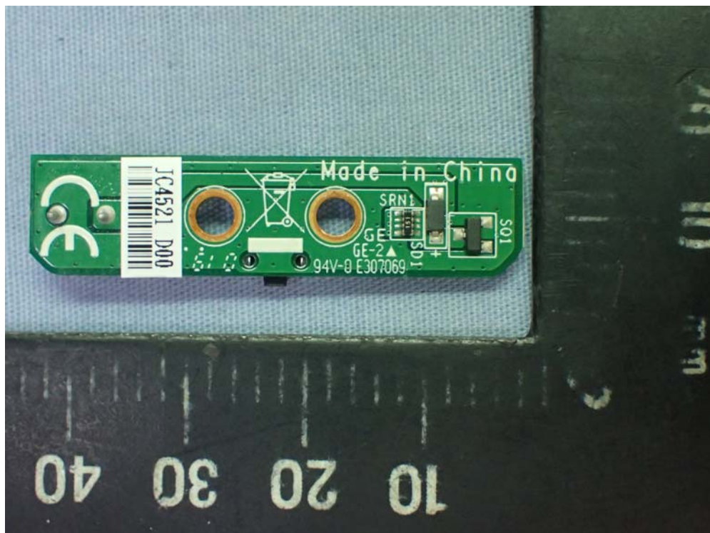
Figure 56 Barcode Scanner mPAD, Internal View (Switch Board, Back View)
