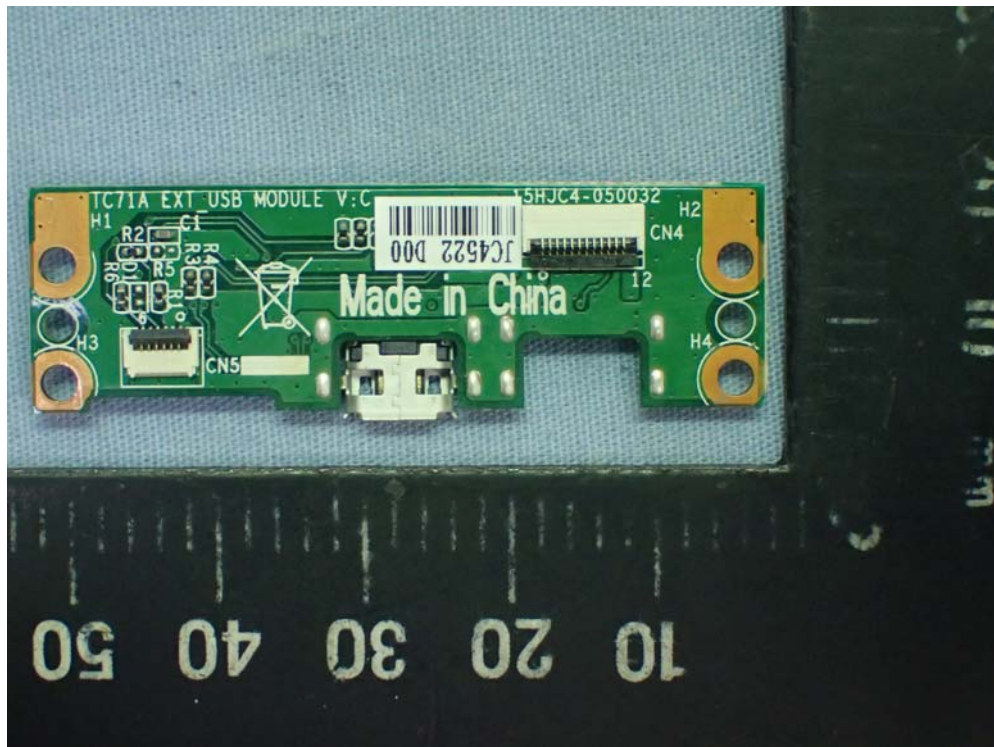
Figure 53 Barcode Scanner mPAD, Internal View (USB Board, Back View)
