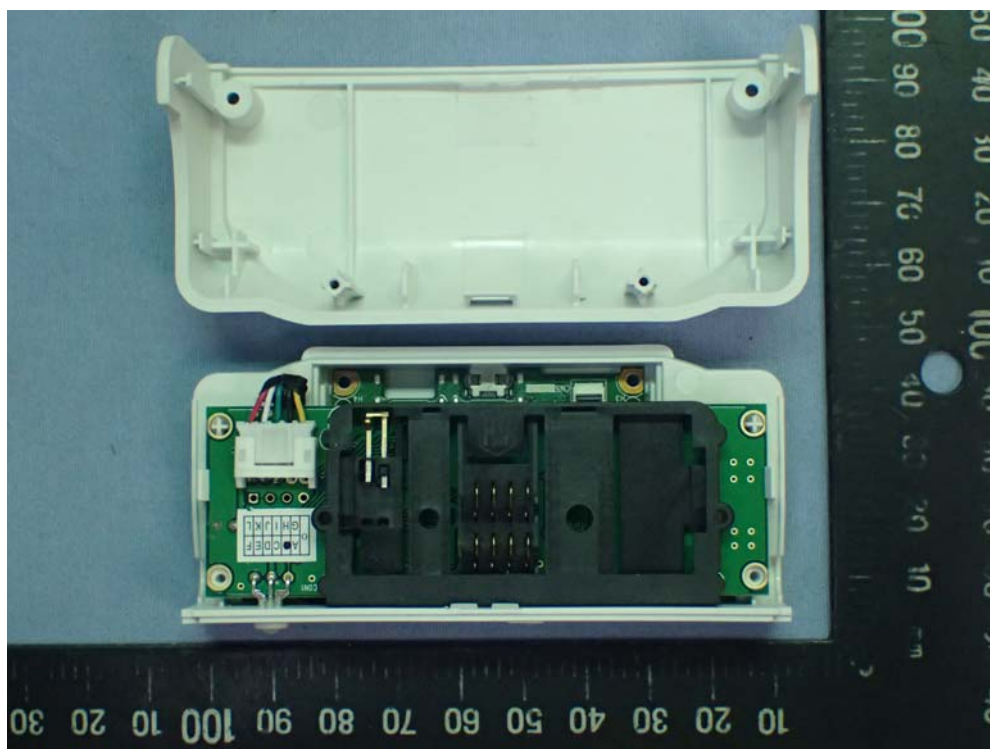
Figure 58 SCR mPAD, Internal View (Removed Cover)
