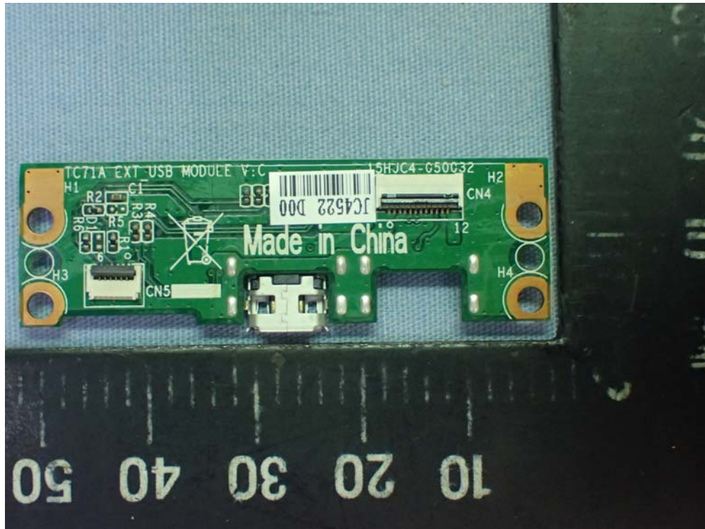
Figure 67 MSR Module, Internal View (USB Board, Back View)
