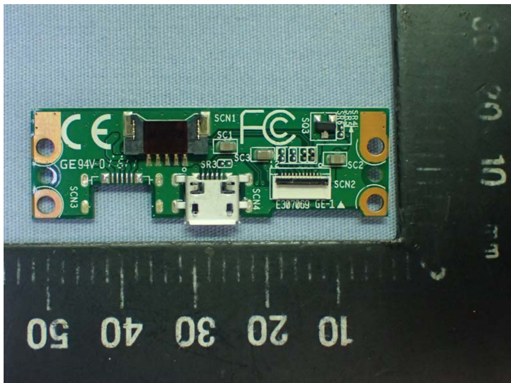
Figure 66 MSR Module, Internal View (USB Board, Front View)
