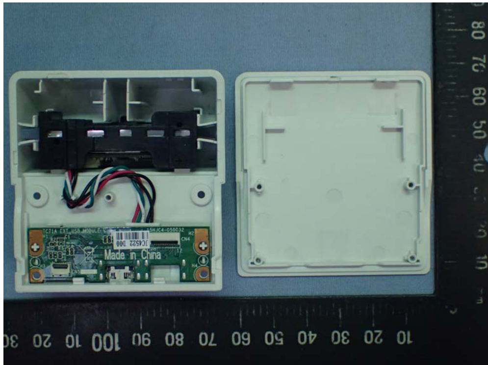
Figure 64 MSR Module, Internal View (Removed Cover)
