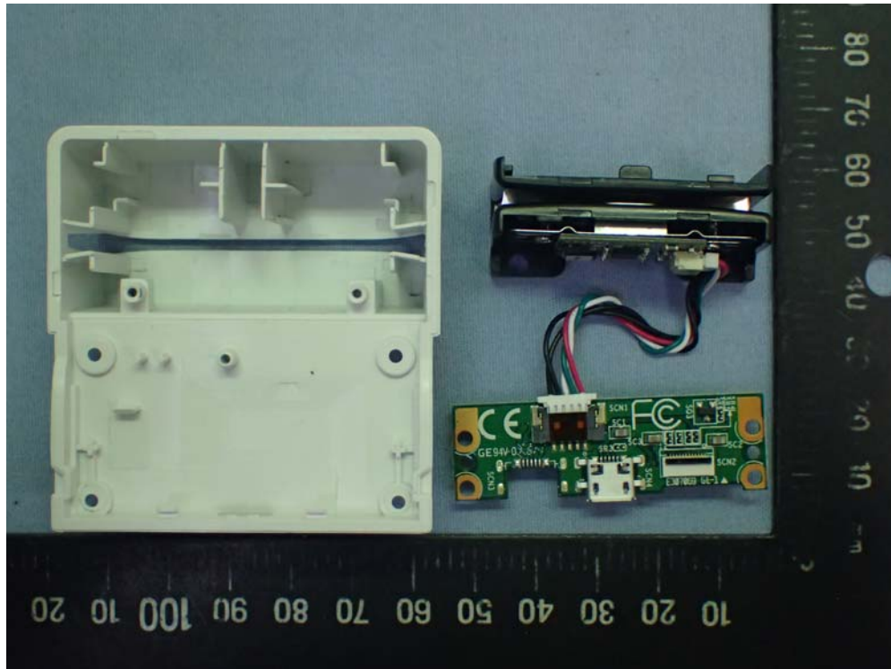
Figure 65 MSR Module, Internal View
