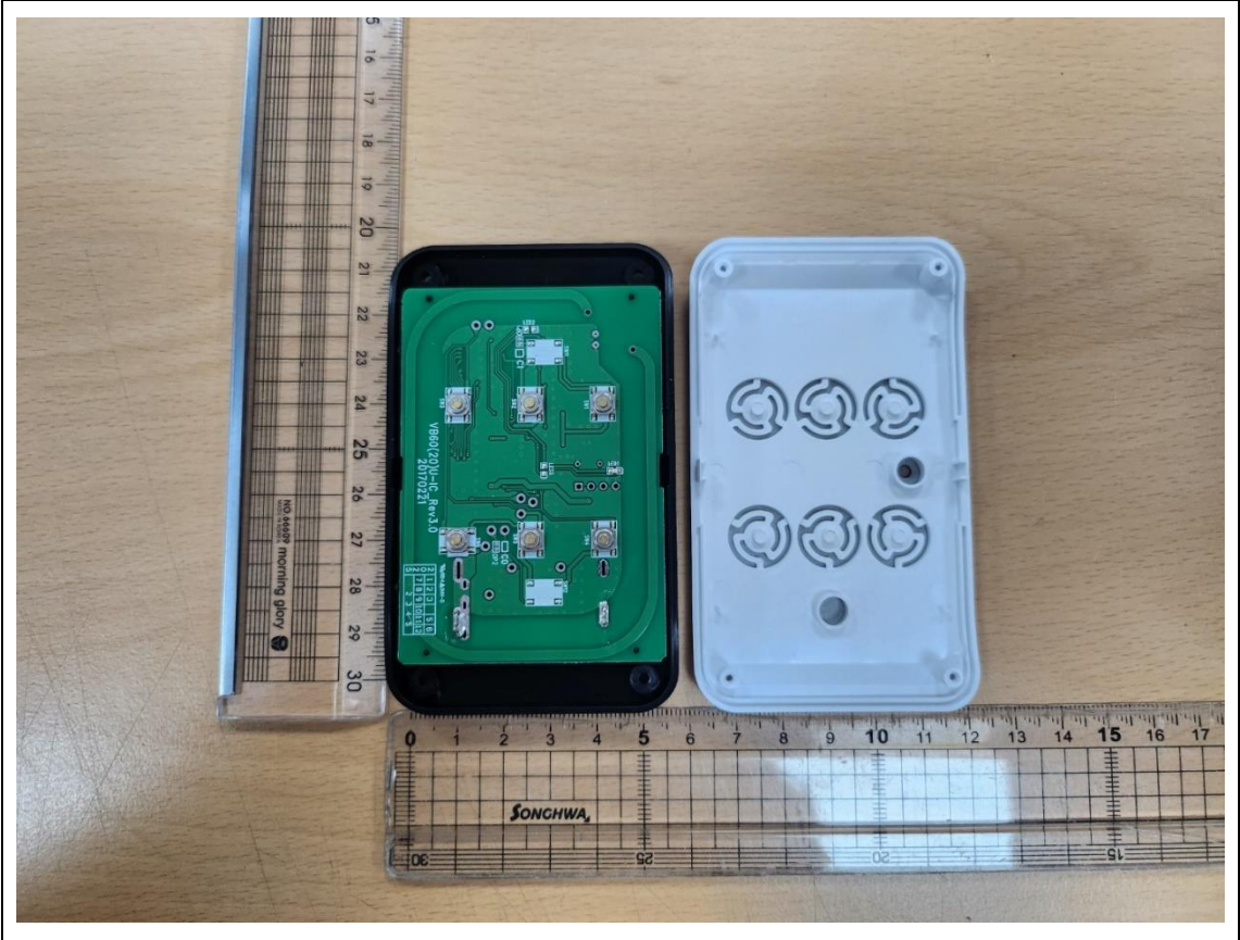
Internal side
