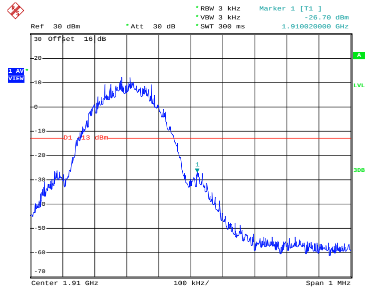
Higher Band Edge Plot on Channel 810 (1909.8 MHz)
