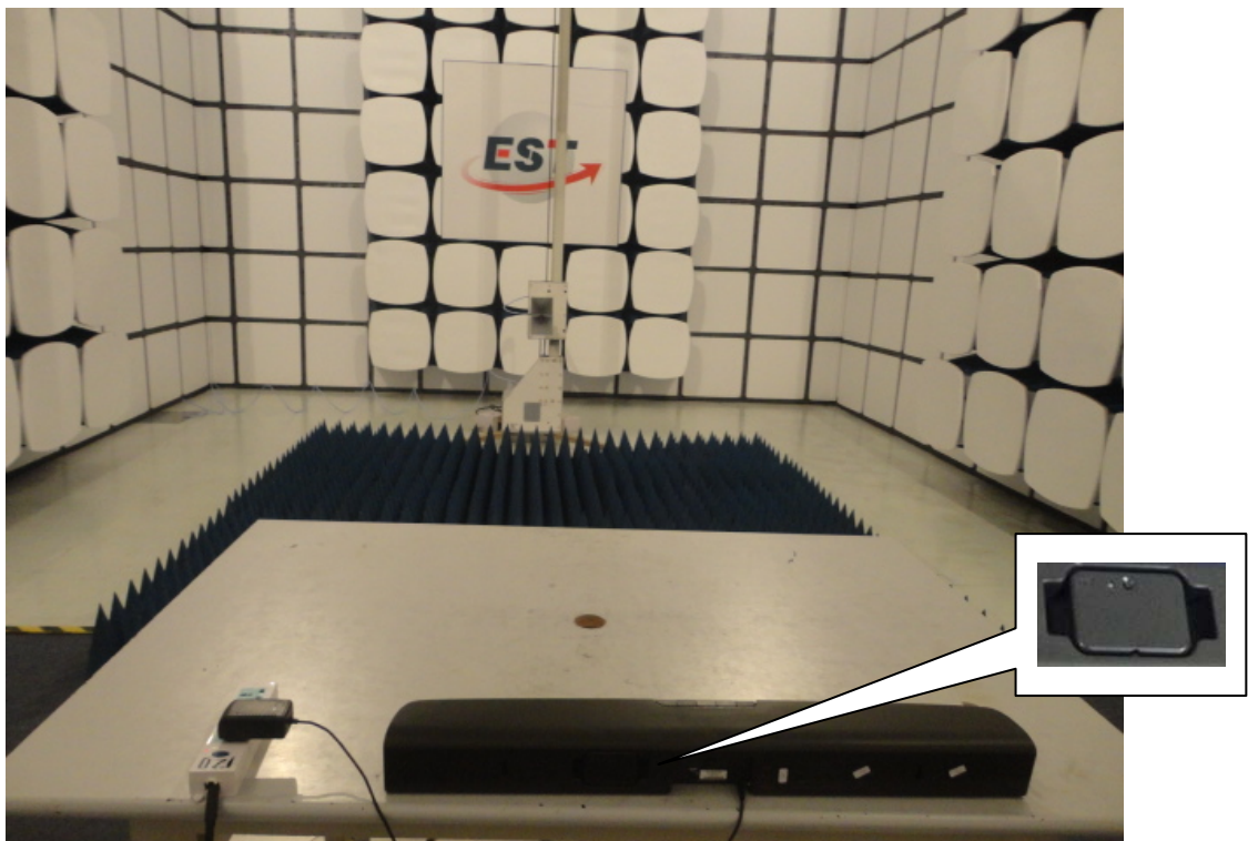
Radiated Test (1000-25000 MHz)
