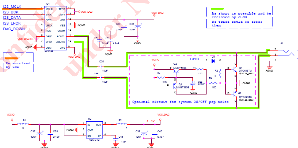
Fig 9.2 DAC reference design circuit
