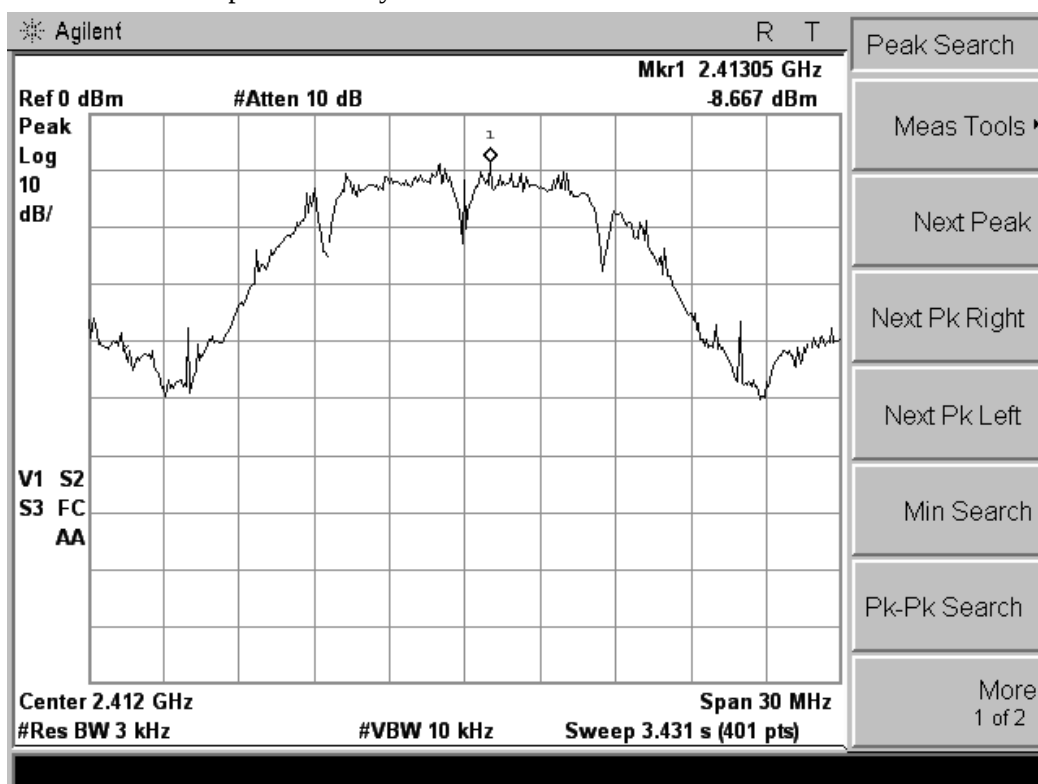
802.11b power density
