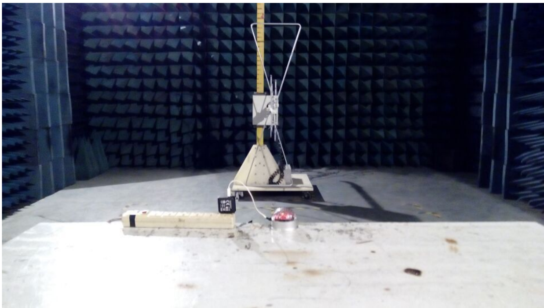
Radiated Emission (Below 1GHz)
