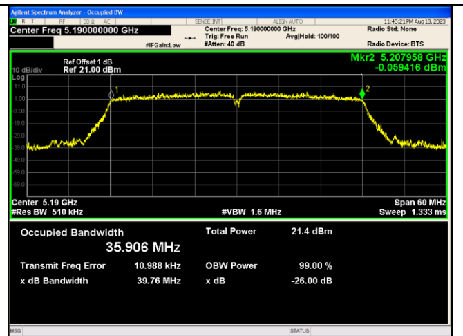
IEEE 802.11ac Channel 38 40MHz Antenna 3
