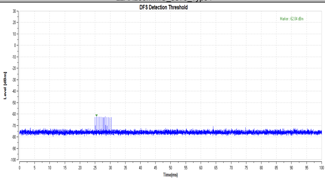
11AX160MIMO_5570_Type5
