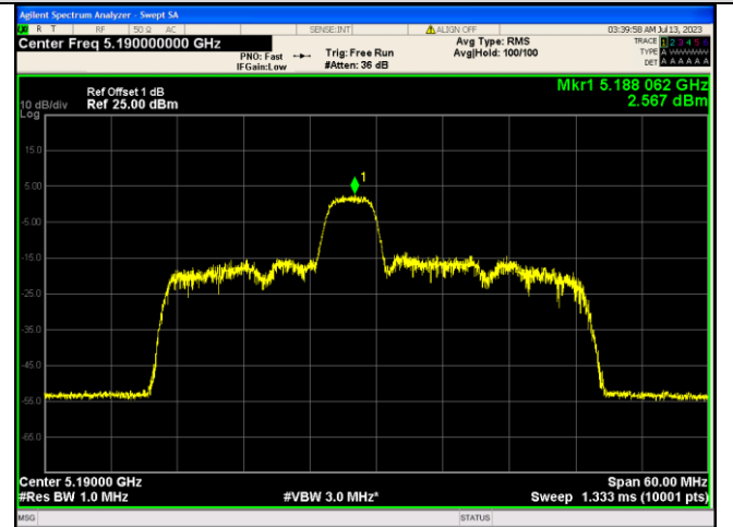
IEEE 802.11ax_Channel 38_40MHz_Antenna 1_RU&amp;Index 52RU40
