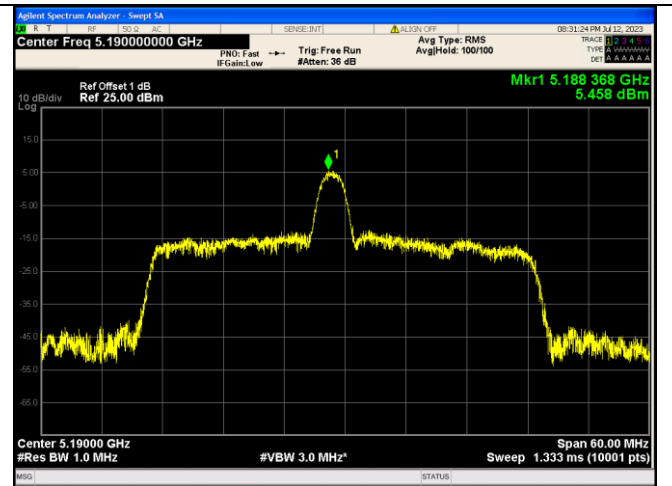
IEEE 802.11ax_Channel 38_40MHz_Antenna 1_RU&amp;Index 26RU8
