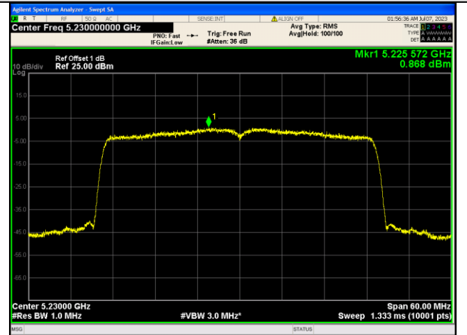
IEEE 802.11ax_Channel 46_40MHz_Antenna 1_RU&amp;Index 484RU65
