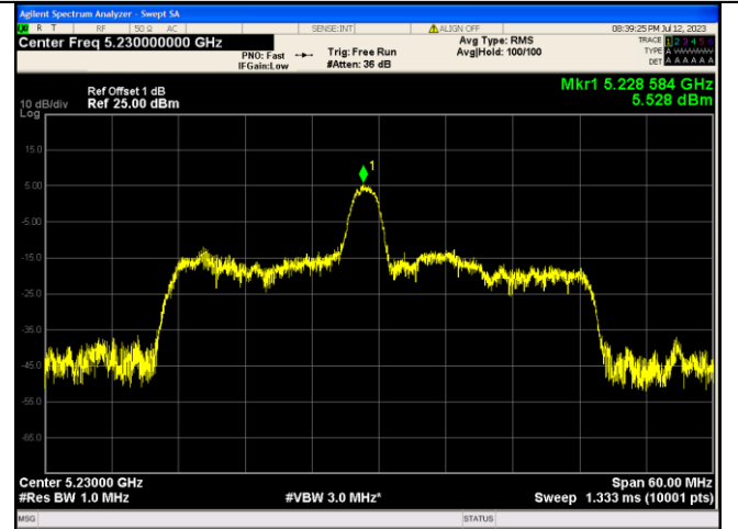
IEEE 802.11ax_Channel 46_40MHz_Antenna 1_RU&amp;Index 26RU8
