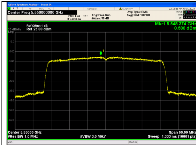
IEEE 802.11ax Channel 110_40MHz_Antenna 0 RU&Index 484RU65
