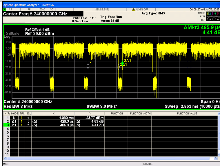
IEEE 802.11ax 20MHz Channel 48
