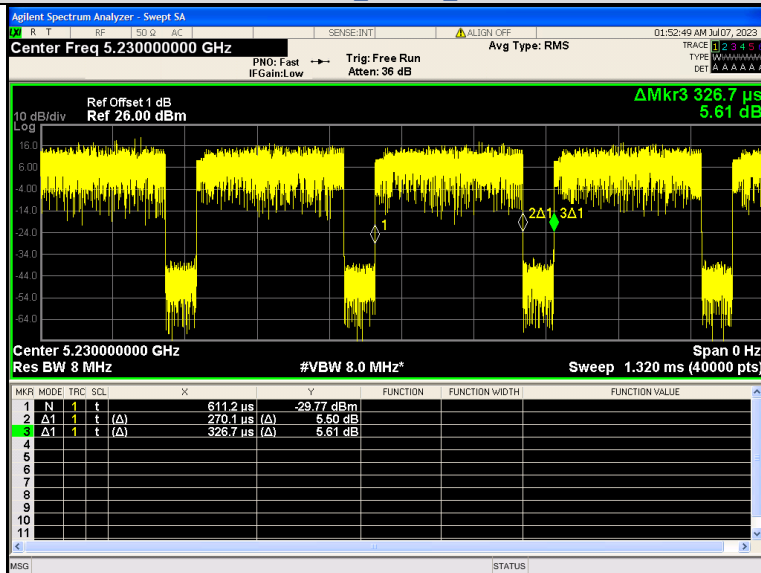
IEEE 802.11ax 40MHz Channel 46
