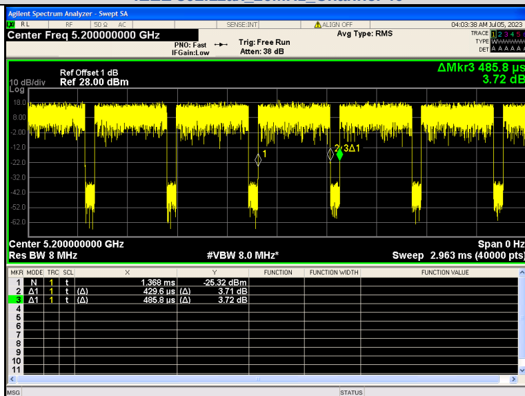
IEEE 802.11ax 20MHz Channel 40
