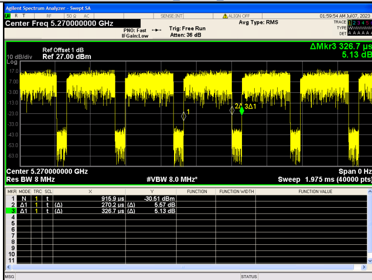
IEEE 802.11ax 40MHz Channel 54
