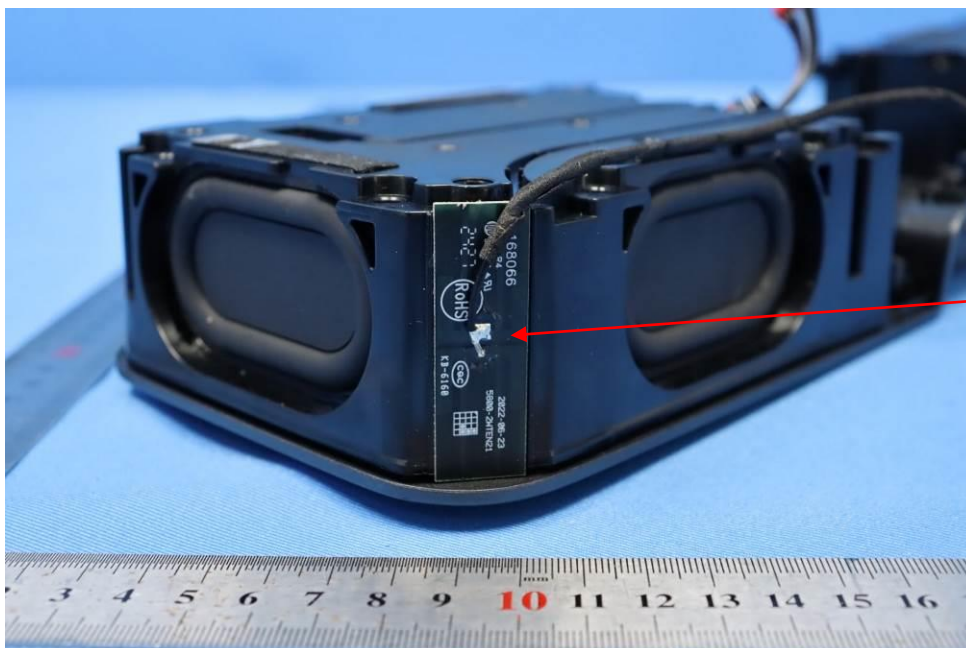
WIFI antenna1
