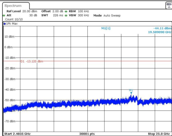
BLE_1M_Ant1_2402_2483.5~25000
