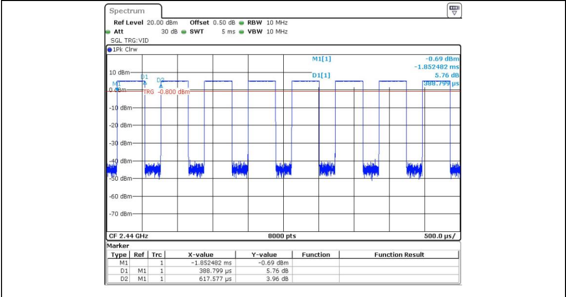
BLE_1M_Ant1_2440
