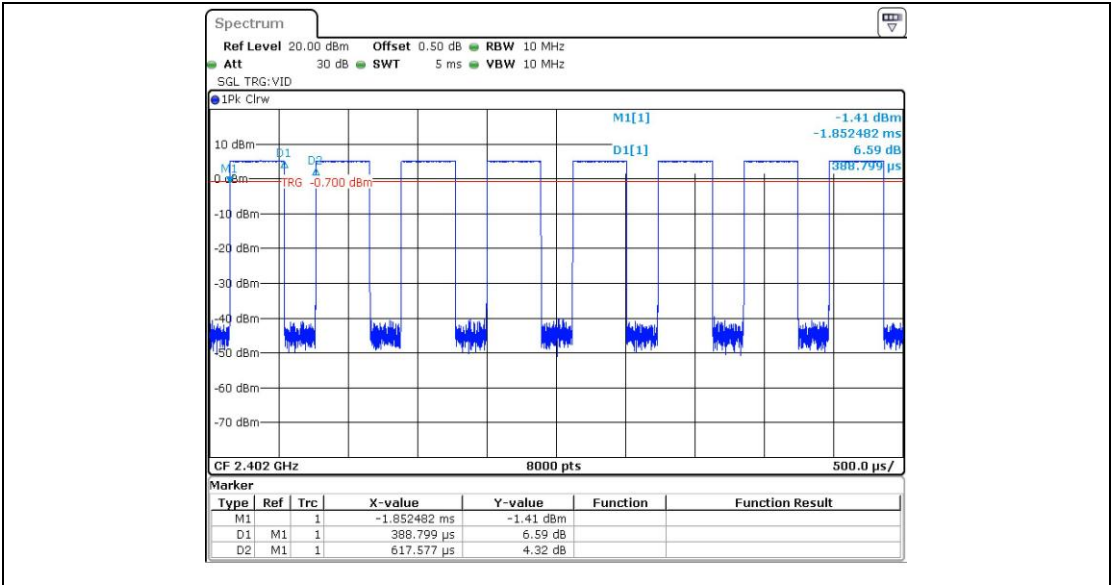
BLE_1M_Ant1_2402
