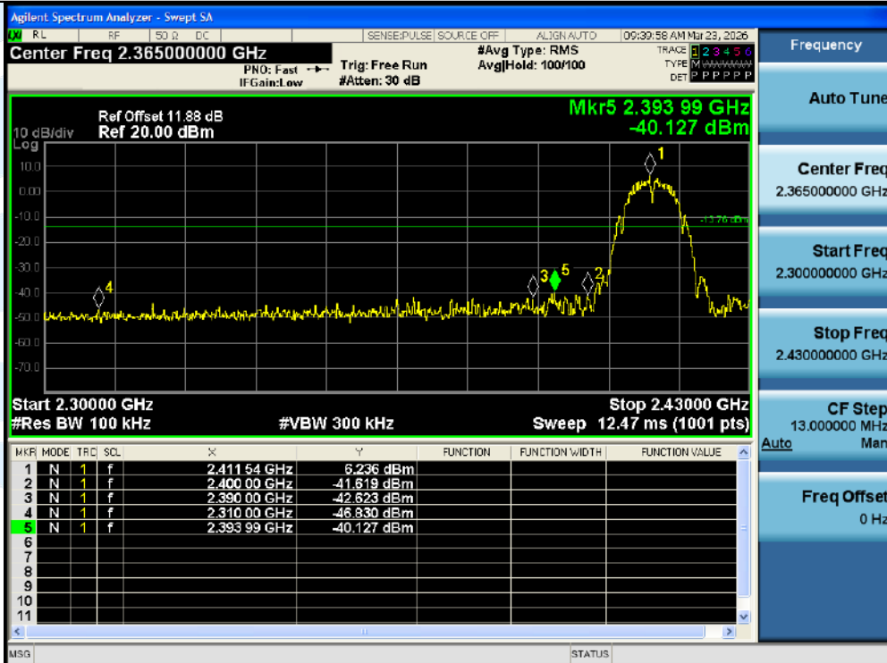
11B-Ant2-2412-PASS
