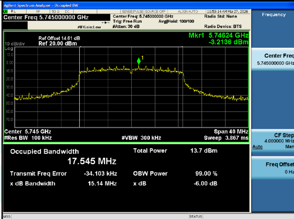
11AC20MIMO-Ant1-5745-PASS
