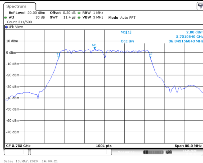
11AC40SISO_Ant2_5755
