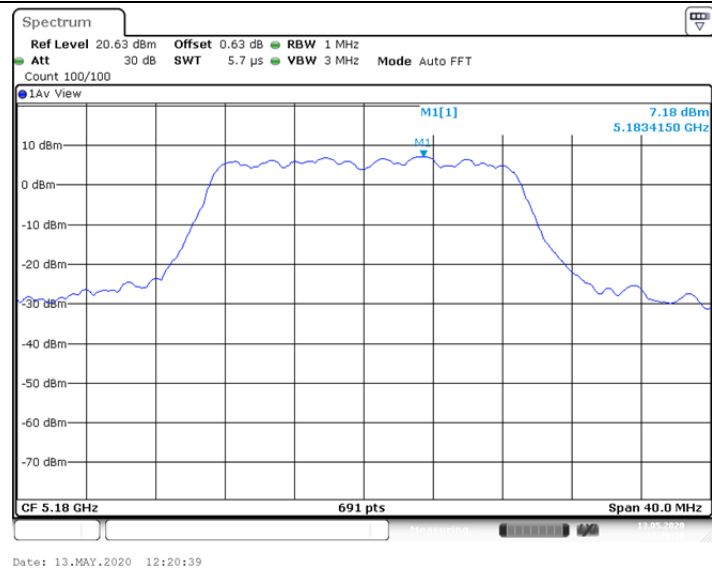
11N20SISO_Ant2_5180
