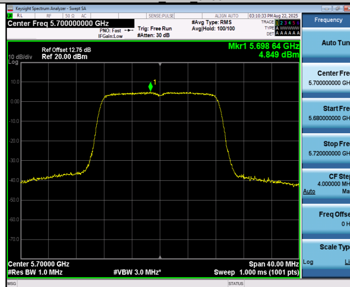
11A Ant2 5700
