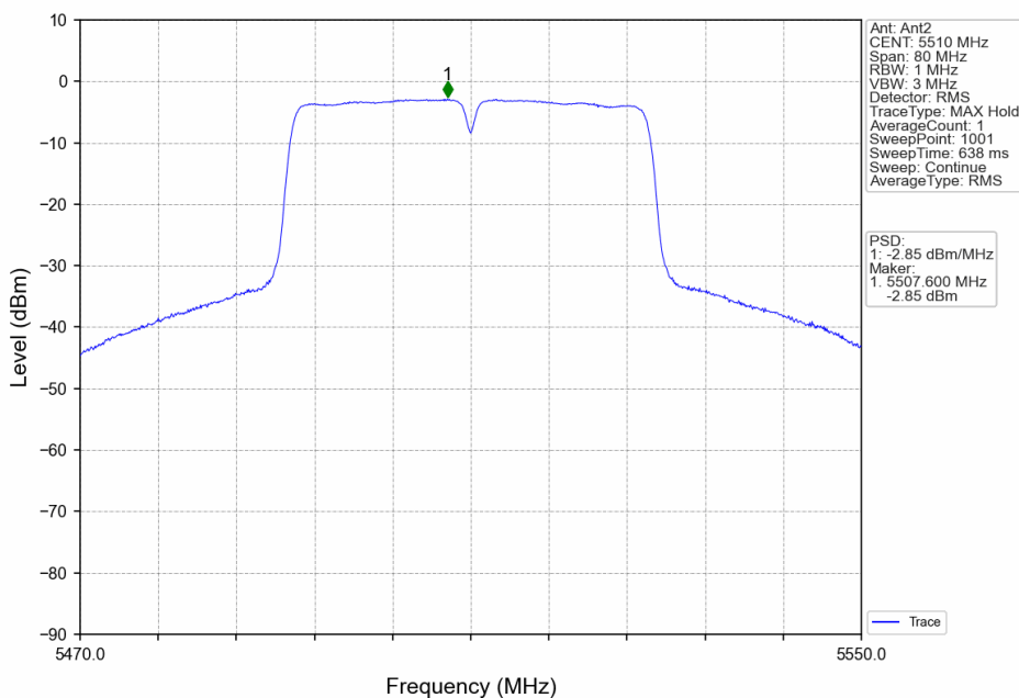
802.11n(HT40)_LCH_5510MHz_MIMO_NTNV
