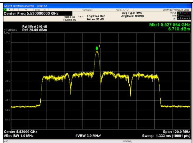
IEEE 802.11ax Channel 106 80MHz_Antenna 0 RU&Index 26RU17
