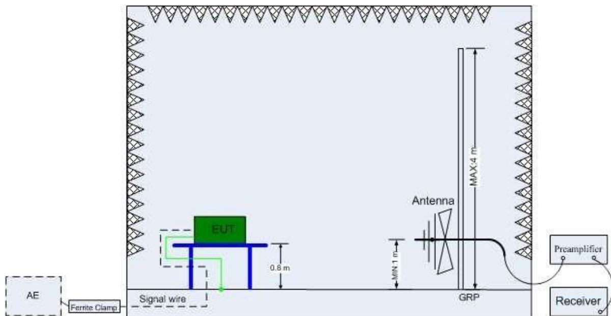
Radiated tests below 1GHz
