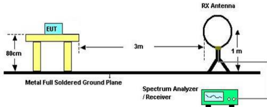
Radiated tests below 1GHz
