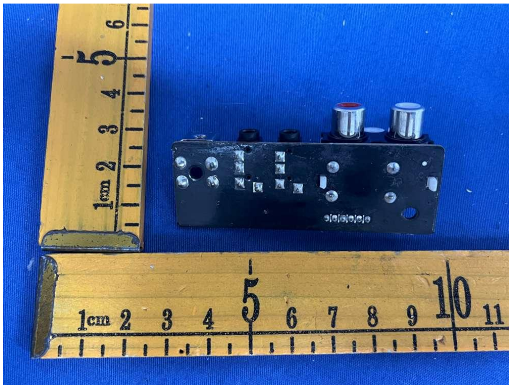
Model 3.1 PCB View
