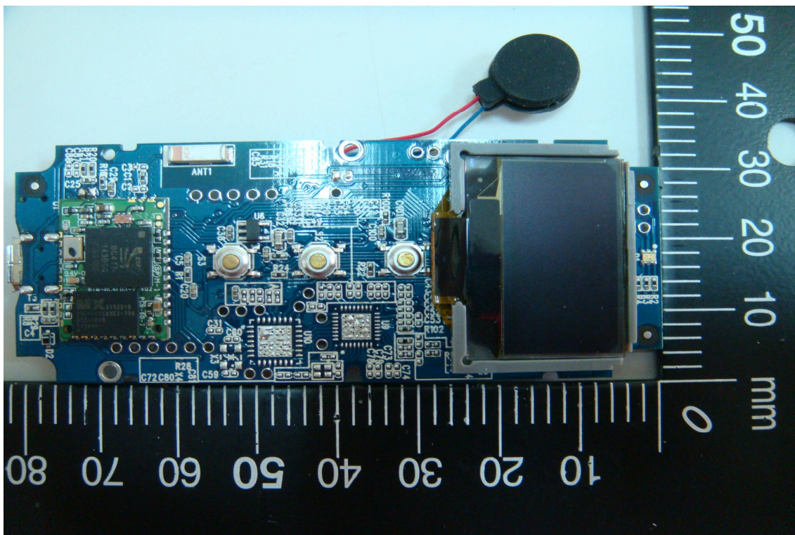
< PCB3-F >
