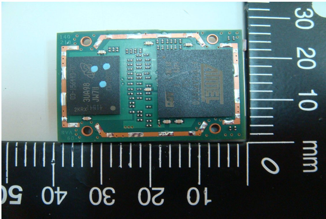
< PCB1-R >
