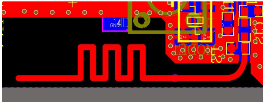
Figure 1 :keyboard Ant
