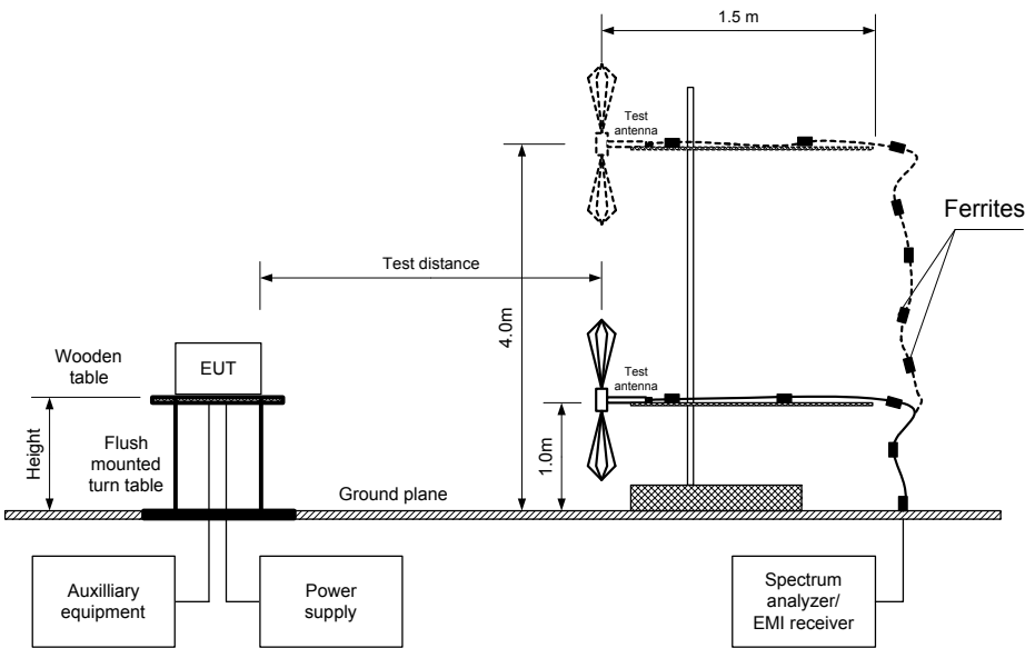
Figure 7.4.1 Band edge emission test setup
