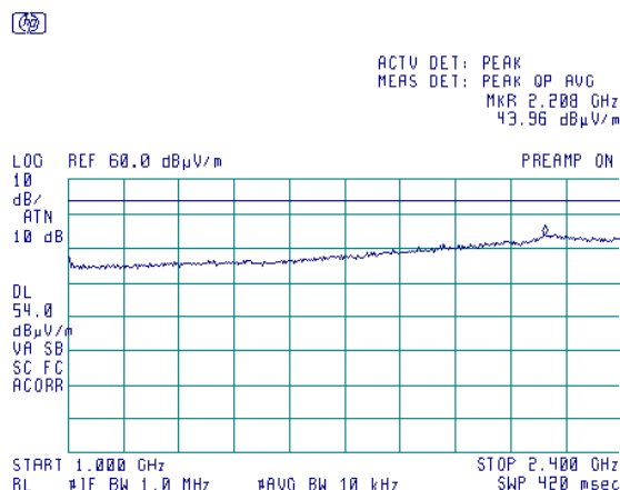
Plot 7.3.11 Radiated emission measurements from 1000 to 2400 MHz at the high carrier frequency 2 ch.26
