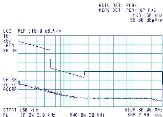
Plot 7.7.8 Radiated emission measurements from 0.15 to 30 MHz at the mid carrier frequency
