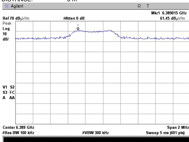
Plot 7.7.38 Radiated emission measurements at the seventh harmonic of mid carrier frequency
