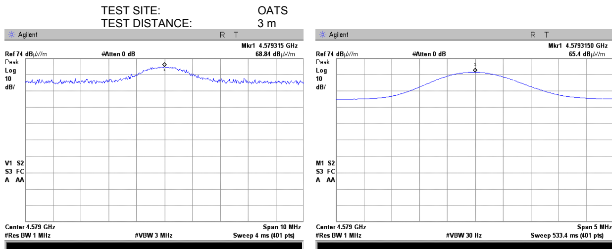
Plot 7.7.32 Radiated emission measurements at the fifth harmonic of mid carrier frequency
