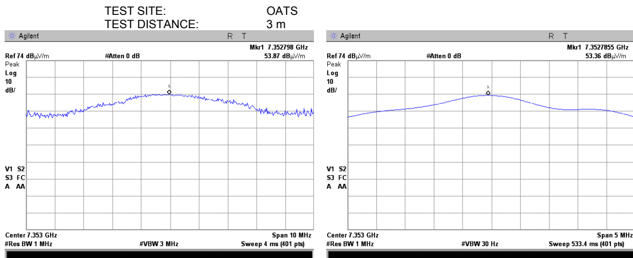
Plot 7.7.42 Radiated emission measurements at the eighth harmonic of high carrier frequency
