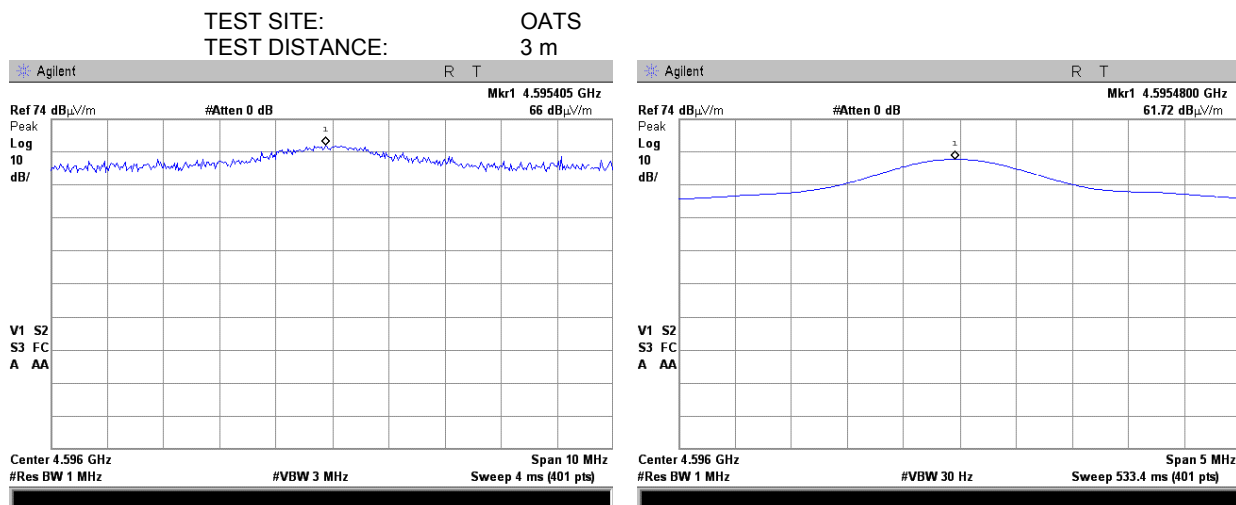
Plot 7.7.33 Radiated emission measurements at the fifth harmonic of high carrier frequency
