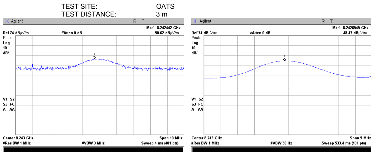
Plot 7.7.44 Radiated emission measurements at the ninth harmonic of mid carrier frequency
