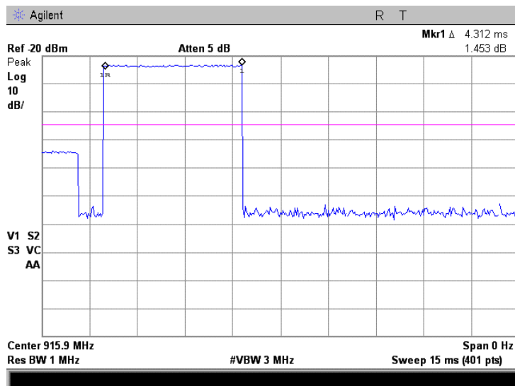
Plot 7.7.49 Transmission pulse duration in normal use
