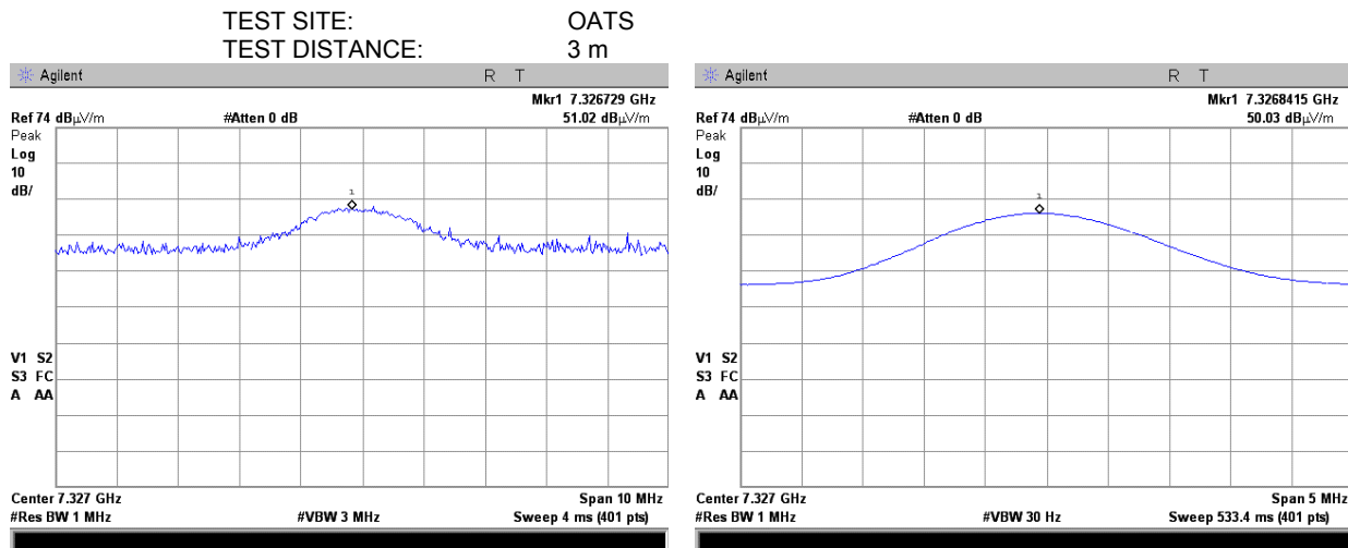
Plot 7.7.41 Radiated emission measurements at the eighth harmonic of mid carrier frequency
