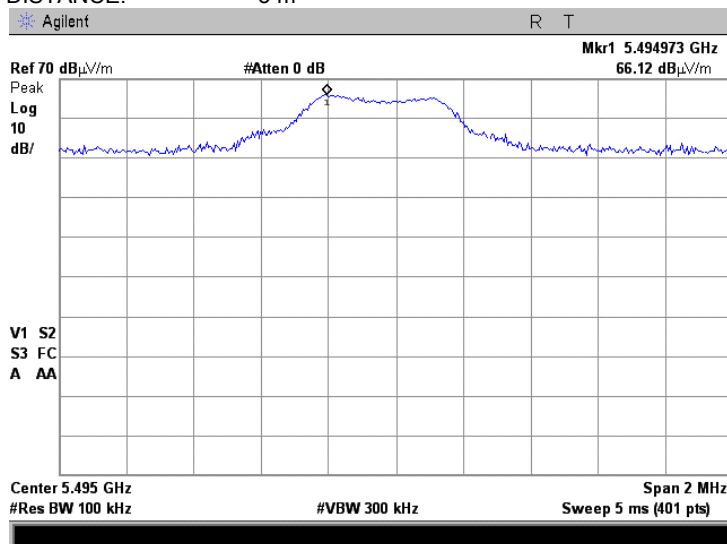
Plot 7.7.36 Radiated emission measurements at the sixth harmonic of high carrier frequency
