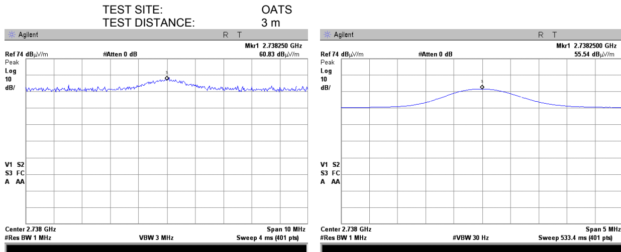
Plot 7.7.25 Radiated emission measurements at the third harmonic of low carrier frequency
