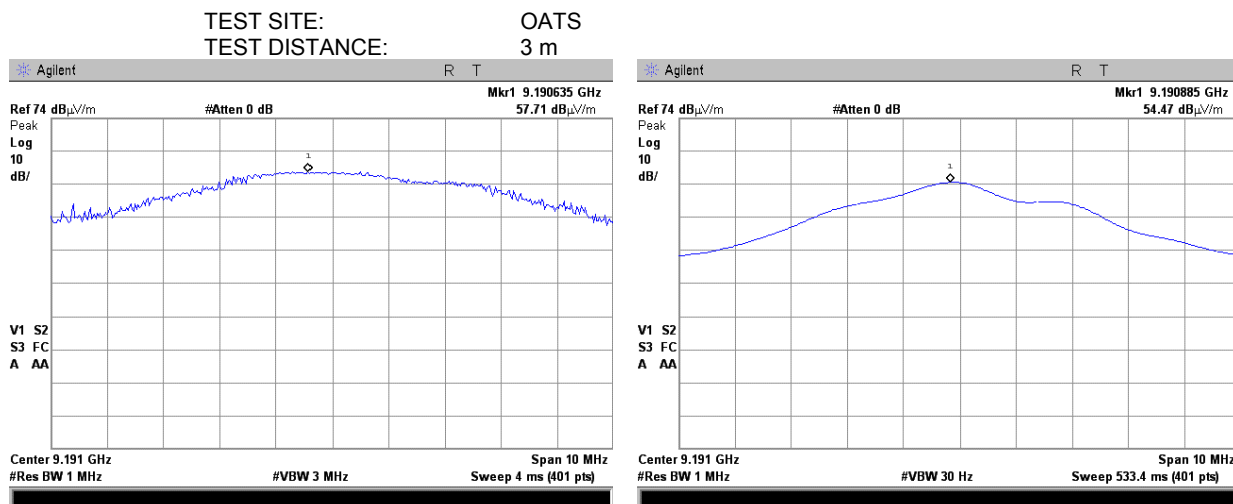
Plot 7.7.48 Radiated emission measurements at the tenth harmonic of high carrier frequency
