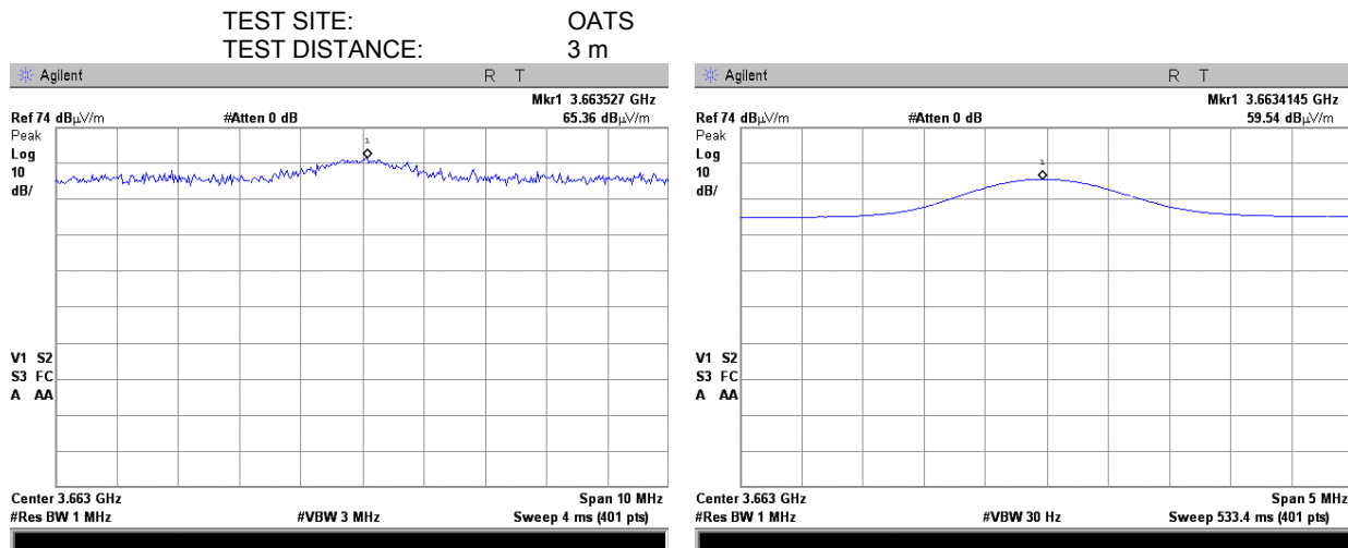
Plot 7.7.29 Radiated emission measurements at the fourth harmonic of mid carrier frequency
