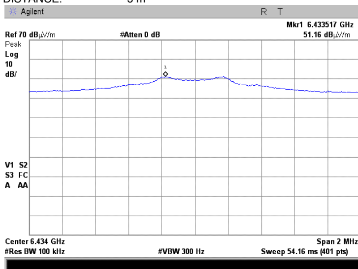
Plot 7.7.40 Radiated emission measurements at the eighth harmonic of low carrier frequency
