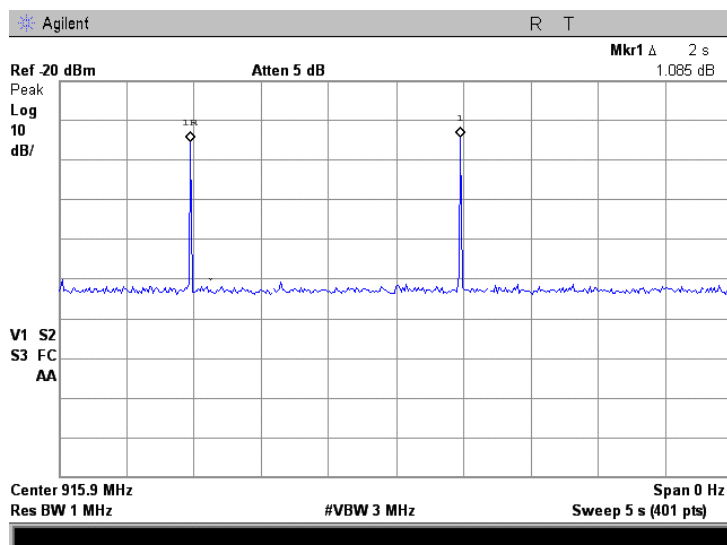
Plot 7.7.50 Transmission pulse period in normal use
