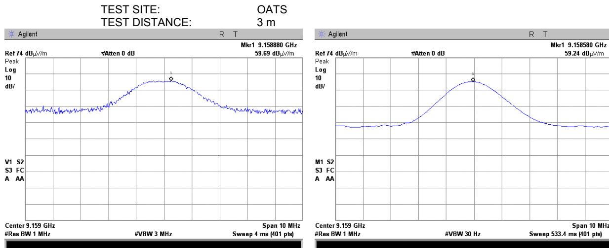
Plot 7.7.47 Radiated emission measurements at the tenth harmonic of mid carrier frequency
