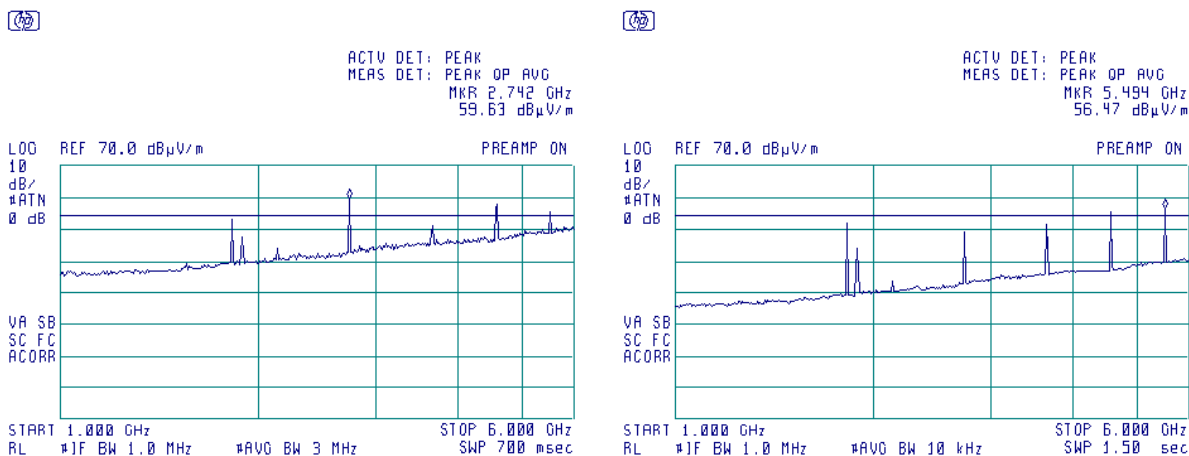
Plot 7.7.18 Radiated emission measurements from 1000 to 6000 MHz at the high carrier frequency
