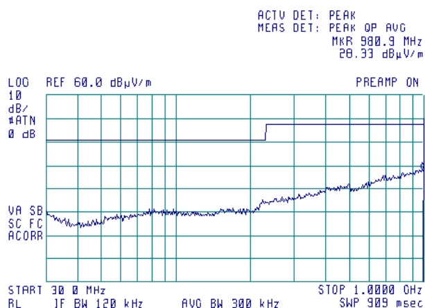
Plot 8.1.4 Radiated emissions measurements in 30 - 1000 MHz range according to ICES-003
