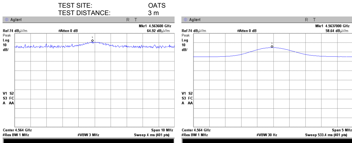
Plot 7.7.31 Radiated emission measurements at the fifth harmonic of low carrier frequency
