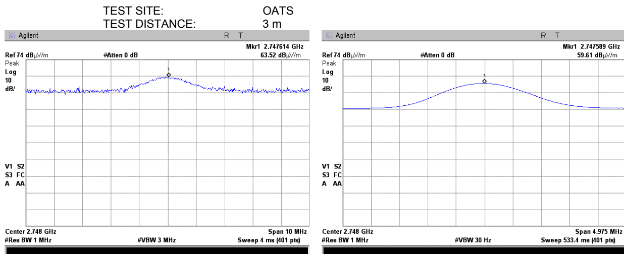
Plot 7.7.26 Radiated emission measurements at the third harmonic of mid carrier frequency
