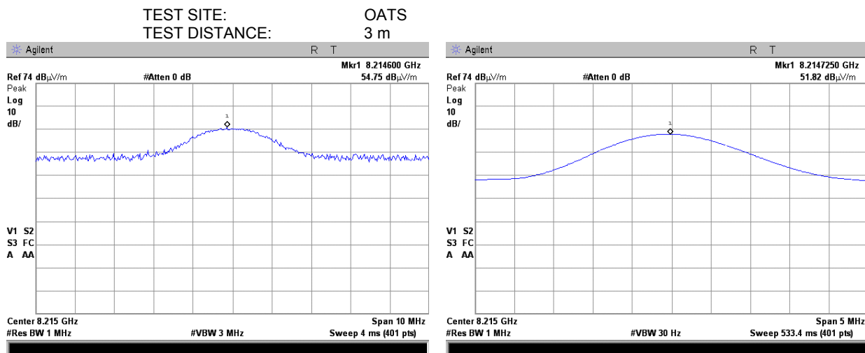
Plot 7.7.43 Radiated emission measurements at the ninth harmonic of low carrier frequency
