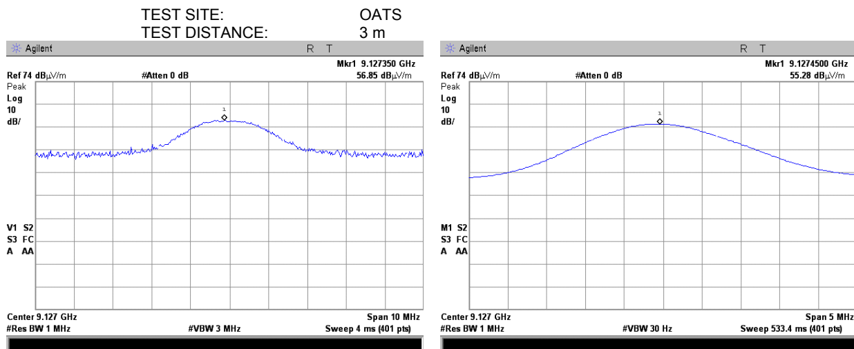
Plot 7.7.46 Radiated emission measurements at the tenth harmonic of low carrier frequency
