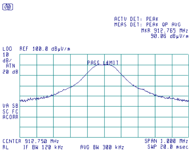
Plot 7.5.1 Field strength of carrier at low frequency in vertical antenna polarization
