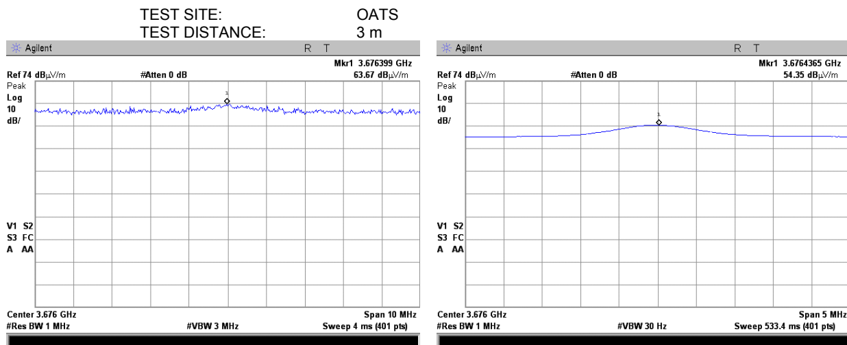
Plot 7.7.30 Radiated emission measurements at the fourth harmonic of high carrier frequency
