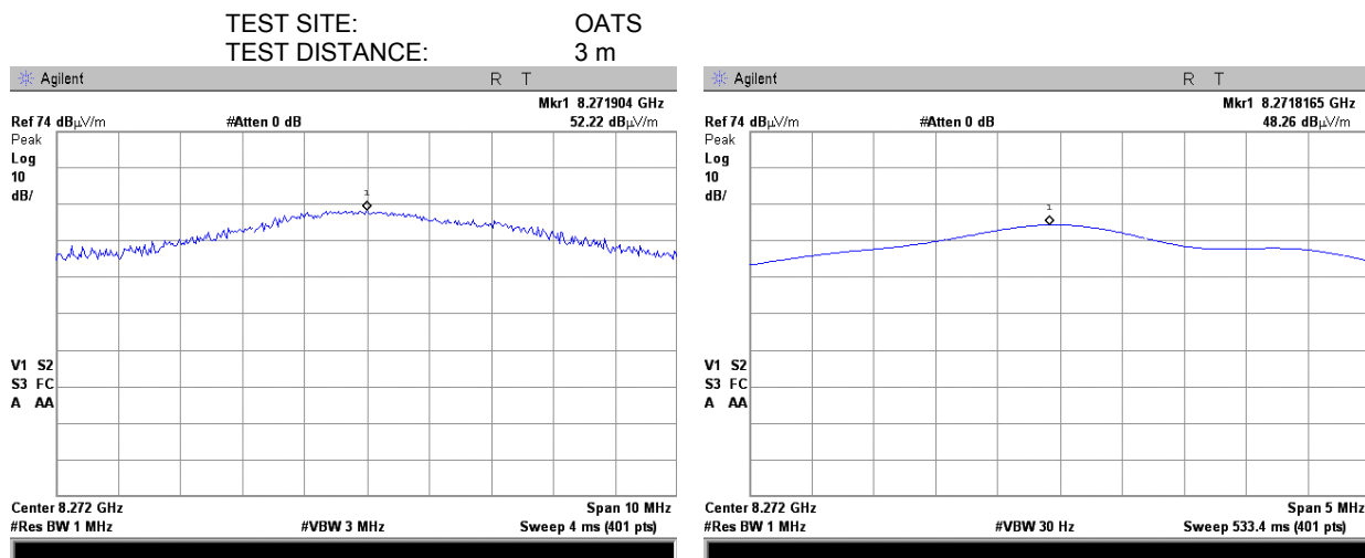
Plot 7.7.45 Radiated emission measurements at the ninth harmonic of high carrier frequency
