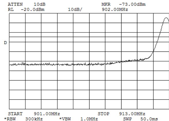
Plot 7.6.1 The highest band edge emission at low carrier frequency with hopping function disabled
