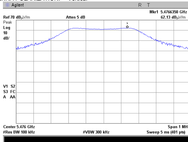
Plot 7.7.45 Radiated emission measurements at the sixth harmonic of low carrier frequency
