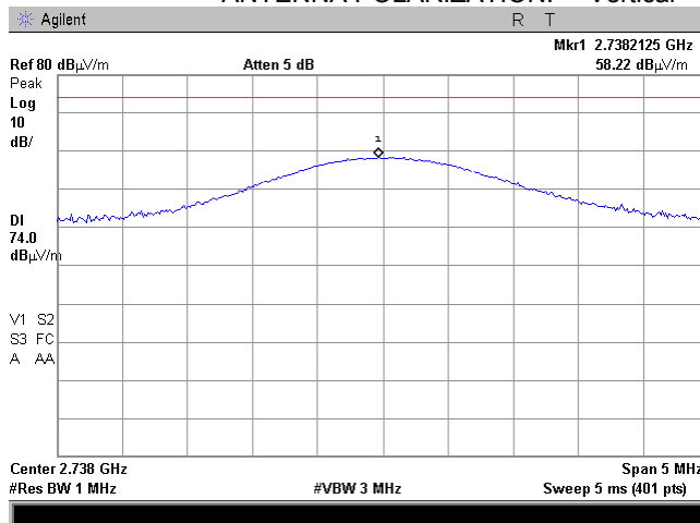
Plot 7.7.27 Radiated emission measurements at the third harmonic of low carrier frequency
