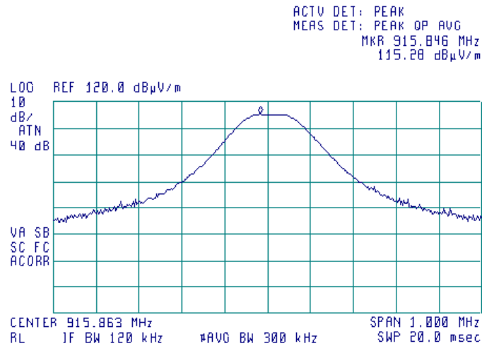
Plot 7.5.16 Peak output power at mid frequency and 85%Unom, horizontal antenna polarization
