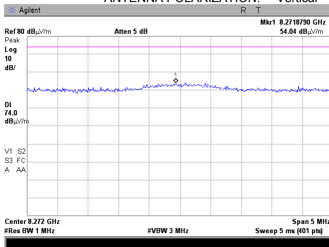
Plot 7.7.67 Radiated emission measurements at the ninth harmonic of high carrier frequency
