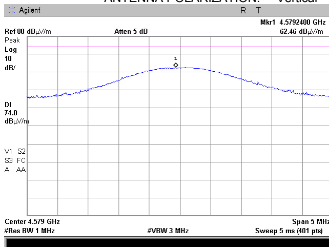
Plot 7.7.41 Radiated emission measurements at the fifth harmonic of mid carrier frequency
