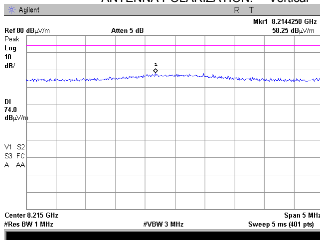
Plot 7.7.63 Radiated emission measurements at the ninth harmonic of low carrier frequency
