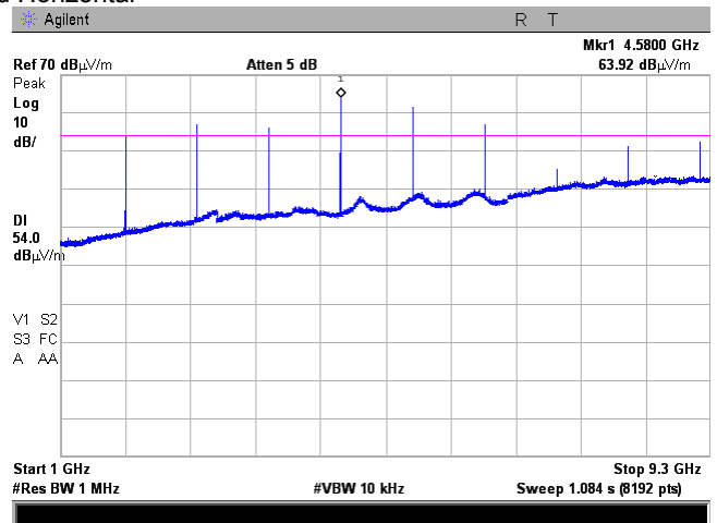
Plot 7.7.19 Radiated emission measurements from 1000 to 9300 MHz at the high carrier frequency
