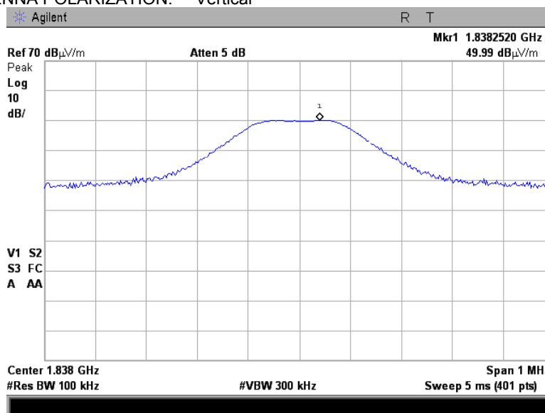
Plot 7.7.25 Radiated emission measurements at the second harmonic of high carrier frequency
