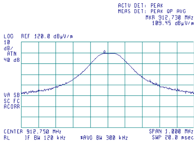
Plot 7.5.14 Peak output power at low frequency and 85%Unom, horizontal antenna polarization
