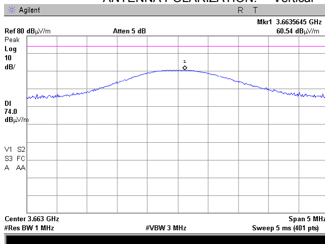
Plot 7.7.35 Radiated emission measurements at the fourth harmonic of mid carrier frequency
