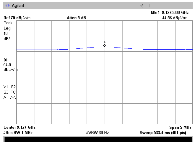
Plot 7.7.69 Radiated emission measurements at the tenth harmonic of low carrier frequency
