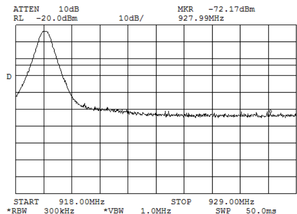
Plot 7.6.2 The highest band edge emission at high carrier frequency with hopping function disabled
