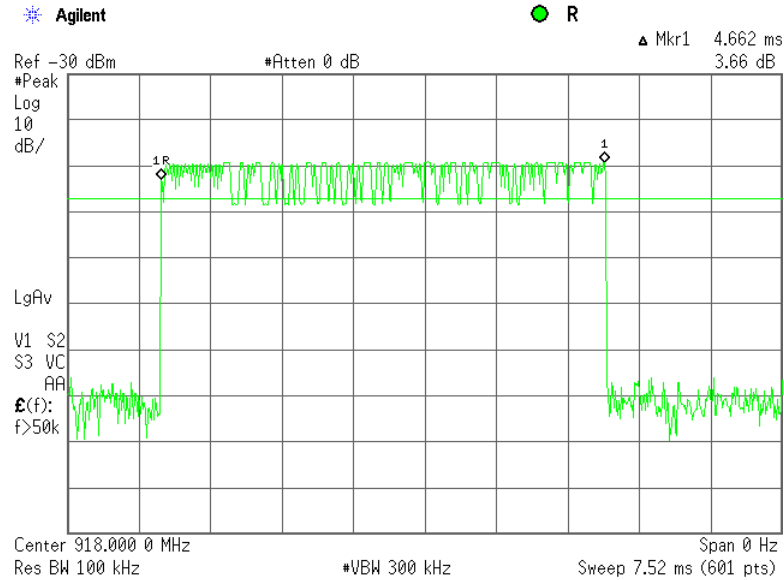
Plot 7.7.74 Transmission pulse duration
