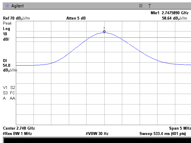
Plot 7.7.29 Radiated emission measurements at the third harmonic of mid carrier frequency
