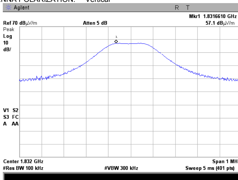
Plot 7.7.23 Radiated emission measurements at the second harmonic of mid carrier frequency
