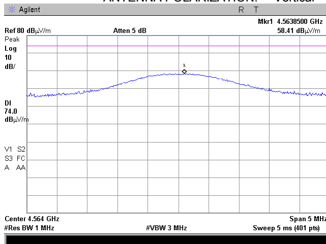
Plot 7.7.39 Radiated emission measurements at the fifth harmonic of low carrier frequency
