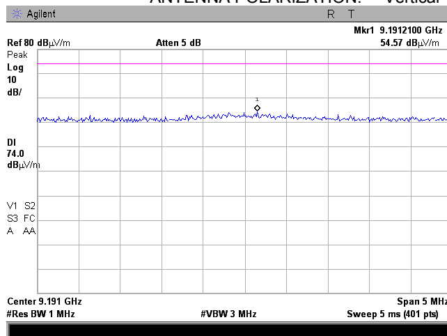
Plot 7.7.73 Radiated emission measurements at the tenth harmonic of high carrier frequency
