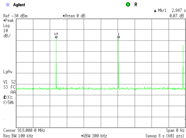
Plot 7.7.75 Transmission pulse period
