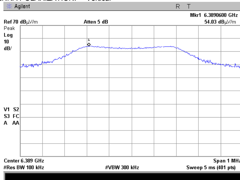
Plot 7.7.51 Radiated emission measurements at the seventh harmonic of low carrier frequency
