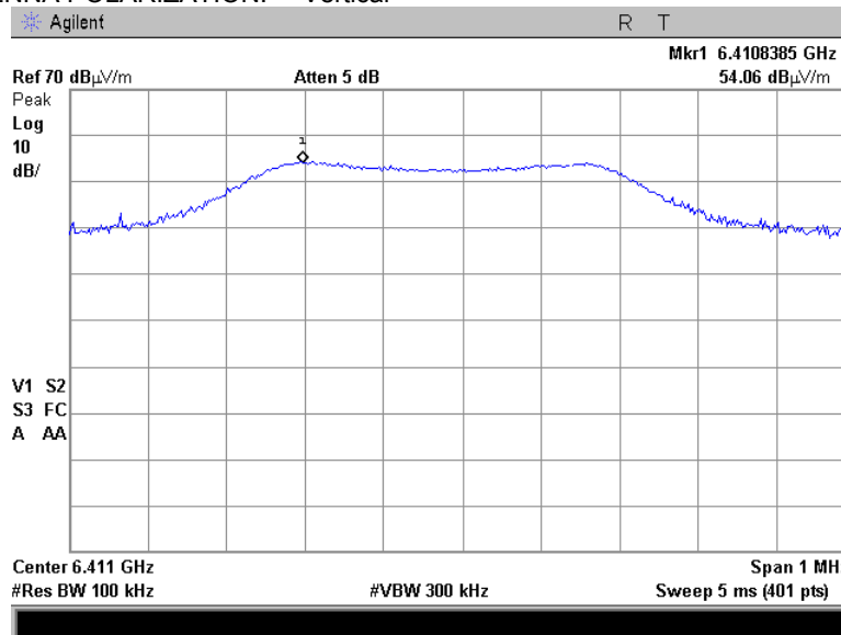
Plot 7.7.53 Radiated emission measurements at the seventh harmonic of mid carrier frequency
