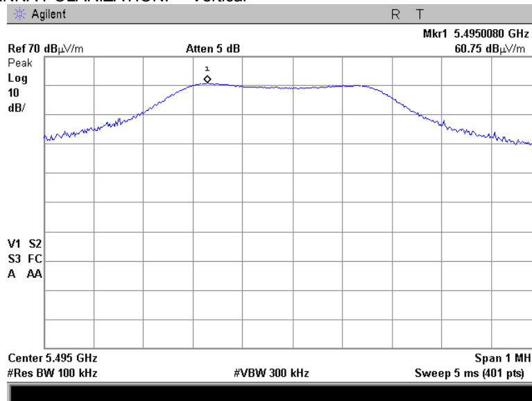
Plot 7.7.47 Radiated emission measurements at the sixth harmonic of mid carrier frequency
