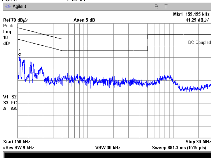
Plot 7.9.2 Conducted emission measurements
