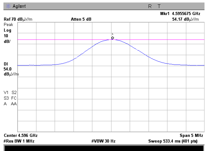
Plot 7.7.43 Radiated emission measurements at the fifth harmonic of high carrier frequency
