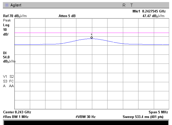
Plot 7.7.65 Radiated emission measurements at the ninth harmonic of mid carrier frequency
