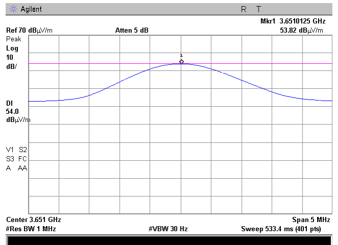
Plot 7.7.33 Radiated emission measurements at the fourth harmonic of low carrier frequency
