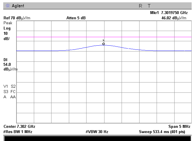
Plot 7.7.57 Radiated emission measurements at the eighth harmonic of low carrier frequency
