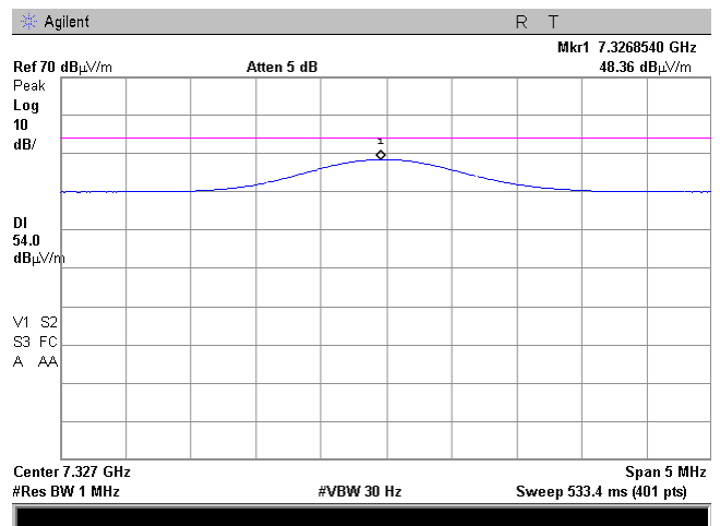
Plot 7.7.59 Radiated emission measurements at the eighth harmonic of mid carrier frequency
