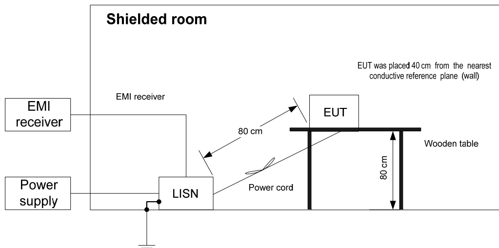
Figure 7.9.1 Setup for conducted emission measurements, table-top equipment
