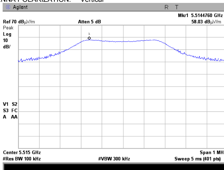
Plot 7.7.49 Radiated emission measurements at the sixth harmonic of high carrier frequency
