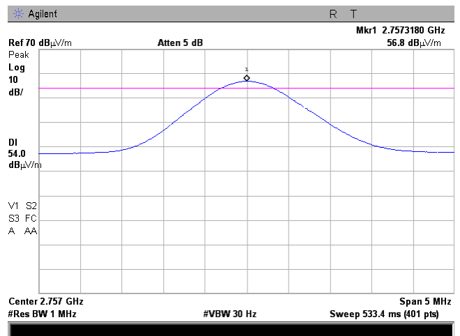
Plot 7.7.31 Radiated emission measurements at the third harmonic of high carrier frequency
