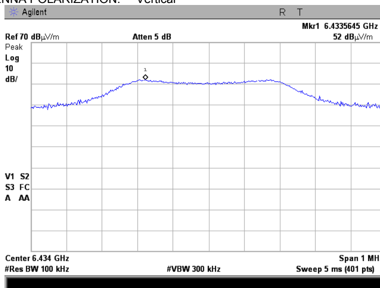
Plot 7.7.55 Radiated emission measurements at the seventh harmonic of high carrier frequency
