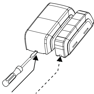
Figure 2 - Decorative cover removal
