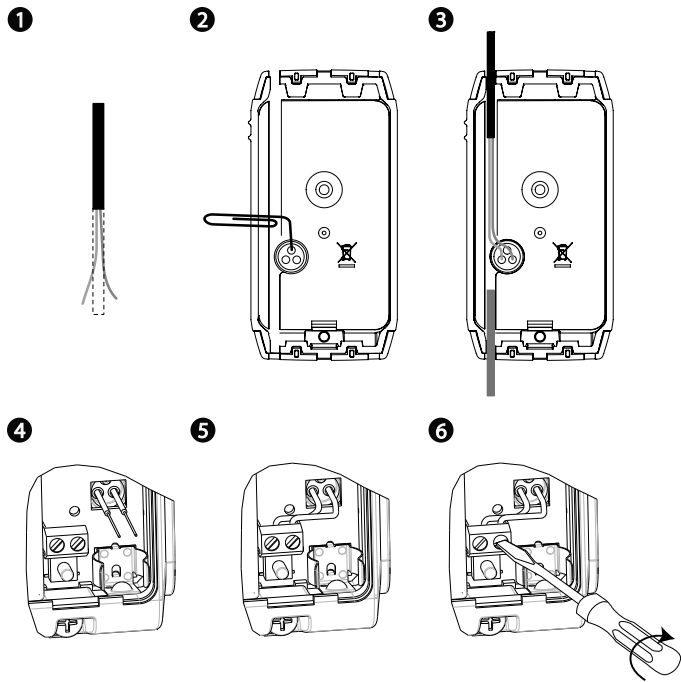
Figure 9 - Auxiliary wiring
