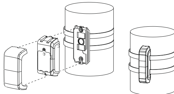
Figure 6 - Curved surface mounting
