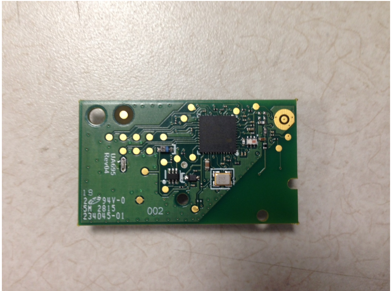
MCT-350 SMA (UA695 Rev 05) PCB assembly rear side view
