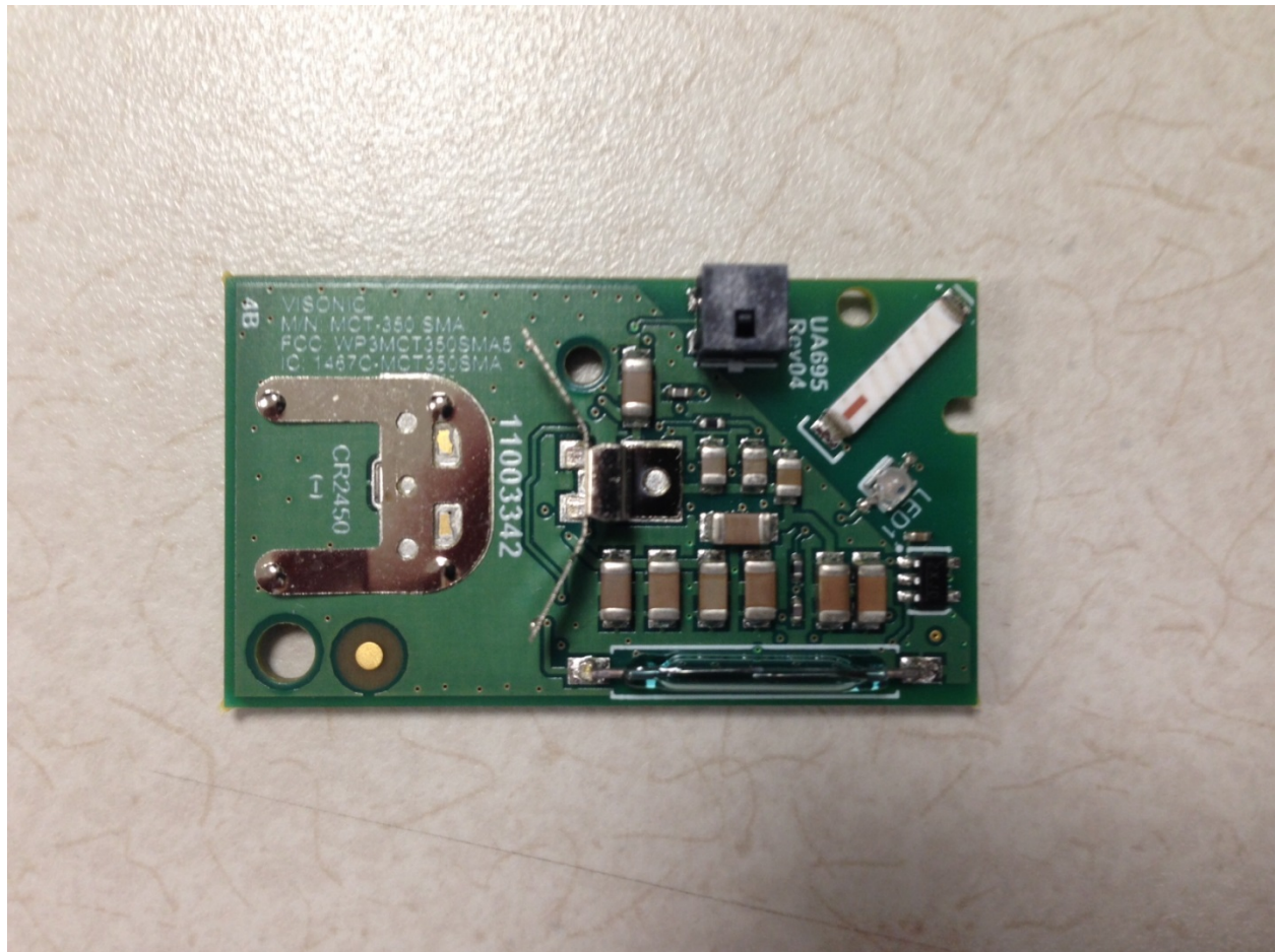
MCT-350 SMA (UA695 Rev 05) PCB assembly top side view
