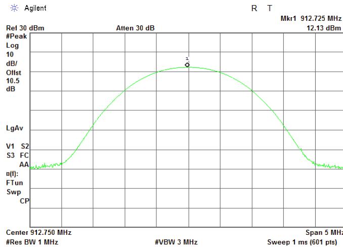
Plot 7.5.2 Peak output power at mid frequency
