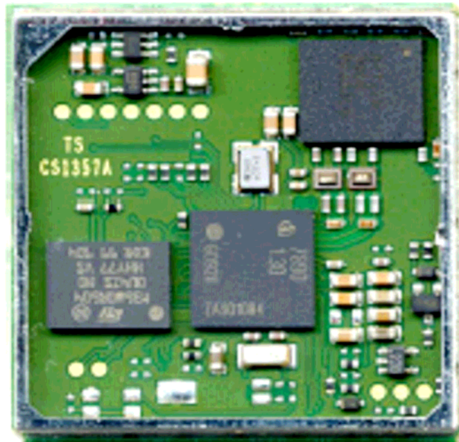
Photograph No.20 GE864-Quad V2 module PCB front view
