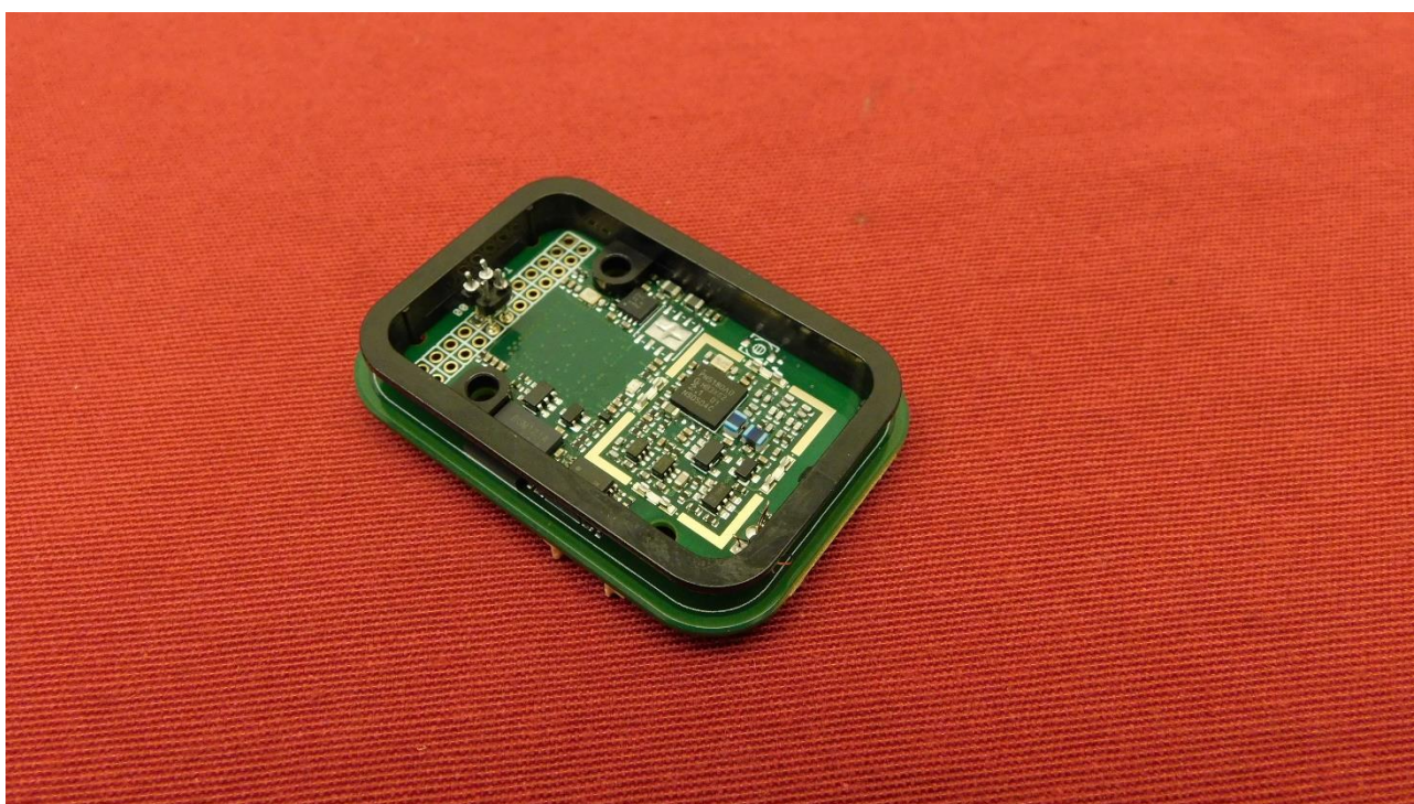
Picture 6: PCB 1 of EUT - bottom view without shielding
