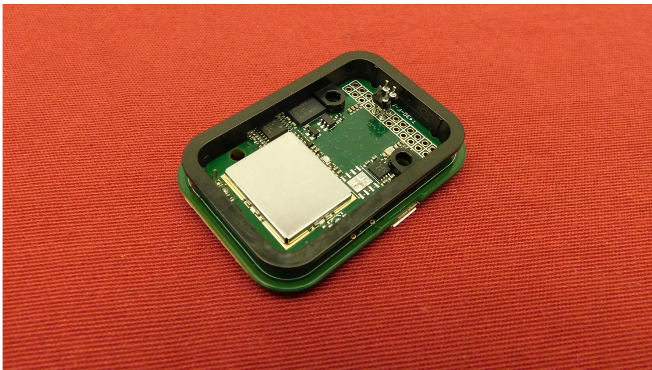
Picture 5: PCB 1 of EUT - bottom view with shielding
