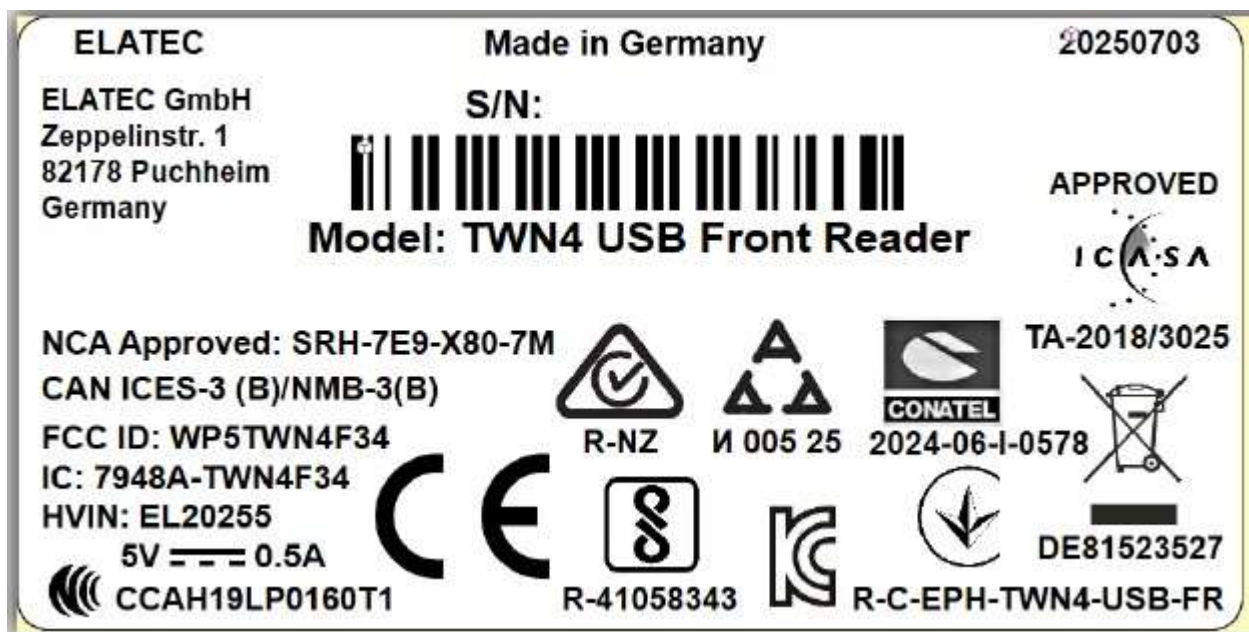
Picture2: Name plate of EUT
