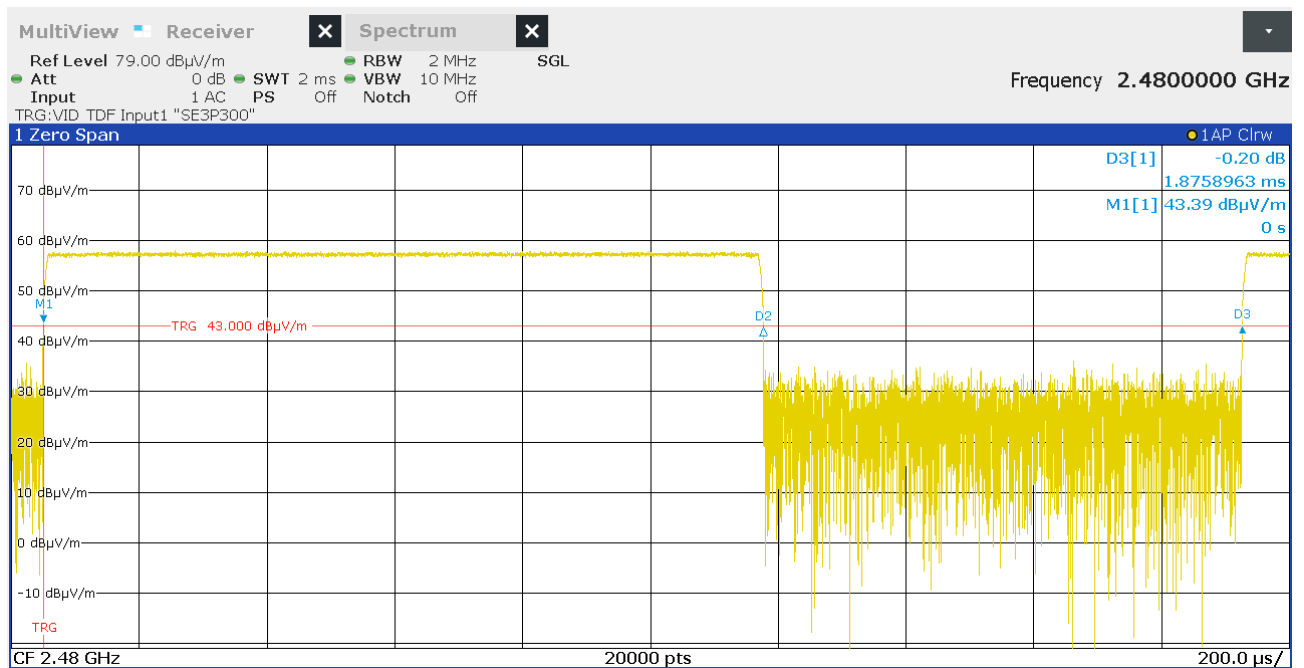
Figure 8: Chart of duty cycle test on highest channel
