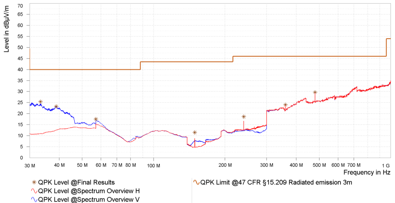
Figure 24: Chart of radiated emissions test from 30 MHz to 1 GHz on lowest channel, EUT position X, antenna polarization horizontal and vertical
