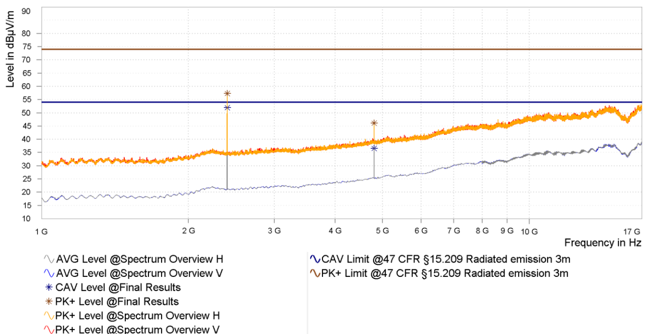
Figure 25: Chart of radiated emissions pre-measurement from 1 GHz to 17 GHz on lowest channel, EUT position X, antenna polarization horizontal and vertical
