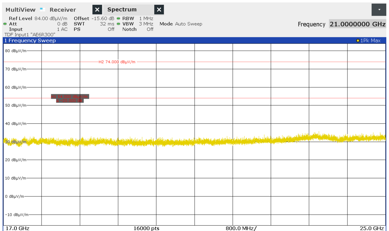
Figure 30: Chart of exploratory emissions measurement from 17 GHz to 25 GHz on highest channel, EUT position Y, antenna polarization vertical
