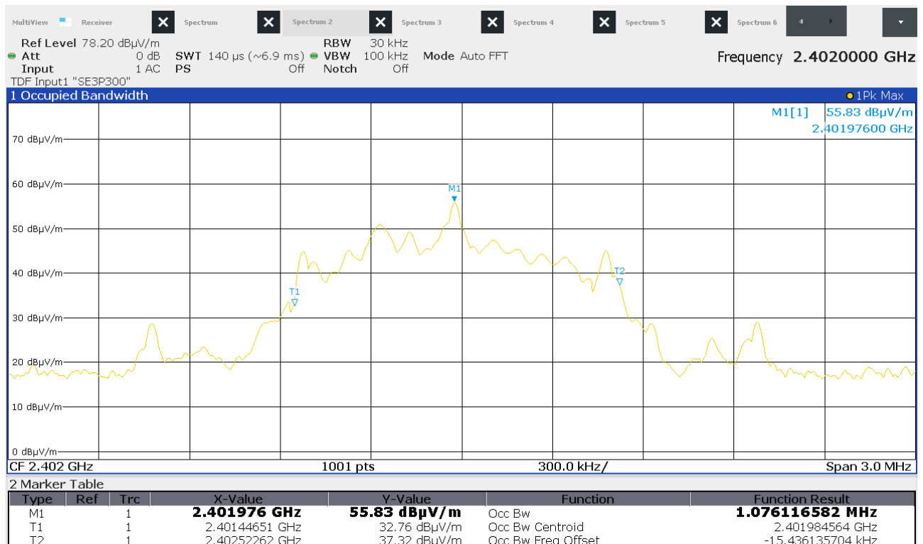
Figure 12: Chart of occupied bandwidth test on lowest channel
