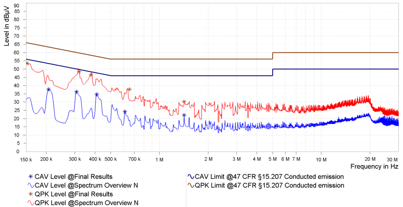
Figure 7: Chart of AC powerline conducted emissions on N
