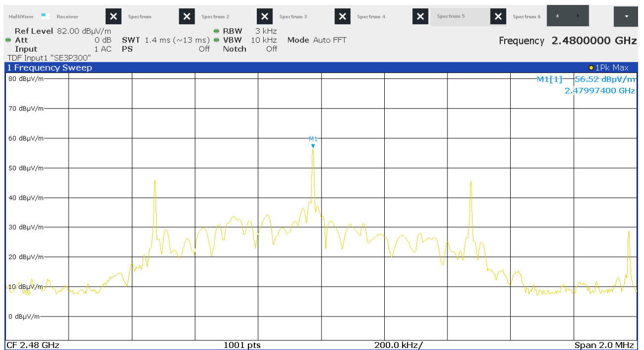
Figure 20: Chart of radiated power spectral density on highest channel
