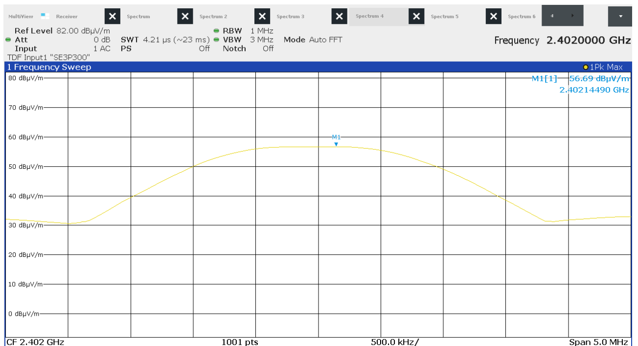
Figure 15: Chart of field strength at 3 m on lowest channel, EUT position X, antenna polarization horizontal
