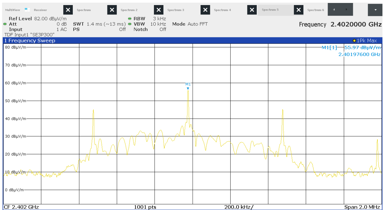
Figure 18: Chart of radiated power spectral density on lowest channel
