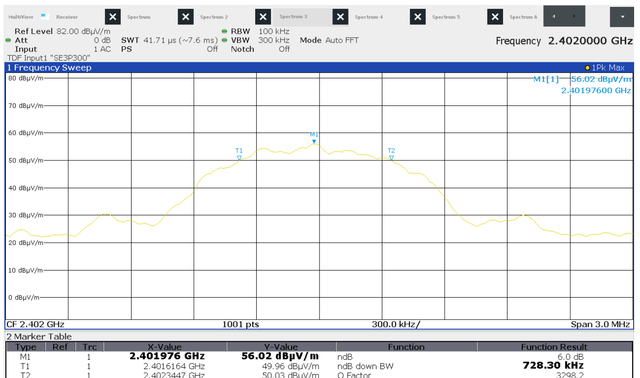
Figure 9: Chart of 6 dB bandwidth test on lowest channel
