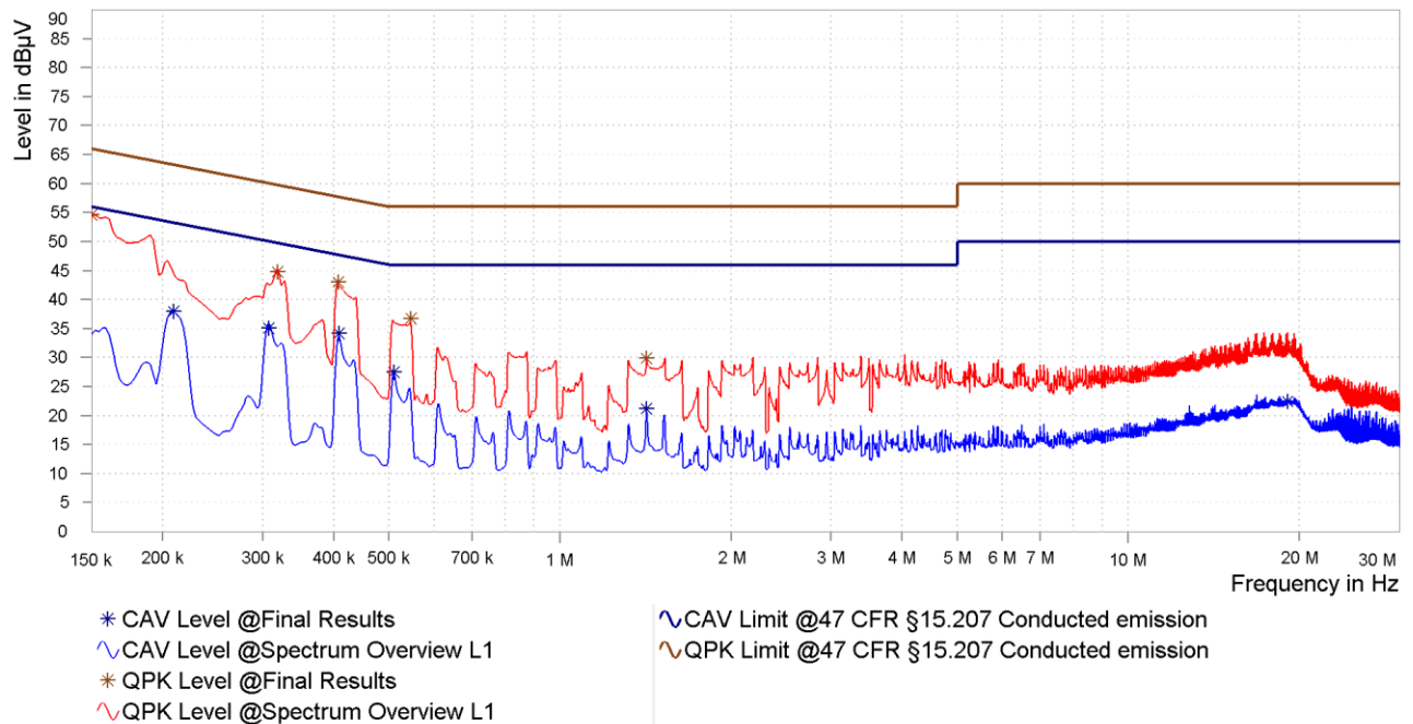
Figure 6: Chart of AC powerline conducted emissions on L1
