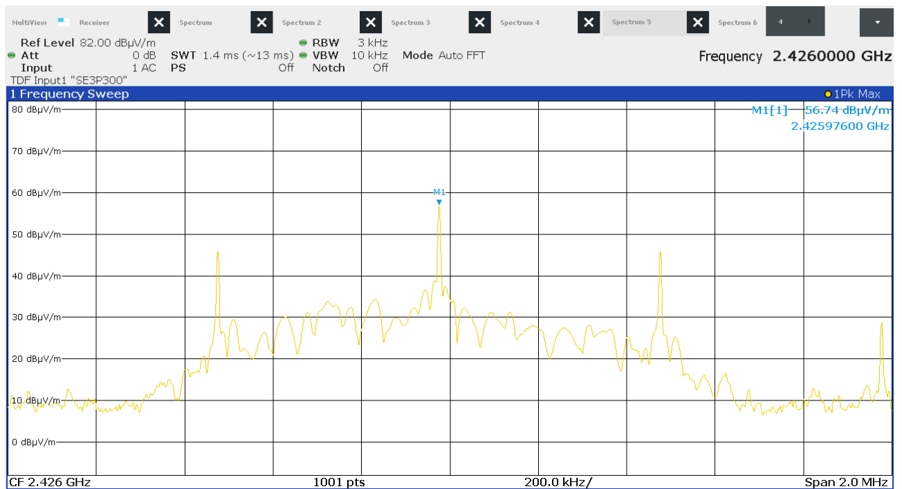
Figure 19: Chart of radiated power spectral density on middle channel
