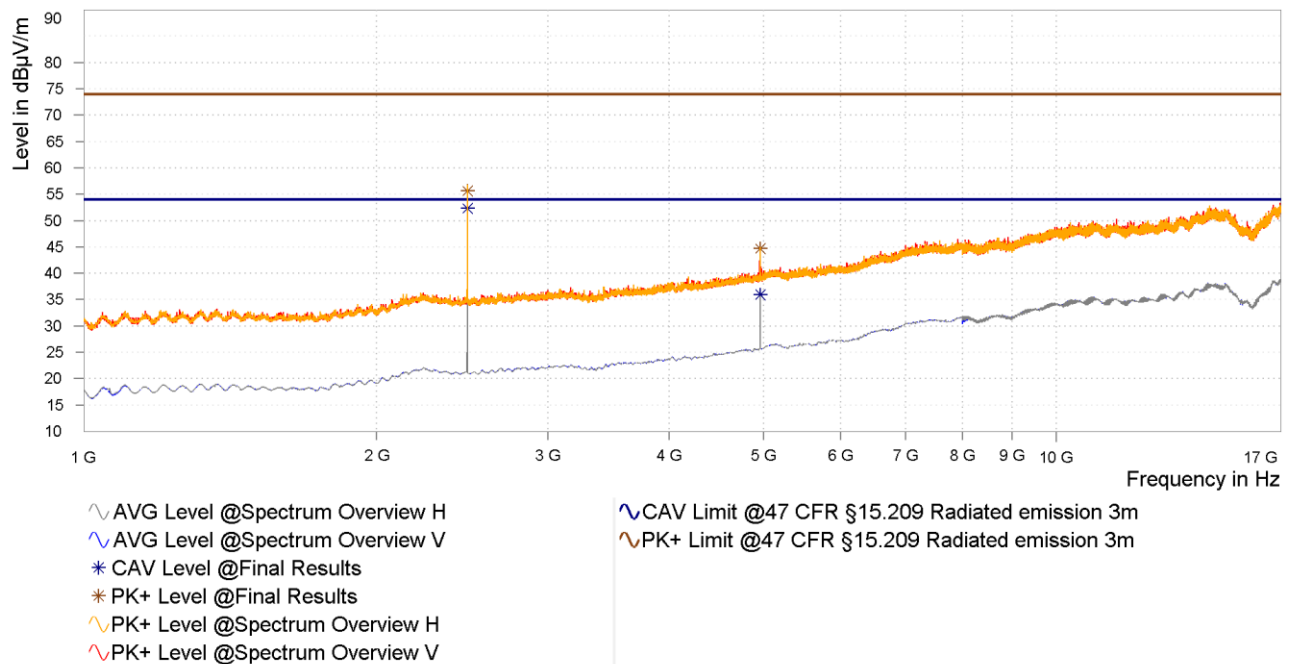
Figure 29: Chart of radiated emissions pre-measurement from 1 GHz to 17 GHz on highest channel, EUT position X, antenna polarization horizontal and vertical
