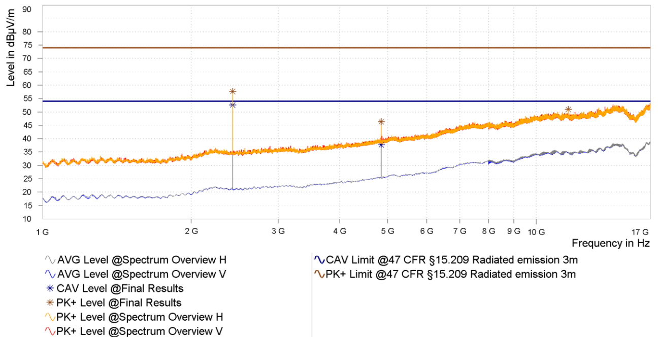
Figure 27: Chart of radiated emissions pre-measurement from 1 GHz to 17 GHz on middle channel, EUT position X, antenna polarization horizontal and vertical.
