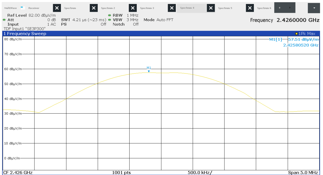
Figure 16: Chart of field strength at 3 m on middle channel, EUT position X, antenna polarization horizontal
