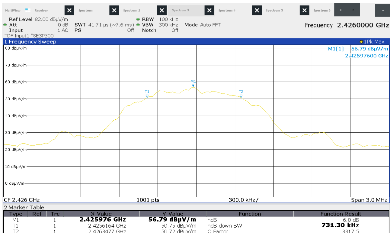
Figure 10: Chart of 6 dB bandwidth test on middle channel
