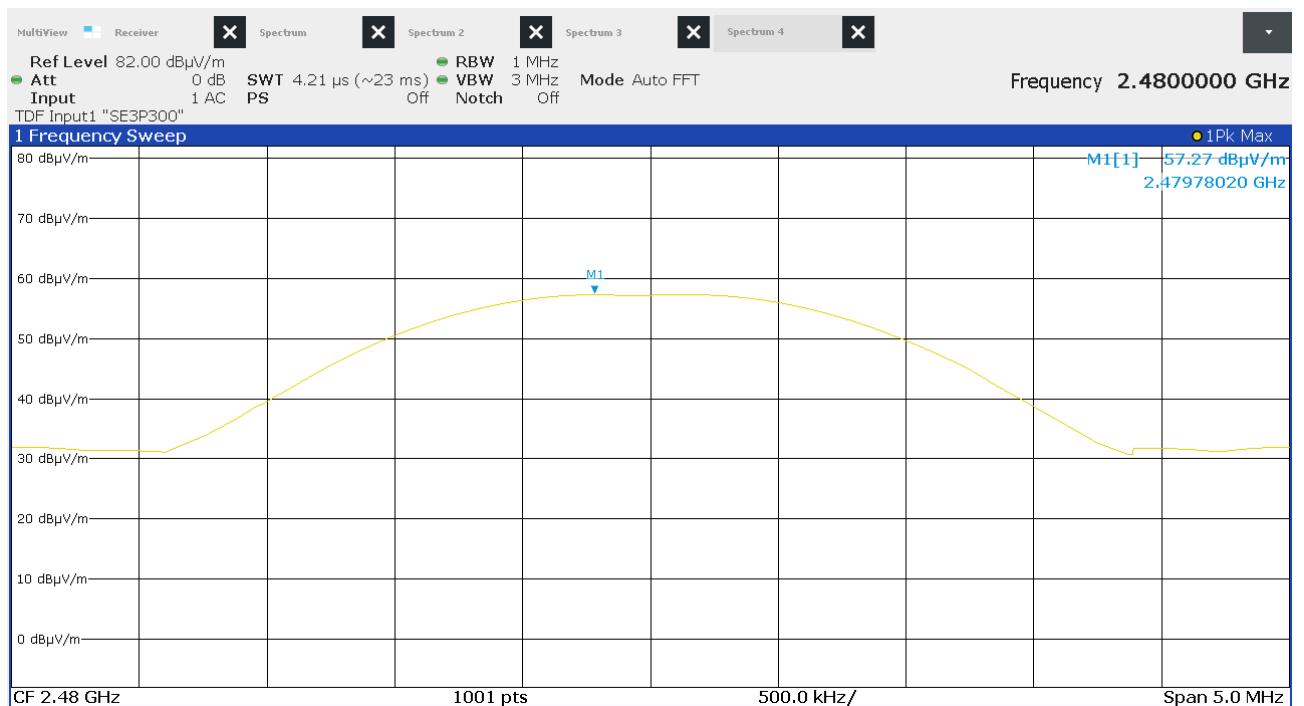
Figure 17: Chart of field strength at 3 m on highest channel, EUT position X, antenna polarization horizontal
