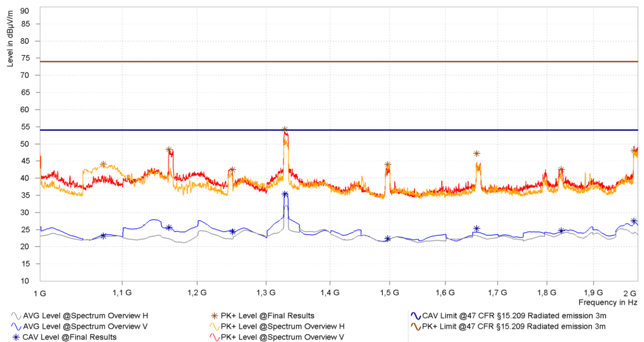
Figure 15: Chart of emissions test from 1 GHz to 2 GHz, EUT position Z, antenna polarization horizontal and vertical, with tag
