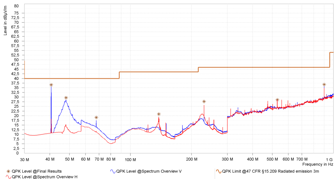
Figure 14: Chart of radiated emissions test from 30 MHz to 1 GHz, EUT position Z, antenna polarization horizontal and vertical, with tag
