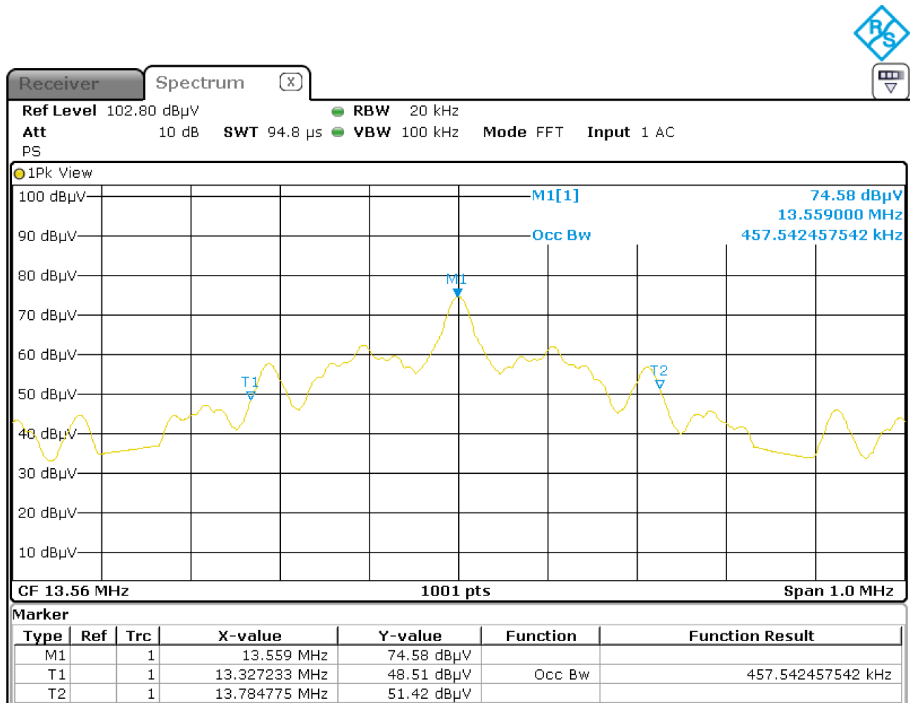
Figure 11: Chart of occupied bandwidth test, with tag
