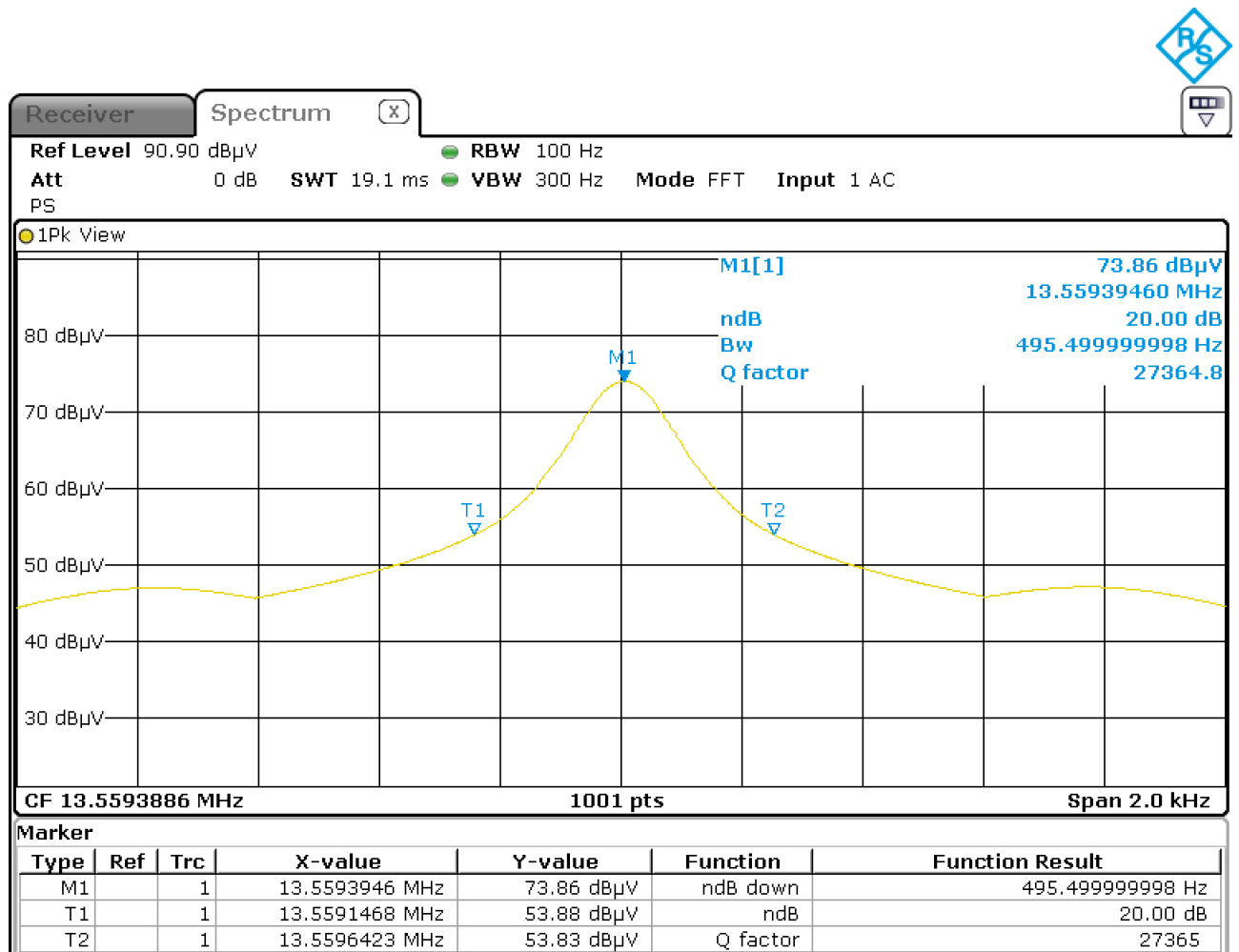
Figure 10: Chart of 20 dB bandwidth test at normal conditions, with tag
