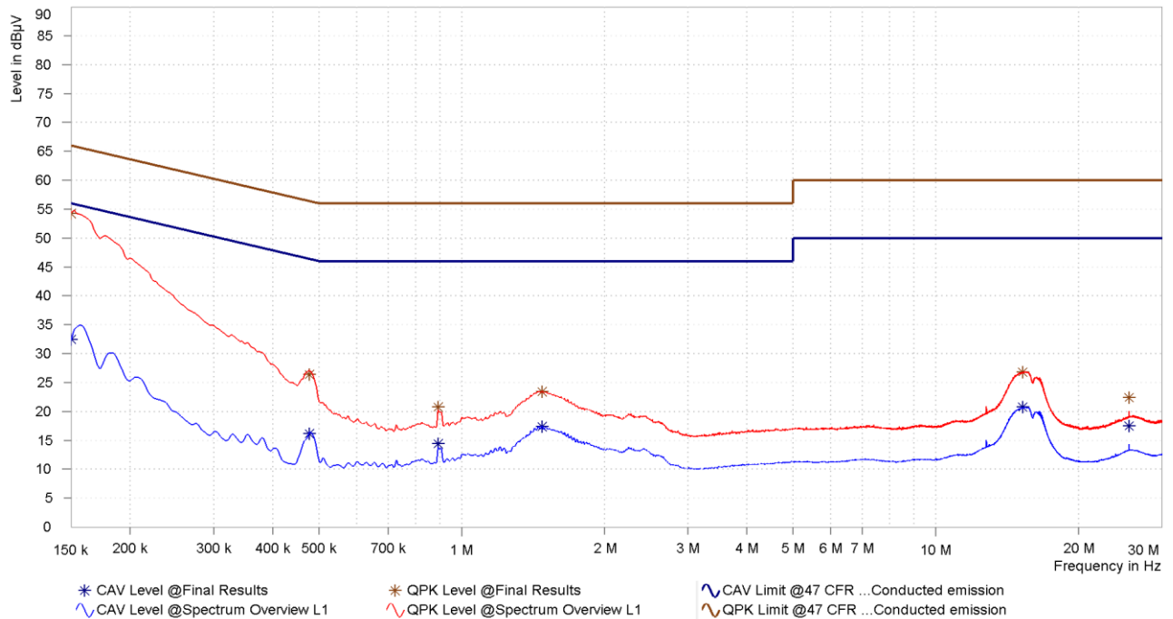
Figure 8: Chart of AC powerline conducted emissions on L1
