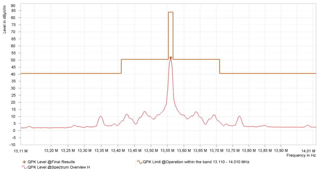
Figure 12: Chart of emission within the band 13.110 MHz to 14.010 MHz, EUT in position Z, without tag, antenna in line
