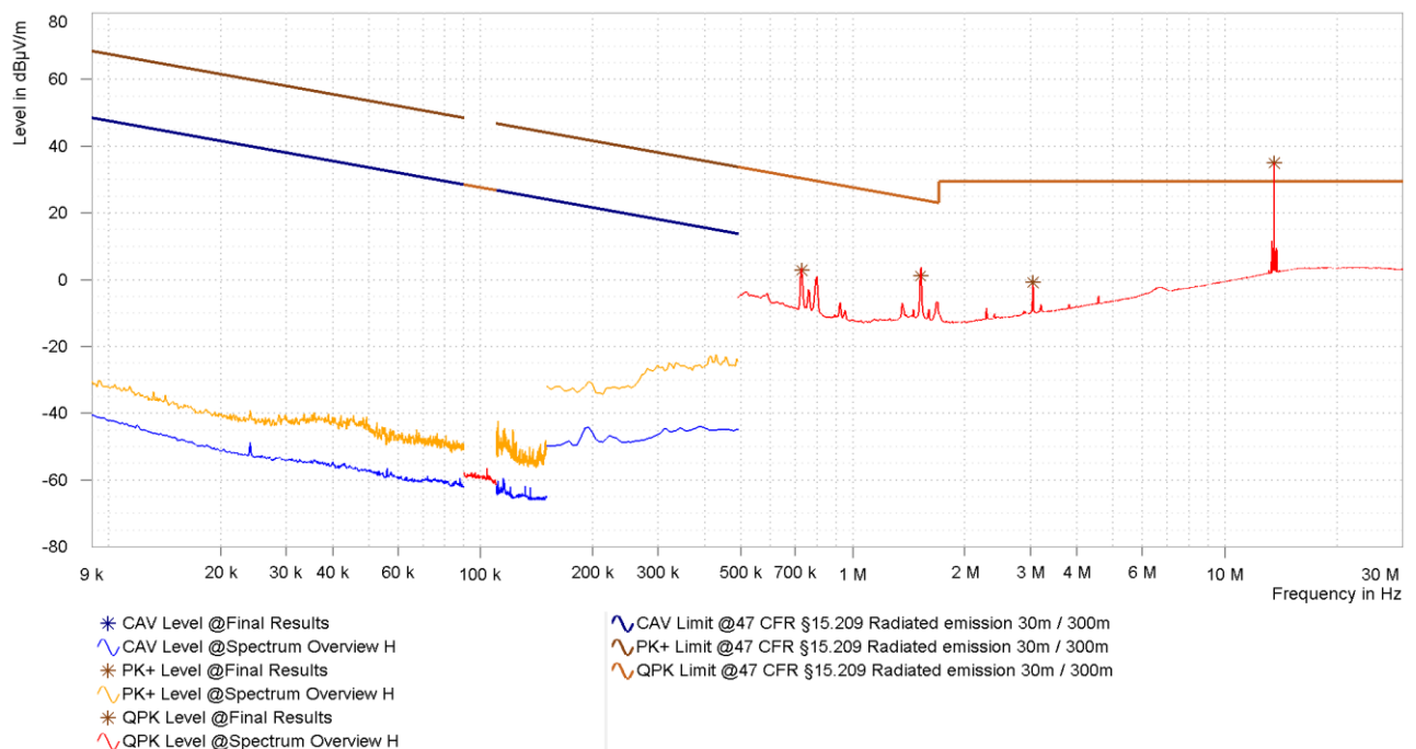
Figure 13: Chart of radiated emissions test below 30 MHz, EUT position X, antenna polarization parallel, with tag
