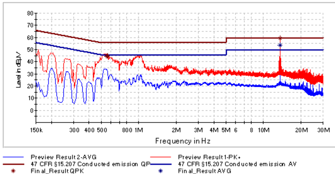
Picture 4: Graphic - Conducted emission on mains, neutral (without termination)
