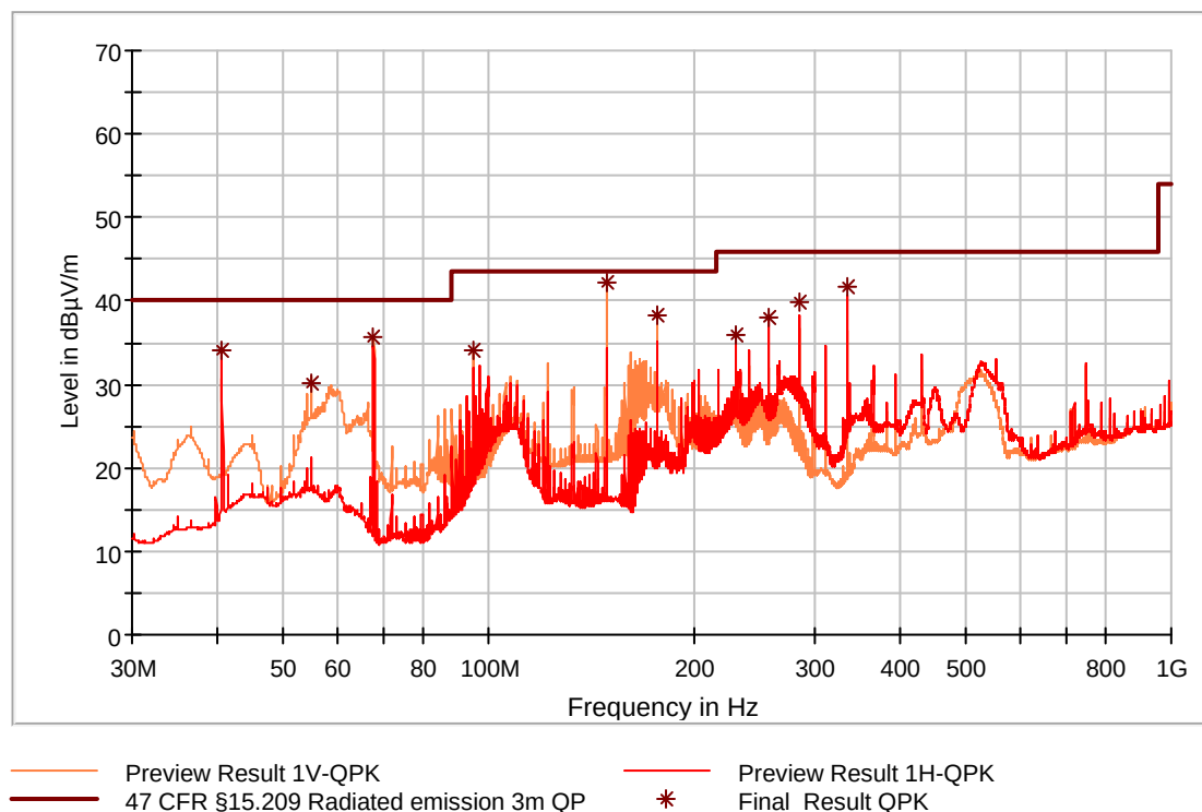
Picture 13: Radiated emission 30 MHz - 1 GHz @ 3 m distance
