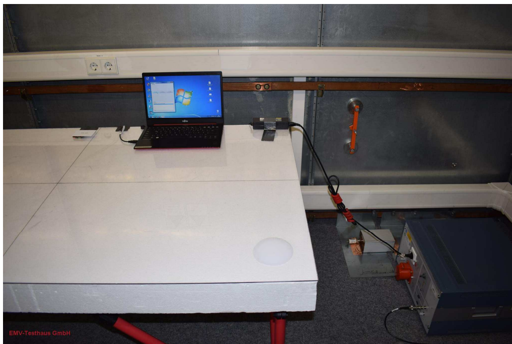
Picture 5: Test setup AC power line conducted emissions (front view)
