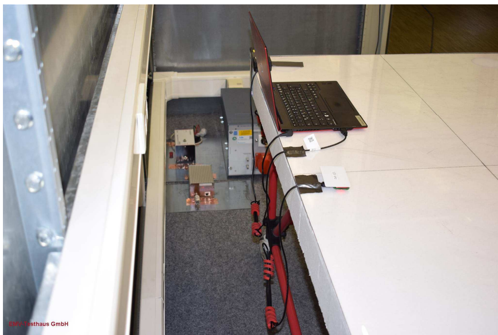
Picture 6: Test setup AC power line conducted emissions (rear view)
