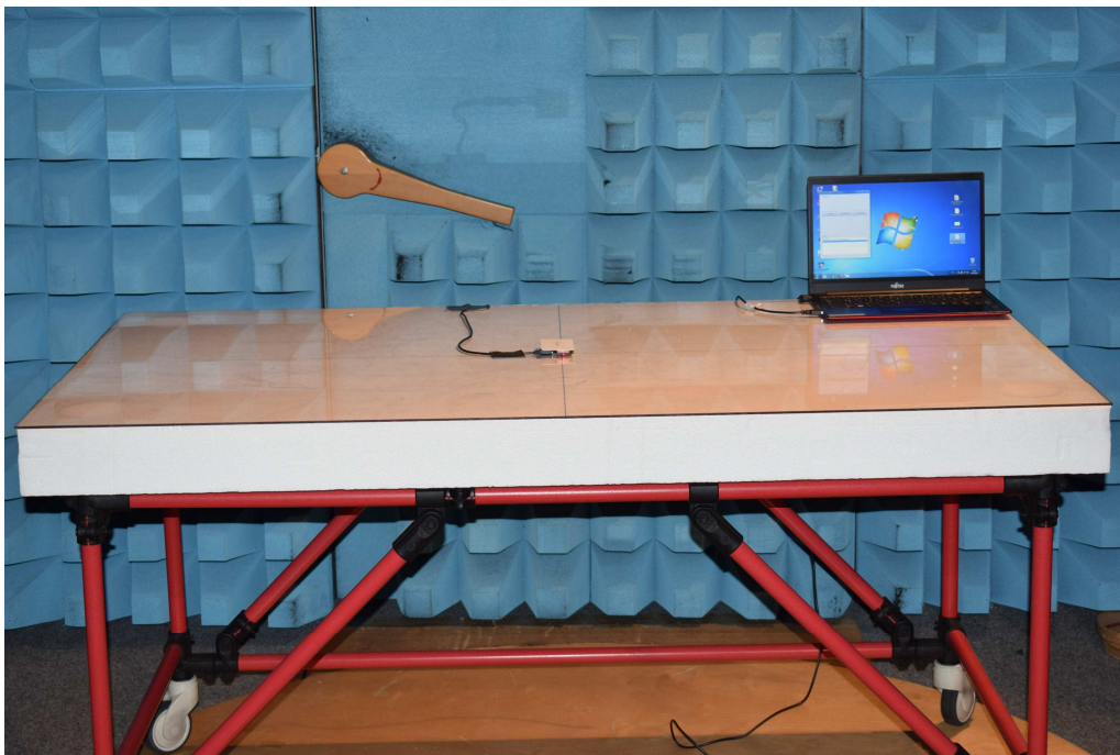
Picture 2: CDC, test setup radiated emission test 9 kHz -30 MHz (rear view)
