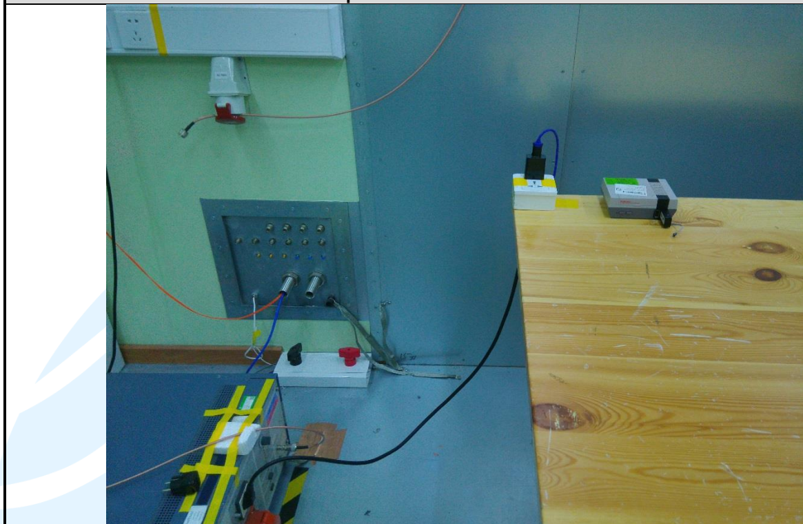
Set-up for AC Conducted Emissions
