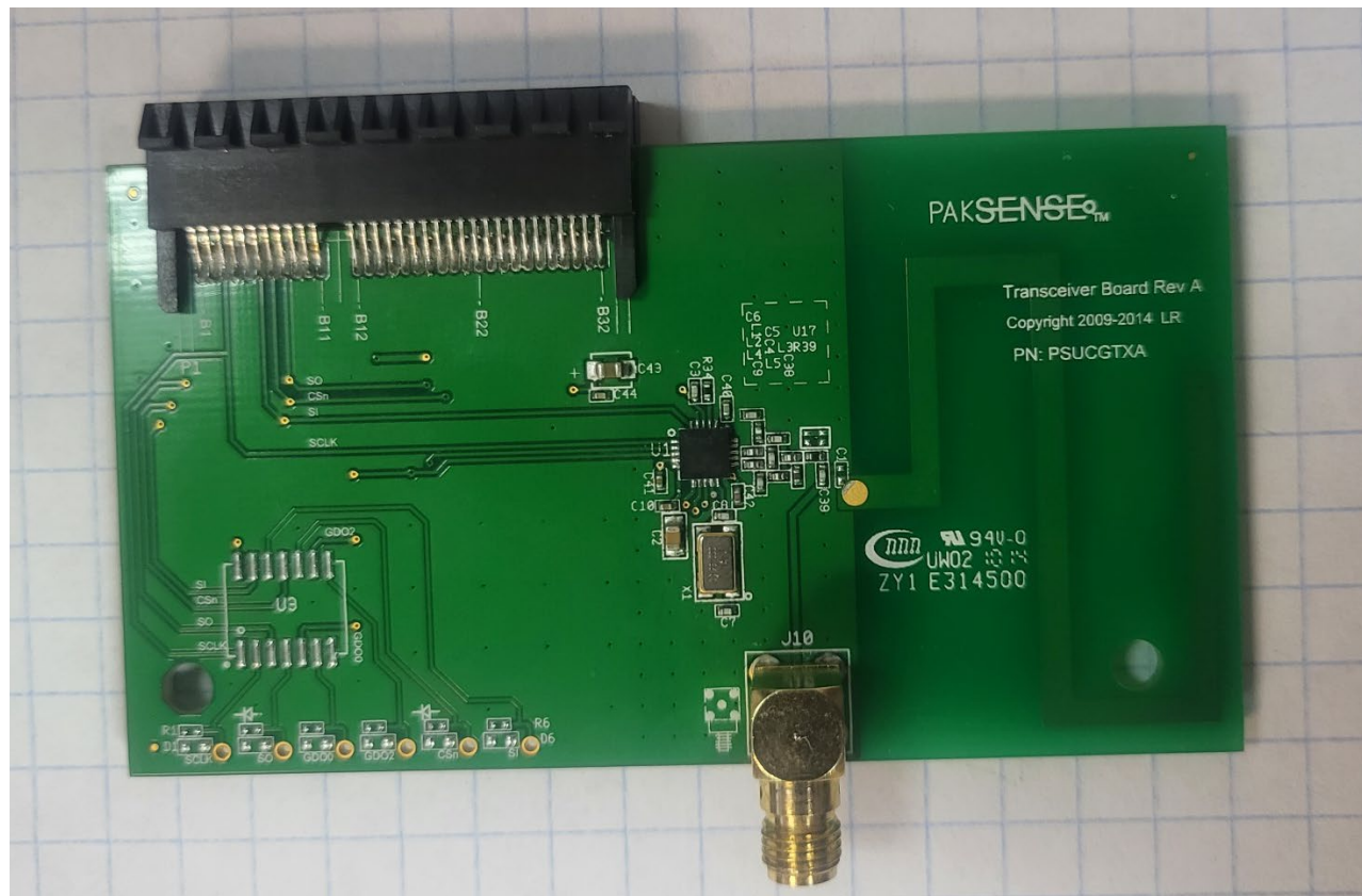
Figure 4. PSASII-04 Radio module (Component Side)
