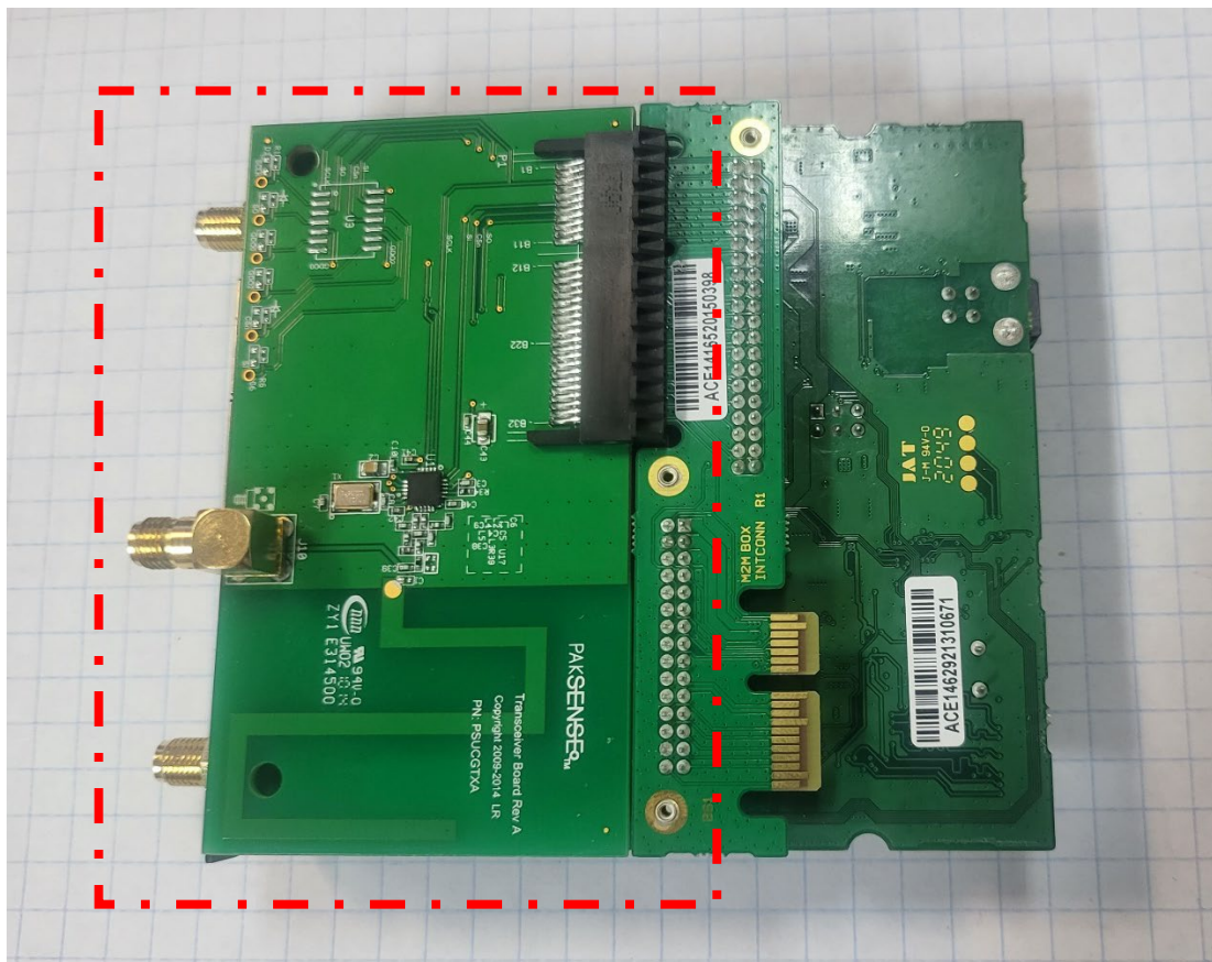
Figure 2. PSASII-04 Radio module installed on HOST Device interface board
