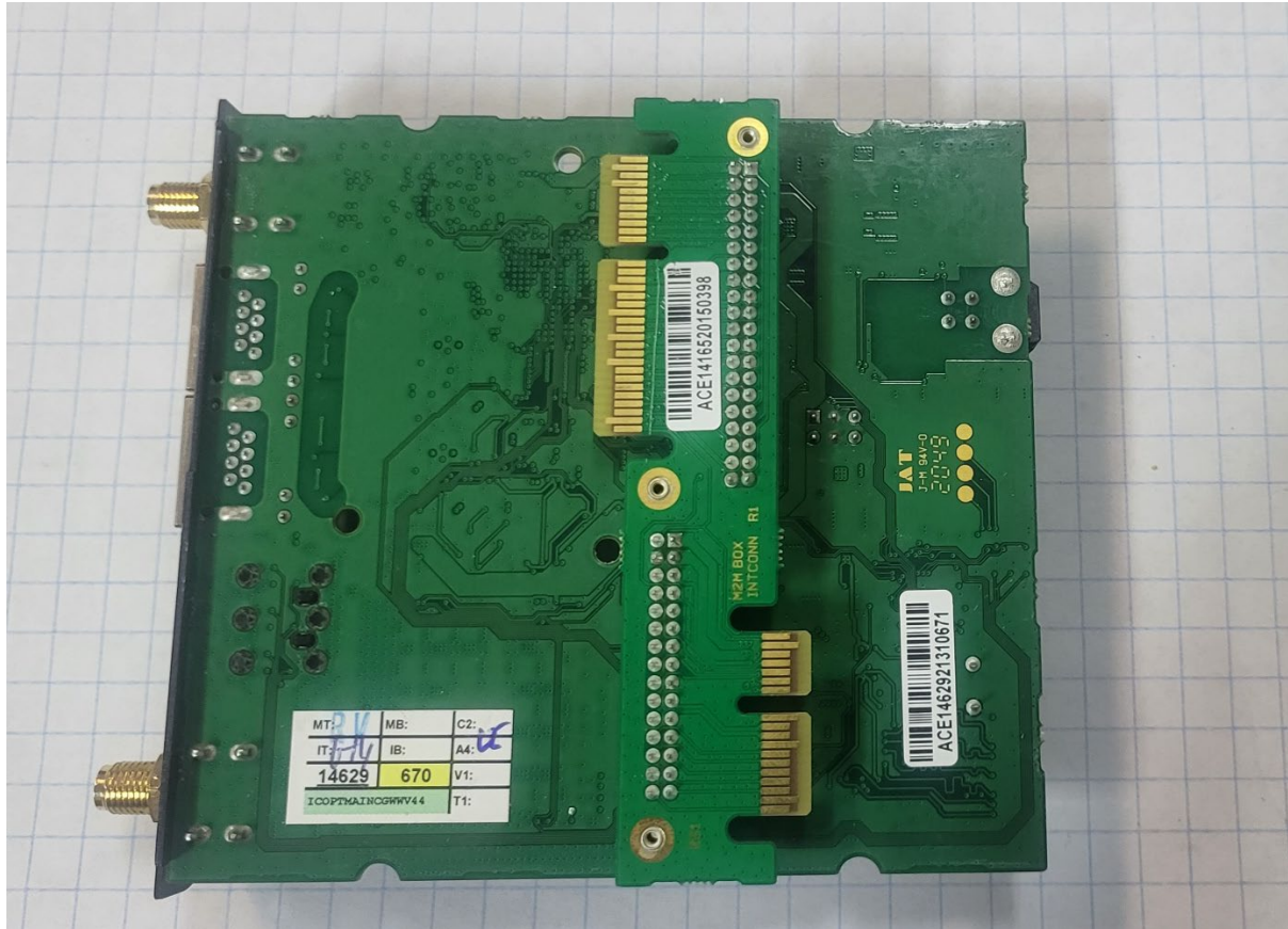
Figure 3. HOST Device interface board with radio module removed.
