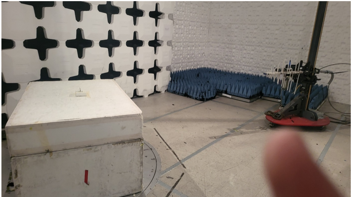
Figure 4. Test Configuration 200- 1000 MHz using Log Periodic Antenna
