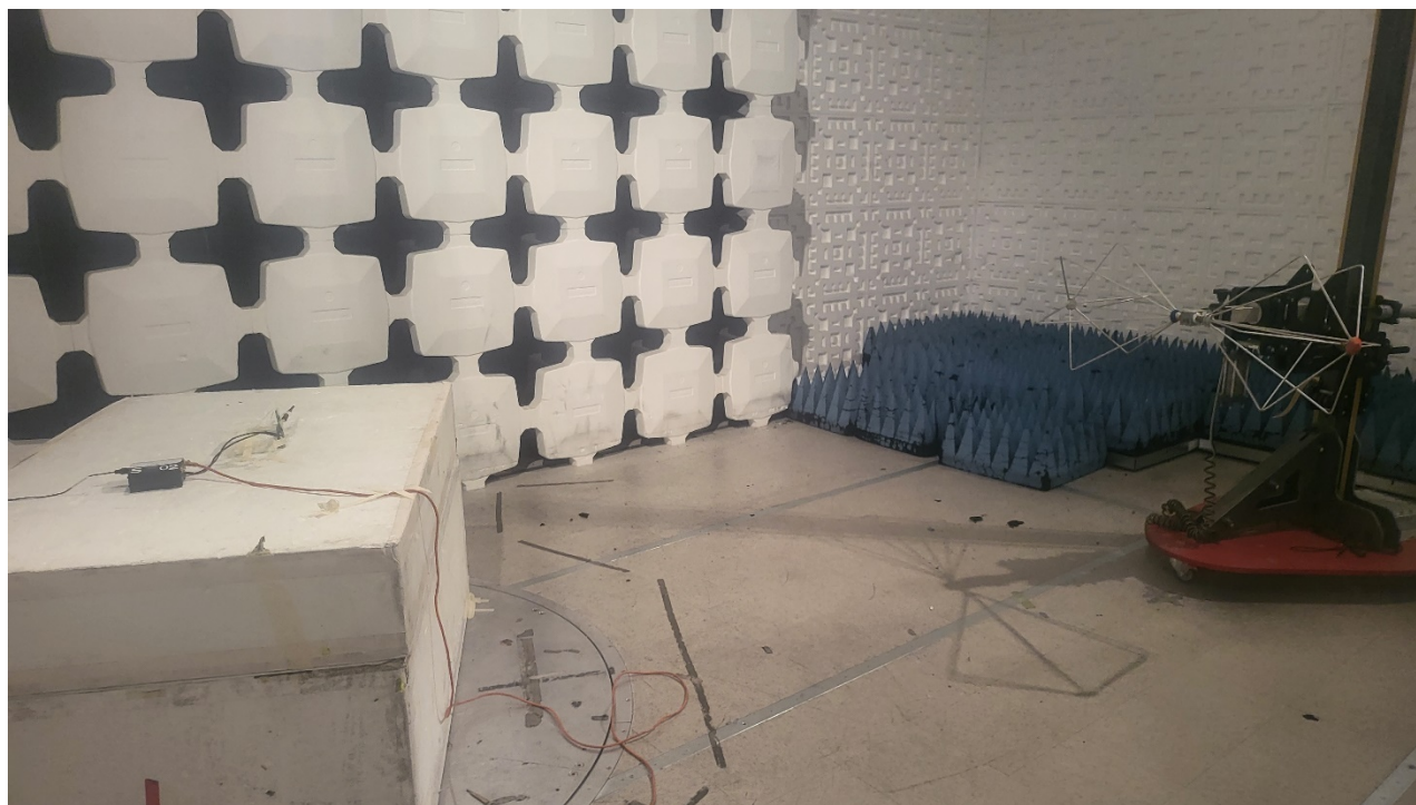
Figure 3. Test Configuration 30-200 MHz using Biconical Antenna
