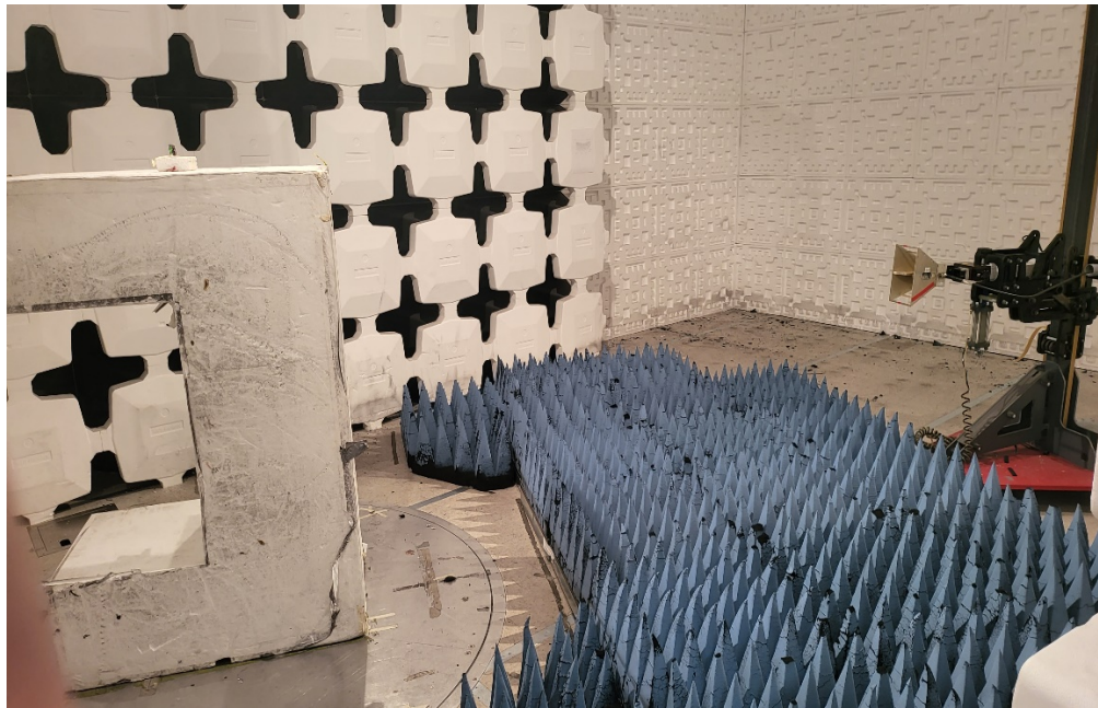
Figure 5. Test Configuration intentional Emissions above 1 GHz
