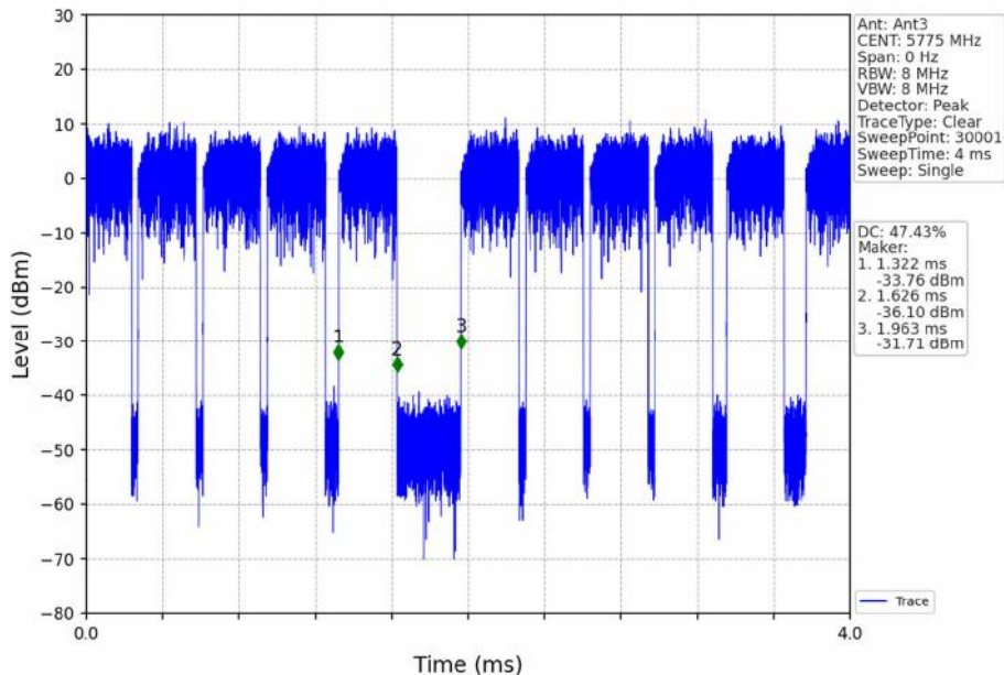
802.11ac(VHT80)_MCH_5775MHz_Ant3_NTNV
