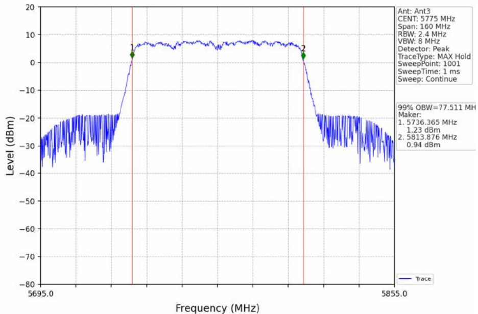
802.11ac(VHT80)_MCH_5775MHz_Ant3_NTNV
