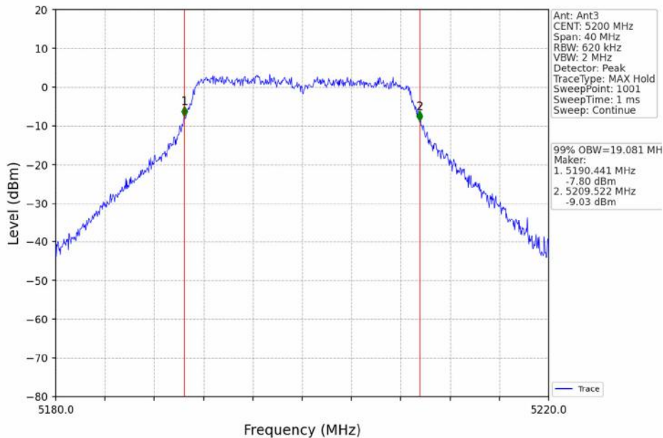
802.11n(HT20)_MCH_5200MHz_Ant3_NTNV
