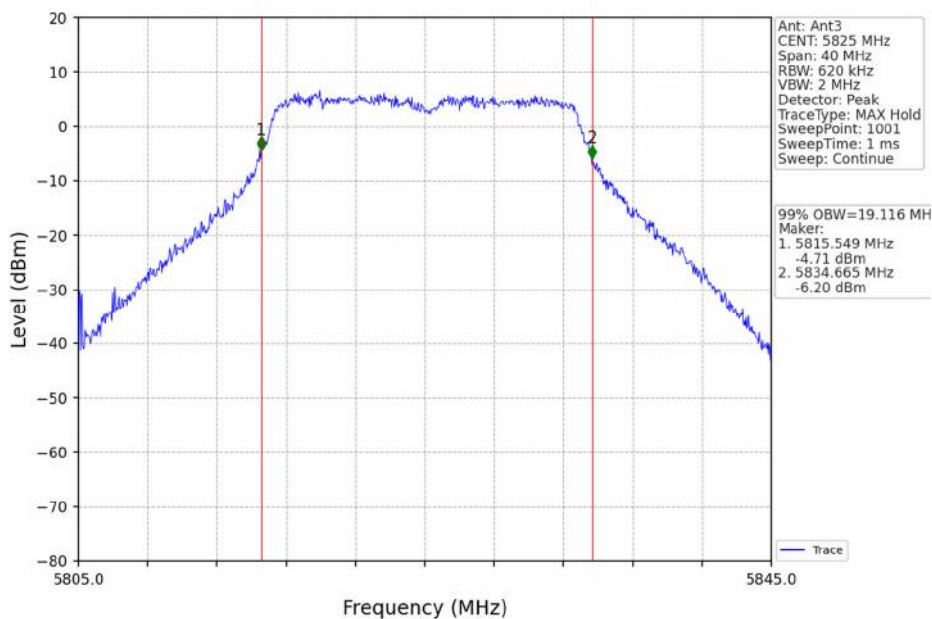
802.11ac(VHT20)_HCH_5825MHz_Ant3_NTNV
