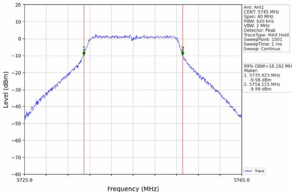
802.11a_LCH_5745MHz_Ant1_NTNV
