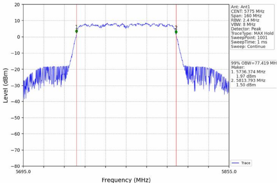
802.11ac(VHT80)_MCH_5775MHz_Ant1_NTNV
