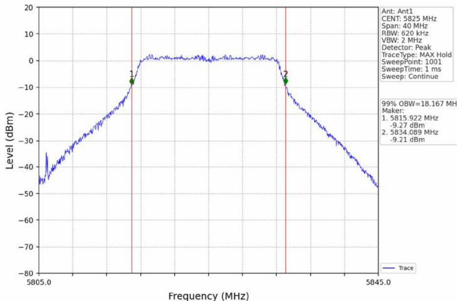
802.11a_HCH_5825MHz_Ant1_NTNV
