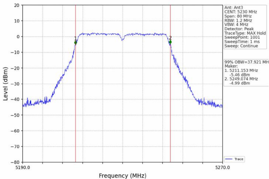
802.11ac(VHT40)_HCH_5230MHz_Ant3_NTNV
