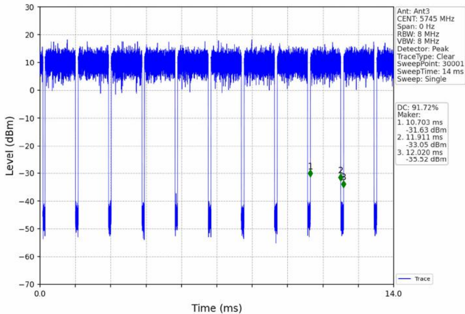
802.11n(HT20)_LCH_5745MHz_Ant3_NTNV
