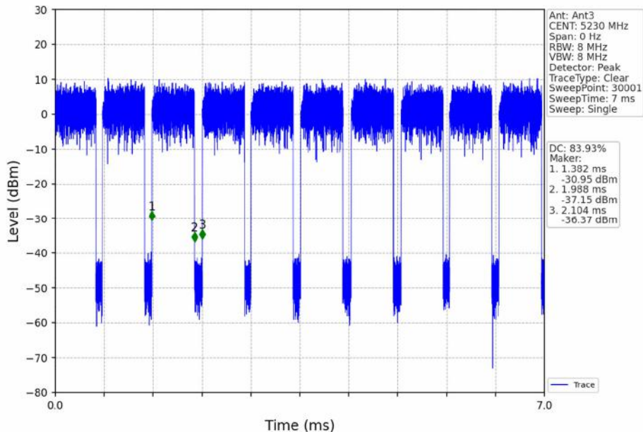
802.11ac(VHT40)_HCH_5230MHz_Ant3_NTNV
