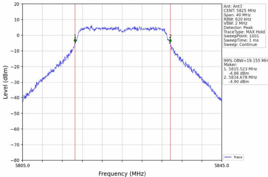
802.11n(HT20)_HCH_5825MHz_Ant3_NTNV
