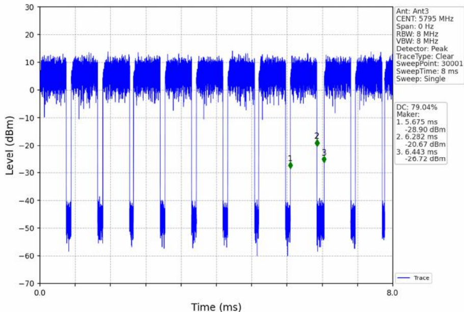
802.11ac(VHT40)_HCH_5795MHz_Ant3_NTNV
