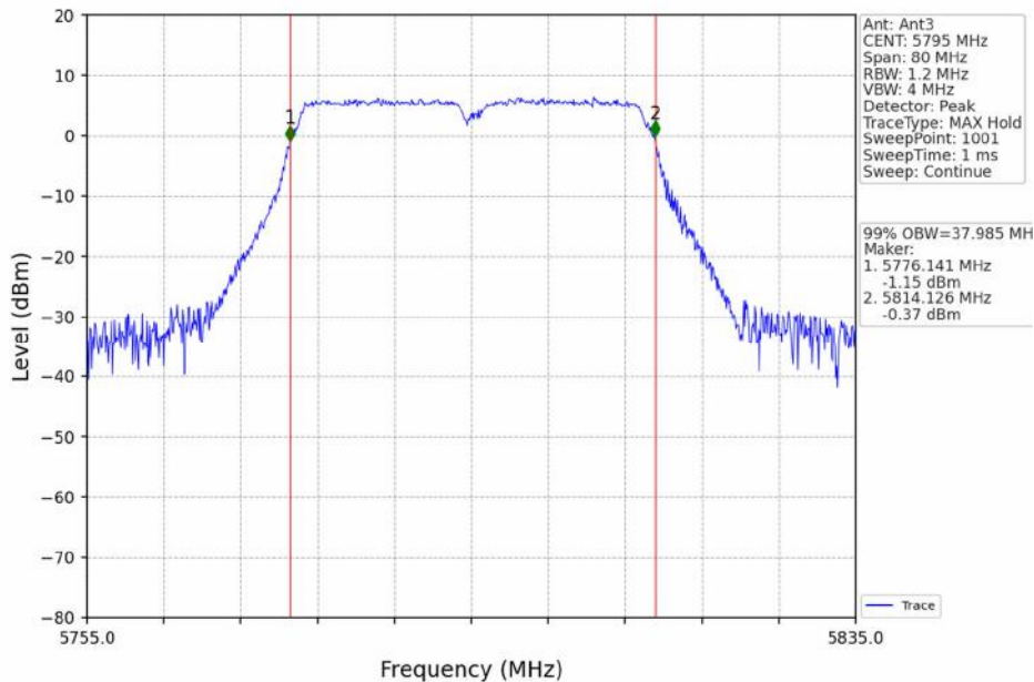
802.11n(HT40)_HCH_5795MHz_Ant3_NTNV
