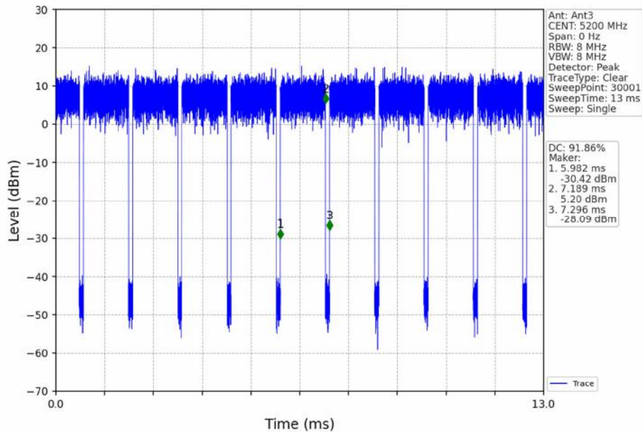
802.11n(HT20)_MCH_5200MHz_Ant3_NTNV
