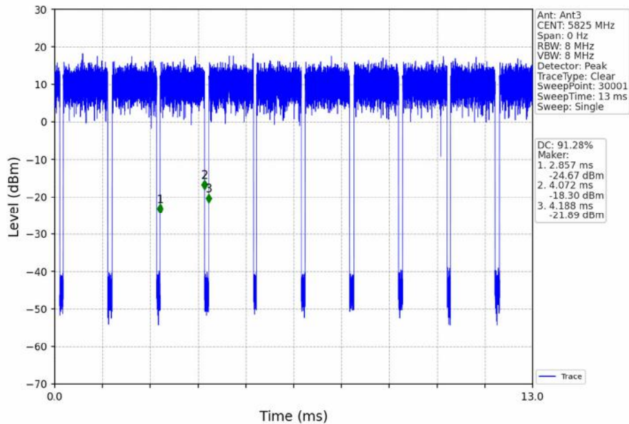
802.11ac(VHT20)_HCH_5825MHz_Ant3_NTNV
