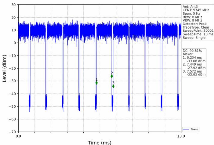
802.11ac(VHT20)_LCH_5745MHz_Ant3_NTNV
