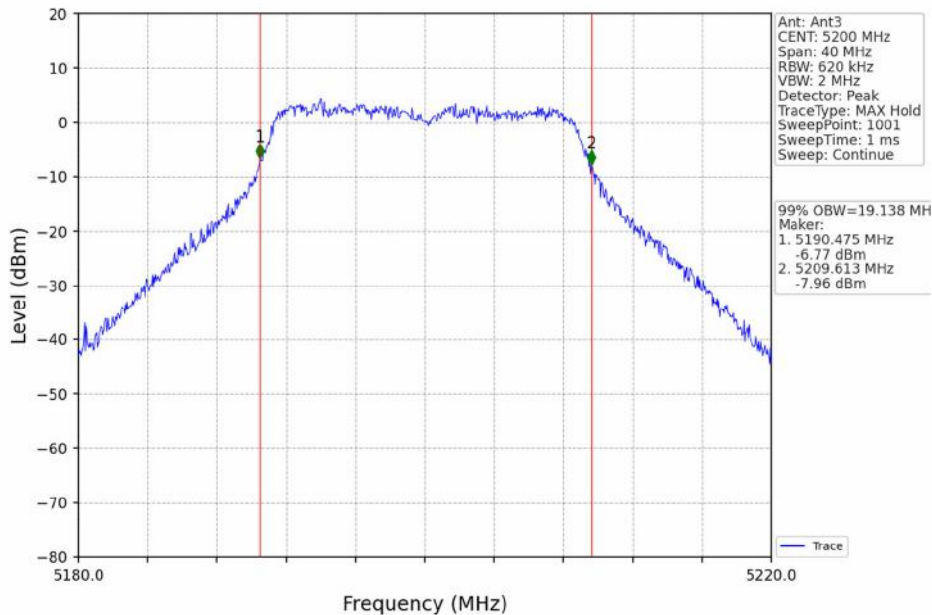
802.11ac(VHT20)_MCH_5200MHz_Ant3_NTNV
