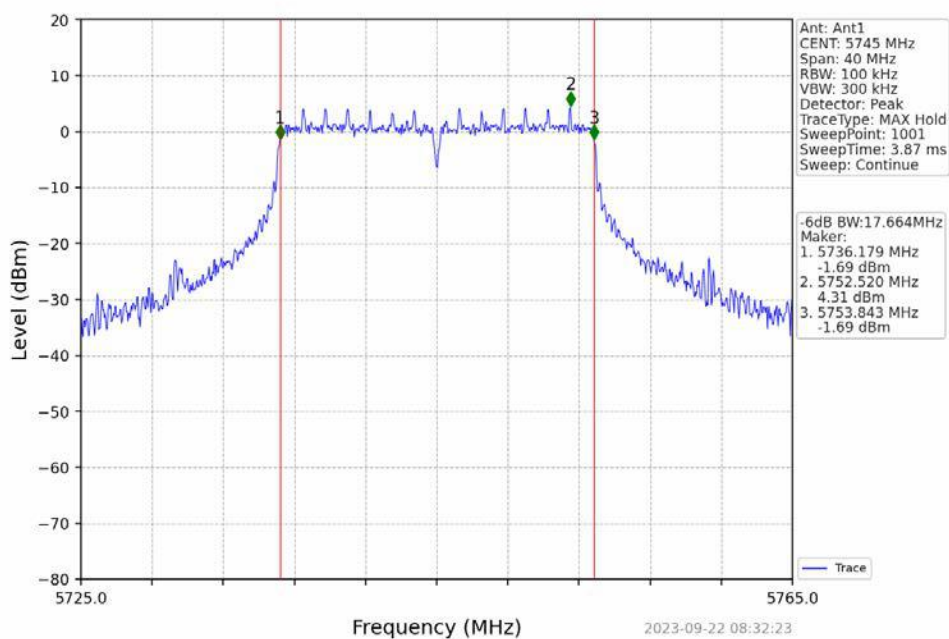
802.11n(HT20)_LCH_5745MHz_NTNV
