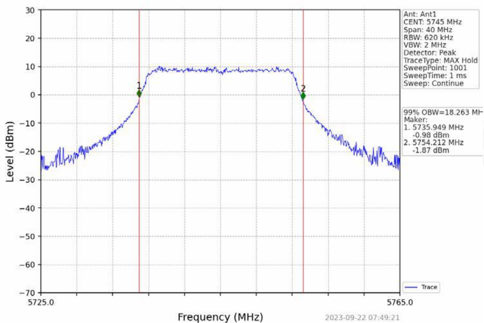
802.11a_LCH_5745MHz_NTNV
