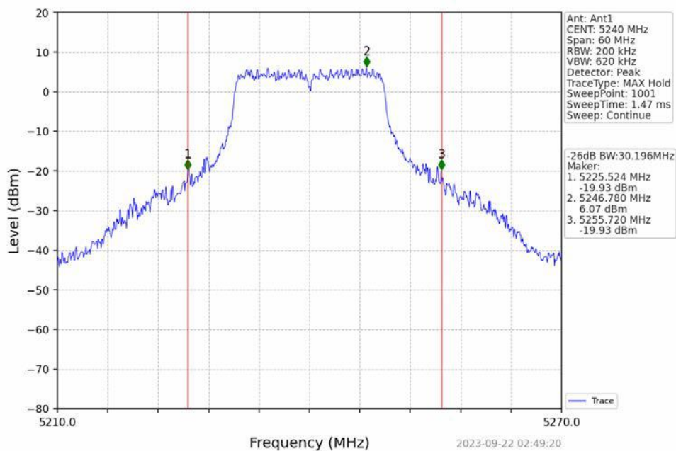
802.11n(HT20)_HCH_5240MHz_NTNV
