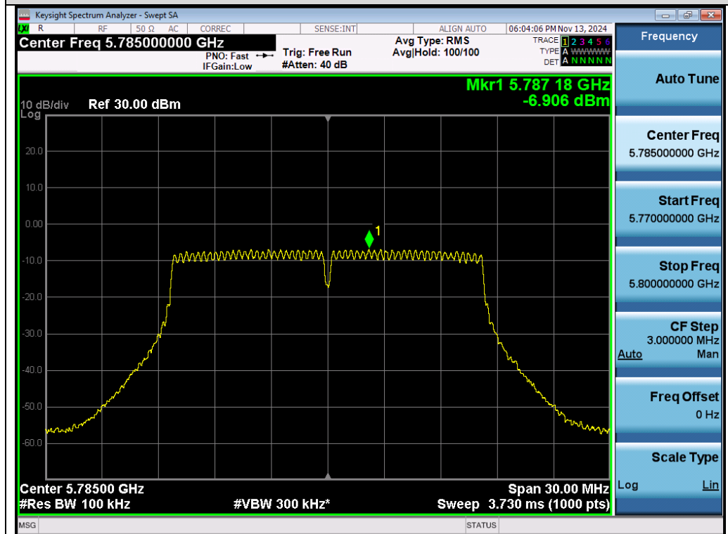
Test_Graph_802.11a_Chain B_5785_6Mbps_PSD
