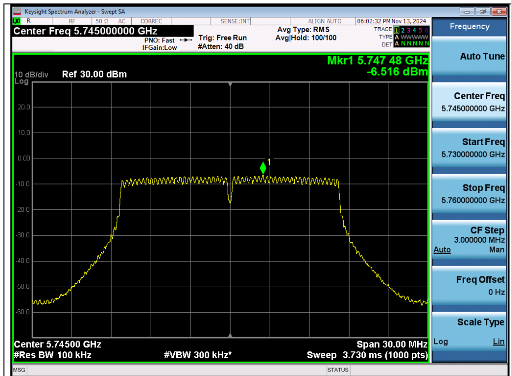
Test_Graph_802.11a_Chain B_5745_6Mbps_PSD
