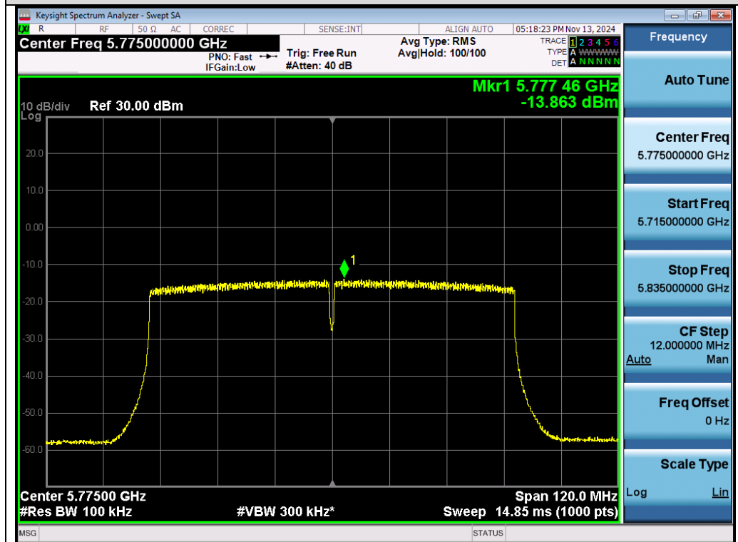
Test_Graph_802.11ac80_Chain A_5775_MCS0_PSD
