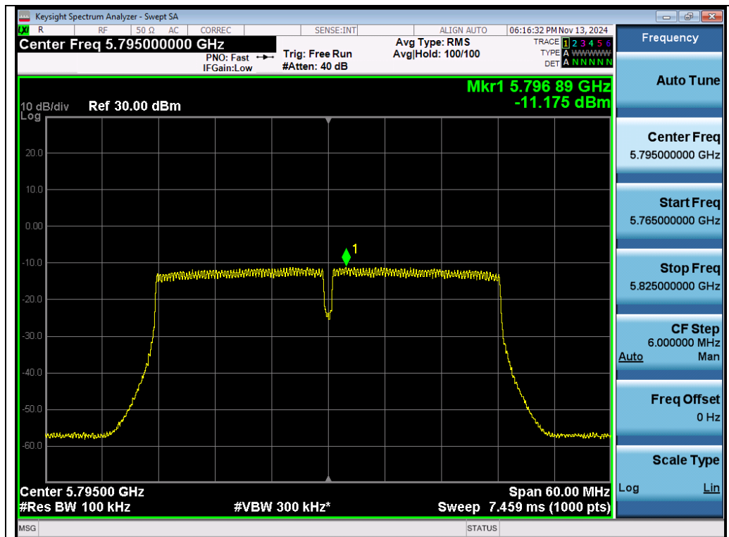
Test_Graph_802.11ac40_Chain B_5795_MCS0_PSD
