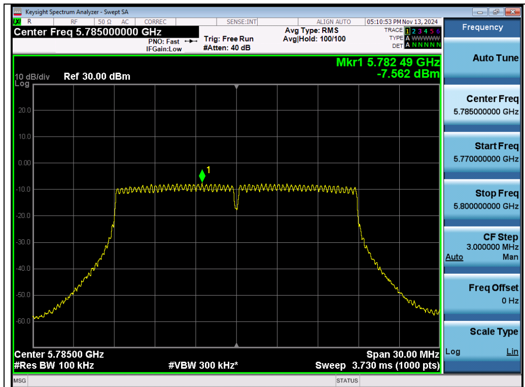
Test_Graph_802.11n20_Chain A_5785_MCS0_PSD
