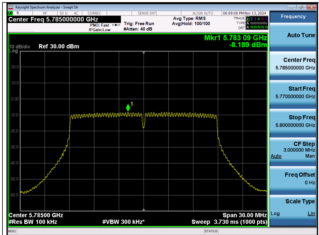
Test_Graph_802.11n20_Chain B_5785_MCS0_PSD
