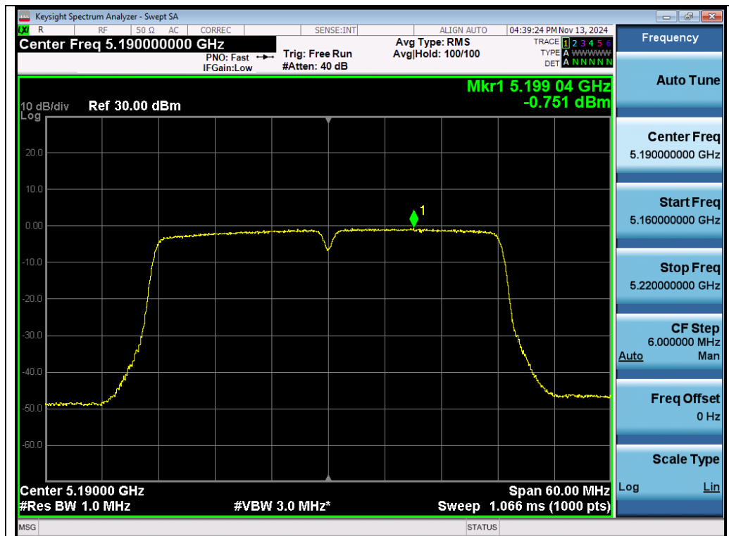
Test_Graph_802.11n40_Chain A_5190_MCS0_PSD
