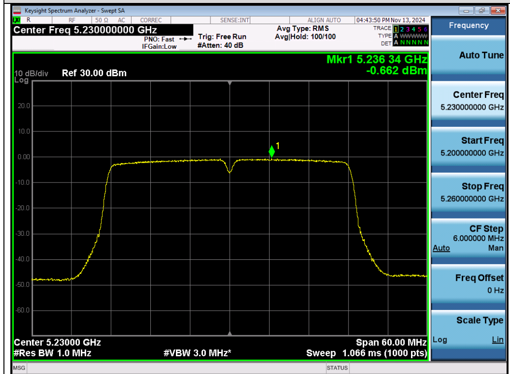
Test_Graph_802.11n40_Chain A_5230_MCS0_PSD
