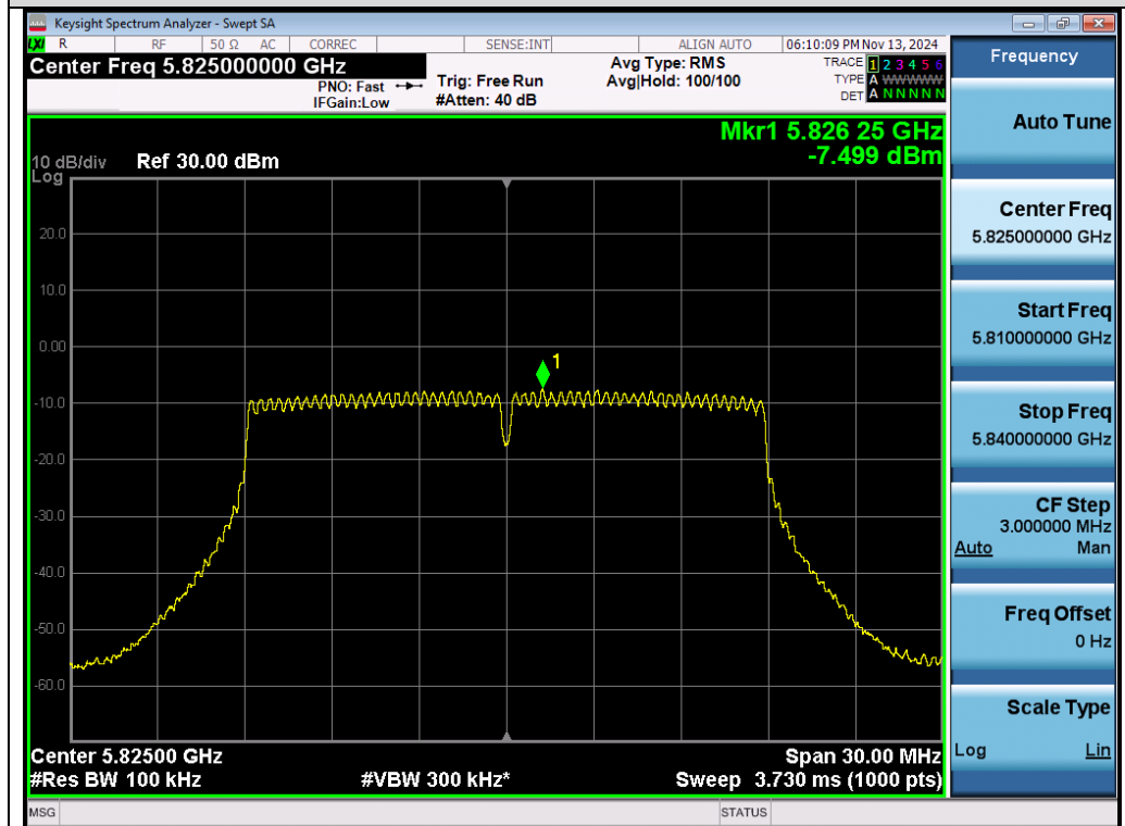
Test_Graph_802.11n20_Chain B_5825_MCS0_PSD
