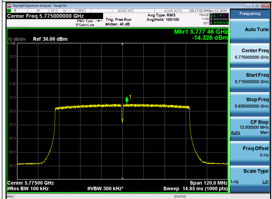
Test_Graph_802.11ac80_Chain B_5775_MCS0_PSD
