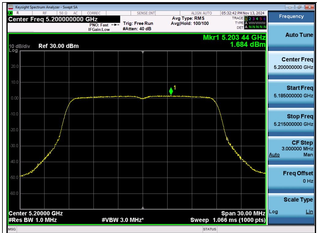
Test_Graph_802.11n20_Chain B_5200_MCS0_PSD
