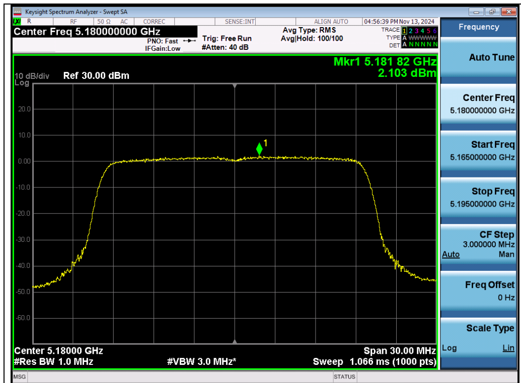
Test_Graph_802.11ax20_Chain A_5180_MCS0_PSD
