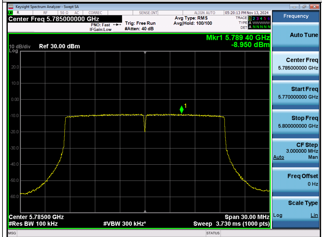
Test_Graph_802.11ax20_Chain A_5785_MCS0_PSD
