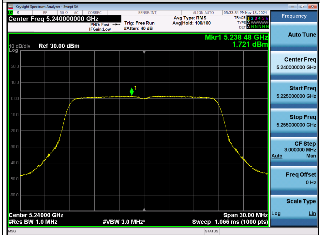
Test_Graph_802.11n20_Chain B_5240_MCS0_PSD
