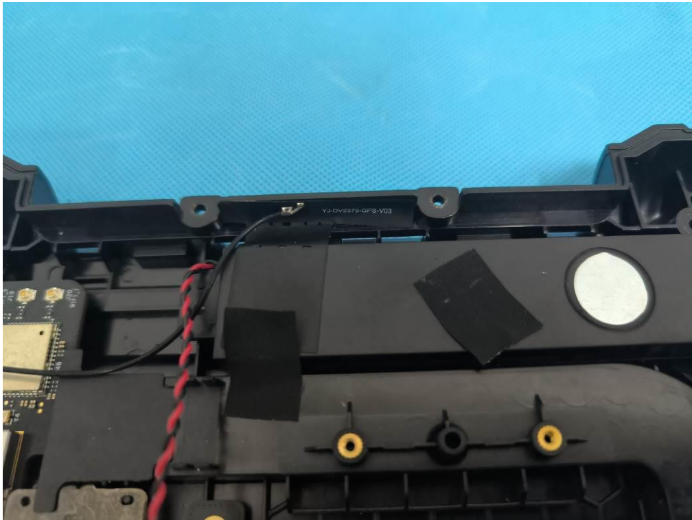
OPEN VIEW OF EUT (FIGURE 12)
